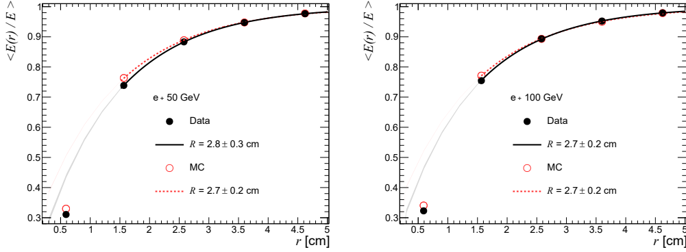
Figure 16: Statistical mean of \langle E(r)/E \rangle as a function of r for nominal positron energy of 50 GeV and 100 GeV in data and simulation. The radial containment R is extracted from the fitted exponential function defined in Eq. 7.4 using \langle E(r)/E \rangle = 0.9 (the error on R is evaluated by propagating the parameter fit uncertainties and by considering different choices of discrete r ).
