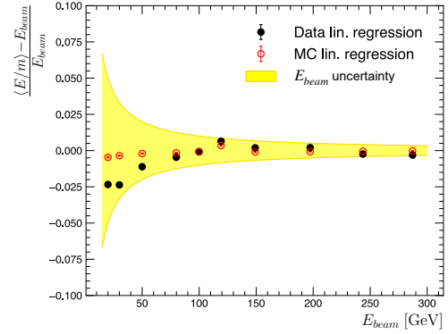
Figure 6b: Linearity with the energy. The measured energies are divided by the slope obtained from a linear fit to as a function of , with the slope and intercept allowed to float. The yellow band represents the relative error on the beam energy from the uncertainty of the dipole currents corresponding to an uncertainty of 1 GeV in momentum.
