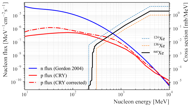
Figure 2: The calculated spallation cross section of ^{37}\text{Ar} from individual xenon isotopes (light dotted curves) and natural xenon (solid black). Overlaid is the surface nucleon flux used in our calculations [33, 34]. According to the model of Silberberg and Tsao [25], the spallation cross section is negligible below about 210 MeV and increases with energy until 4 GeV, beyond which it is assumed to be constant.
