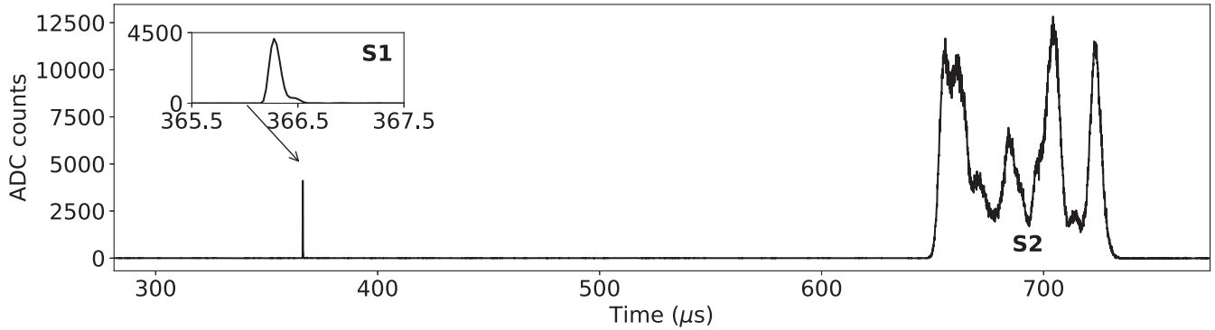
FIG. 4. Typical waveform, summed over all PMTs, for an event from ^{208}\text{Tl} gamma (2.6 MeV) photoelectric absorption. Signals S1 and S2 are highlighted (adapted from [67]).
