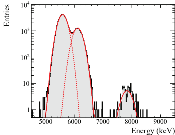
FIG. 5. Secondary scintillation (S2) spectra registered in the NEXT-White detector for ^{83\text{m}}\text{Kr} decays at 41.5 keV (top panel) and ^{222}\text{Rn} (5.590 MeV), ^{218}\text{Po} (6.112 MeV) and ^{214}\text{Po} (7.834 MeV) alphas (bottom panel), obtained at 1.7 \text{ kV cm}^{-1} \text{ bar}^{-1} and 0.62 \text{ kV cm}^{-1} \text{ bar}^{-1} in the EL region, respectively.
