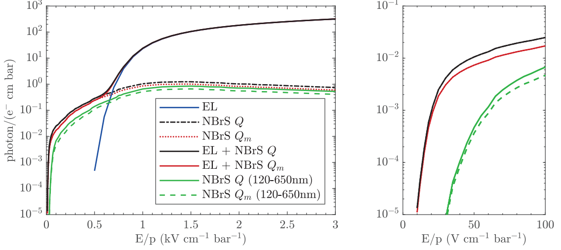
FIG. 16. Simulated secondary scintillation yield in the range of 120-1000 nm as a function of E/p . A dependence with either Q or Q_m has been assumed in Eq. 7. The individual contributions from EL and NBrS are shown ( T = 300 K). A detail of the 0-100 \text{V cm}^{-1} \text{bar}^{-1} region is shown on the right side. For comparison, the simulated NBrS yield in the 120-650 nm range is also plotted.
