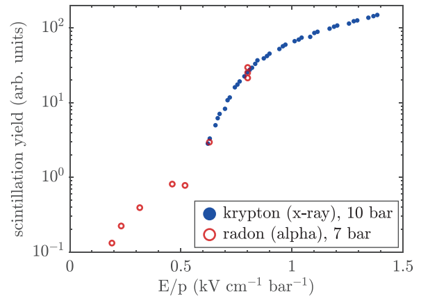
FIG. 6. Secondary scintillation (S2) measured for x-rays (closed circles) and \alpha -particles (open circles) with the NEW-TPC. No corrections for the wavelength-shifting effect of the TPB, light collection or quantum efficiency have been applied.
