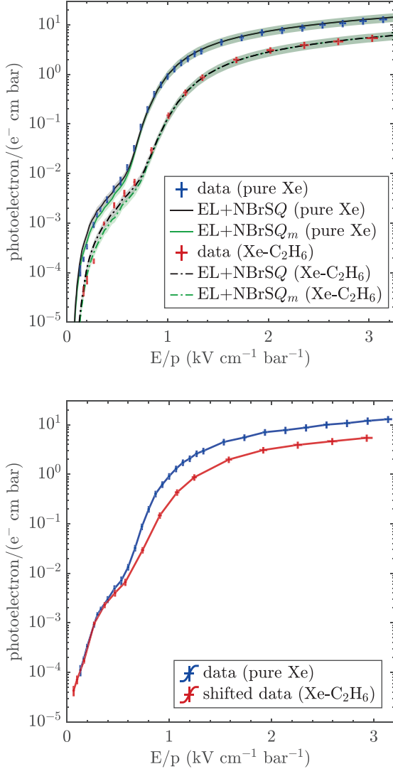
FIG. 14. Top: the number of photoelectrons (68 % confidence level depicted as error bars) obtained experimentally with pure Xe and a Xe-C 2 H 6 admixture (with a 0.12 % C 2 H 6 molar concentration), together with the respective simulated curves (systematic error depicted as coloured bands). The experimental results provided by the two analysis methods for low electric fields have been statistically combined. Bottom: the Xe-C 2 H 6 curve was shifted to the left by 100 V cm -1 bar -1 , illustrating the different nature of the low- E/p emission since it is not quenched, unlike the EL (excimer-based) contribution.
