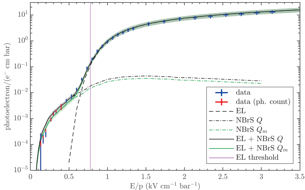
FIG. 11. Number of detected photoelectrons obtained with the driftless GPSC as a function of reduced electric field, being the value normalised according to the gas pressure, drift path and number of primary ionization electrons. At low electric fields, the experimental results obtained with the photon counting method are also shown (points in red). Error bars present the 68 % confidence levels of the experimental data. As defined at the end of section III.B, the EL threshold was obtained from a linear fit to the EL yield data for E/p values above 1 \text{ kV cm}^{-1} \text{ bar}^{-1} , where the yield dependence on E/p is approximately linear. Simulated curves are superimposed to the data, being the NBrS yield obtained assuming proportionality with either Q or Q_m . Coloured bands present the systematic error associated to the simulation curves, dominated by the 20% uncertainty estimated for the detection efficiency.
