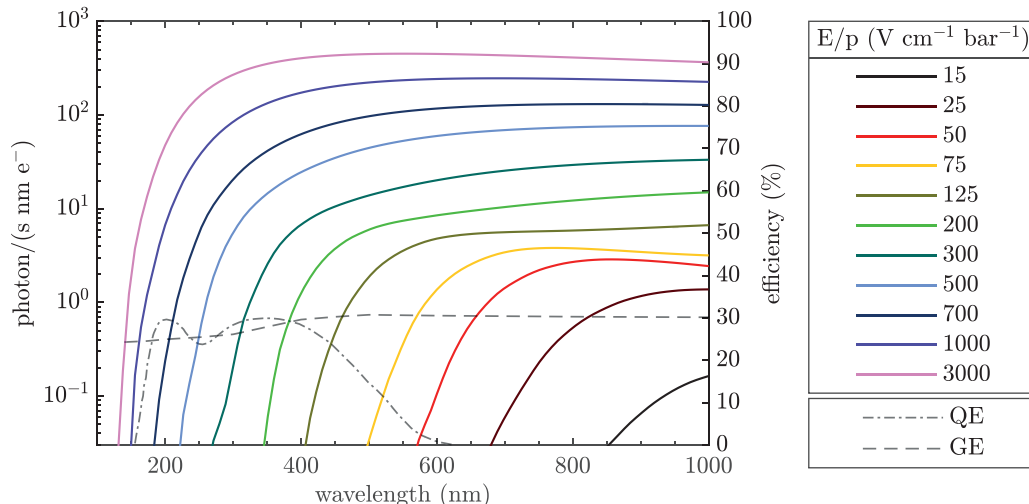
FIG. 2. Computed NBrS emission rate as a function of wavelength for different electric field values, using Eq. 7 with Q_m . The quantum efficiency of the PMT used for the main part of the measurements presented in this work is indicated by the dot-dashed line. The geometrical efficiency of the experimental setup, calculated with GEANT4 (see a description later in the text), is indicated by the dashed line.
