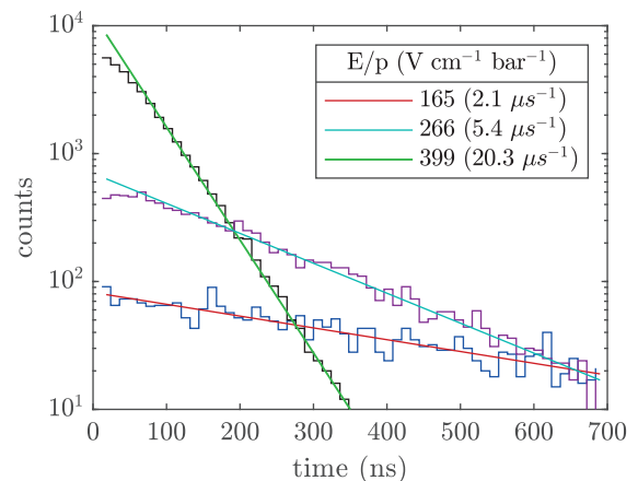
FIG. 12. Distribution of time elapsed between photoelectron events in the NBrS region obtained from 1500 waveforms for three different electric field values. An exponential function is fitted to each dataset; the photoelectron rates obtained from the fits are shown in the legend.
