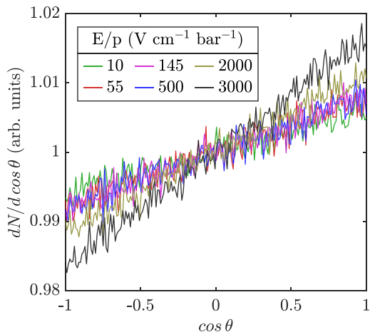
FIG. 1. Angular distributions ( dP/d\cos\theta ) obtained for the angle between the electron momentum vector and the direction of the electric field, prior to each collision, obtained with the transport code PYBOLTZ.
