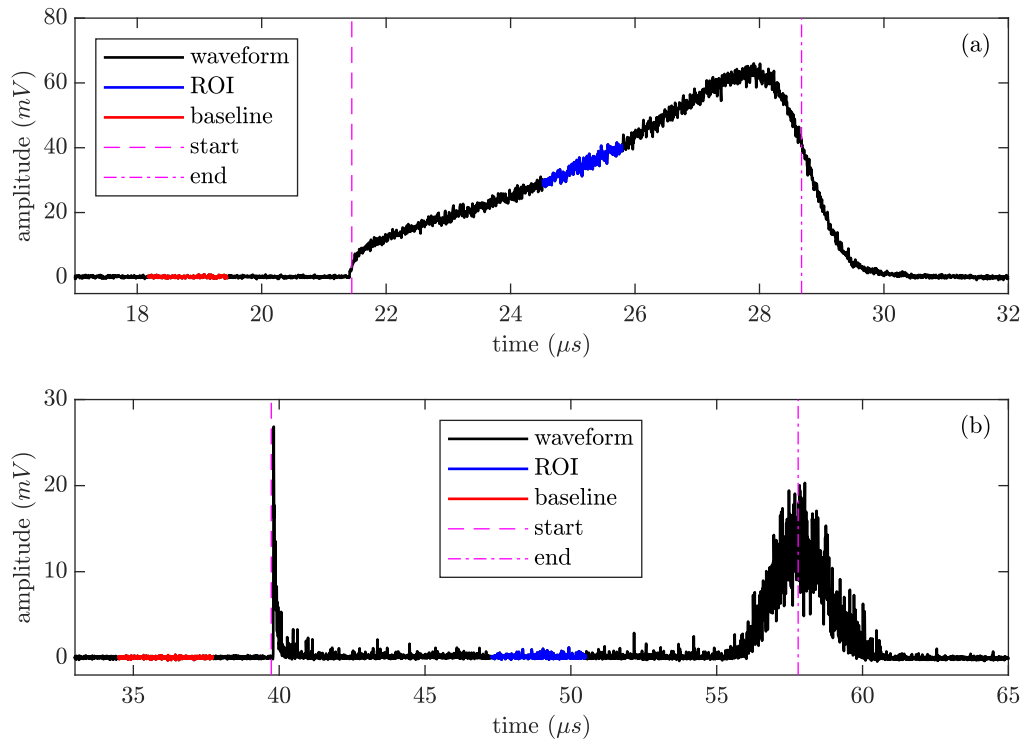
FIG. 8. Typical driftless GPSC waveforms obtained for an E/p value of 1.5 \text{ kV cm}^{-1} \text{ bar}^{-1} , higher than the EL threshold (a) and for an E/p of 320 \text{ V cm}^{-1} \text{ bar}^{-1} , lower than the EL threshold (b). The start- and end-of-event are represented by vertical lines. The regions chosen to determine the NBrS and EL (ROI) are indicated in blue.
