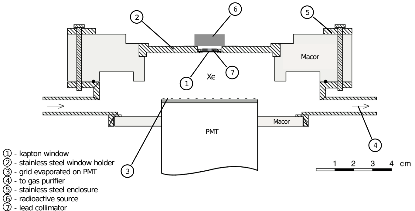
FIG. 7. Schematic of the driftless GPSC used in this work, adapted from [33].
