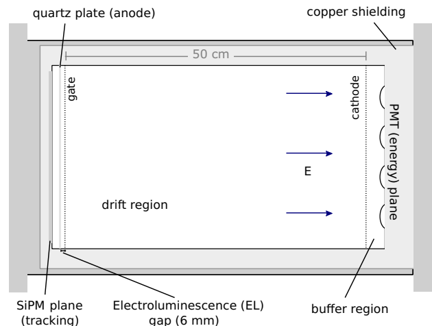
FIG. 3. Schematic of the EL-based TPC developed by the NEXT collaboration for double-beta decay searches in ^{136}\text{Xe} , adapted from [67].
