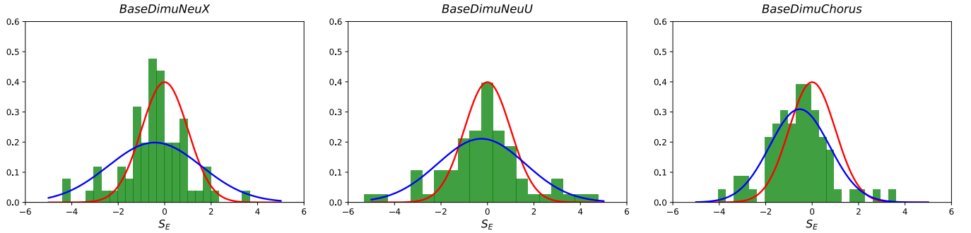
FIG. 16. Distribution of the variable S_E for all experiments in the BaseDimuNeuX analysis (left) and for all experiments in the BaseDimuNeuU analysis (middle). The right panel shows the distribution of the variable S_E from the BaseDimuChorus analysis. All panels show the fitted Gaussian distribution to the actual S_E distribution (blue) compared to the ideal Gaussian S_E distribution with \mu = 0 and \sigma = 1 (red). Note that in the case of the BaseDimuNeuX analysis we do not show a bin with S_E=9.72 which corresponds to the NuTeV neutrino data.
