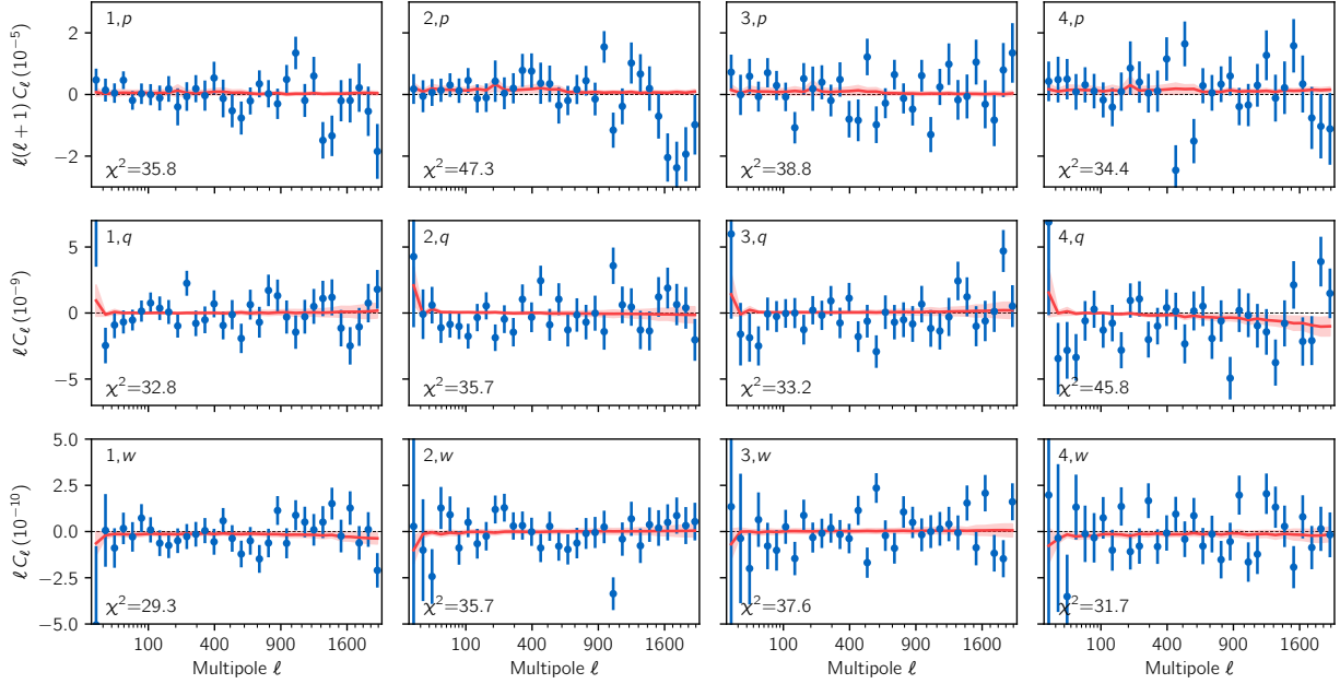
Figure A1. Cross-power spectra between galaxy shapes in the four redshift bins (from left to right) with PSF parameters \mathbf{p} , \mathbf{q} and \mathbf{w} (from top to bottom). The measurements are shown in blue, with error bars computed from 18 000 Gaussian simulations using the DES Y3 catalog ellipticities and positions, as explained in section 4.1.1. The model from eqs. (A3) to (A5) at best-fit is shown by the red line, while the band shows the uncertainty. We find \chi^2 statistics with respect to the best fit between 29.3 and 45.8 (29.3 to 47.3 for the null hypothesis) for 32 degrees of freedom, shown in the lower left corner for each panel, corresponding to a minimum probability-to-exceed of 0.04.
