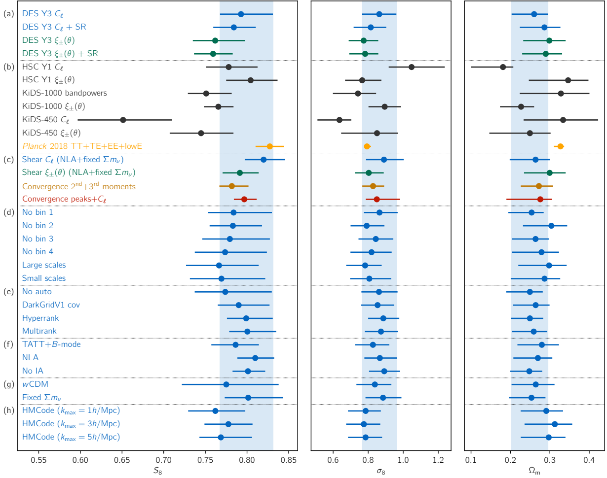
Figure 11. Comparison of one-dimensional marginal posterior distributions over the parameters S_8 \equiv \sigma_8 (\Omega_m/0.3)^{0.5} , \sigma_8 and \Omega_m , from DES Y3 data as well as other experiments, and consistency tests for this work (in blue). (a) Constraints obtained from the harmonic (this work) and real (Amon et al. 2022; Secco, Samuroff et al. 2022) space analyses of DES Y3 data are shown in blue and green (see also fig. 14), both with and without shear ratio information (SR, Sánchez, Prat et al. 2021). (b) Constraints from other weak lensing surveys, namely HSC Y1 (Hikage et al. 2019; Hamana et al. 2020), KiDS-1000 (Asgari et al. 2021) and KiDS-450 (Hildebrandt et al. 2017; Köhlinger et al. 2017) are shown in gray, and constraints from cosmic microwave background observations from Planck 2018 are shown in yellow (Planck Collaboration et al. 2020). (c) Constraints from four weak lensing analyses of DES Y3 data are compared, including the analysis of mass map moments (Gatti et al. 2021b) and peaks (Zürcher et al. 2022), and illustrating a high level of consistency (see also fig. 15). (d) Consistency tests where redshift bins are removed one at a time (first four) and where the data vector is split into its large- and small-scale data points (last two) (see also appendix C). (e) Various other consistency tests: removing auto power spectra, swapping the covariance matrix, and marginalizing over redshift distribution uncertainties with HYPERRANK and MULTIRANK (see also appendix C). (f) Modeling robustness test for intrinsic alignment (IA), including B-mode power spectra, or replacing TATT by NLA, or removing IA contributions altogether (see also section 6.2 fig. 12). (g) Other robustness test, freeing the dark energy equation-of-state w or fixing the neutrino mass to 0.06 eV. (h) Baryonic feedback tests where the matter power spectrum is computed with HMCODE instead of HALOFIT, and fiducial scale cuts are replaced with k_{\max} = 1, 3 and 5 h \text{ Mpc}^{-1} scale cuts (see also section 6.3 and fig. 13).
