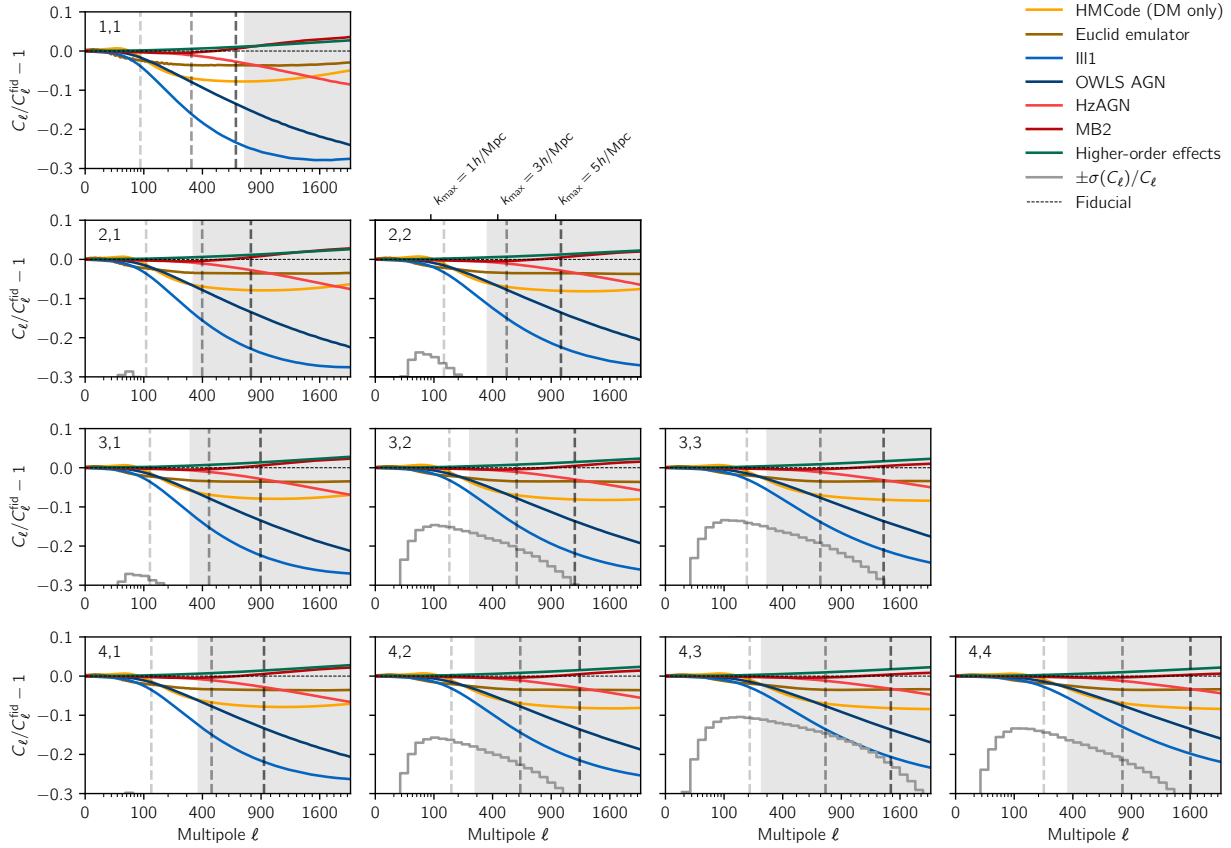
Figure 5. Residual shear power spectra with respect to the fiducial power spectra, C_\ell^{\text{fid}} . The orange (HMCode) and brown (Euclid emulator) curves show residuals for alternative prescription of the non-linear power spectrum (see section 3.2.2). The blue and red curves show the effect of baryons as predicted by four hydrodynamical simulations (Illustris, OWLS AGN, Horizon AGN and MassiveBlack II). Higher-order lensing effects computed with CosmoLike are also shown, in green, to be small. The error bars are shown by the gray step-wise lines which represent \pm\sigma(C_\ell)/C_\ell on the same scale (only -\sigma(C_\ell)/C_\ell is visible). The gray shaded regions show scales that are not used in the fiducial analysis where the effect of baryons is neglected. The gray dashed lines show the scale cuts corresponding to k_{\text{max}} = 1, 3 and 5 h \text{ Mpc}^{-1} (see section 3.5.2).
