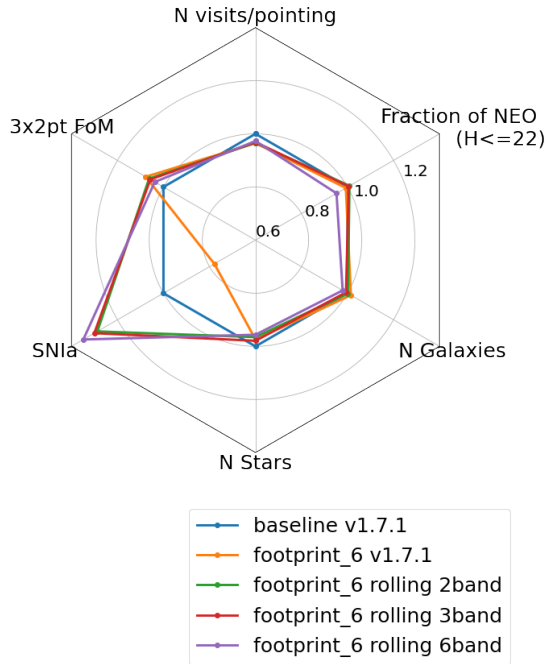
Figure 5. Illustration of a “radar plot” comparing science metrics from a variety of core science areas for five OpSim realizations (as indicated in the legend). Each corner of the hexagon represents a different metric, whose value is mapped to the distance from the center of the hexagon. Clockwise from the top, the metrics measure: the median number of visits per pointing in the WFD ( N visits/pointing ), the fraction of Near Earth Objects of magnitude H \leq 22 detected ( Fraction of NEO ), the numbers of galaxies ( N Galaxies ) and stars ( N stars ) expected to be recovered, the expected number of supernovae type Ia ( SN Ia ) observed sufficiently well to contribute to cosmological measurements (Lochner et al. 2018), and a collective metric for static probes of the extra-galactic sky ( 3x2pt FoM , combining Weak Lensing and Galaxy Clustering, Lochner et al. 2018). This set of OpSim runs varies the footprint (which impacts the science throughput for cosmological supernovae as measured by SN Ia ) and introduces a rolling cadence (which improves SN Ia performance as a denser cadence enables better characterizations at relevant, short time scales and the distribution of visits in a more concentrated sky area leads to small efficiency improvements). This figure is discussed in subsection 4.1.
