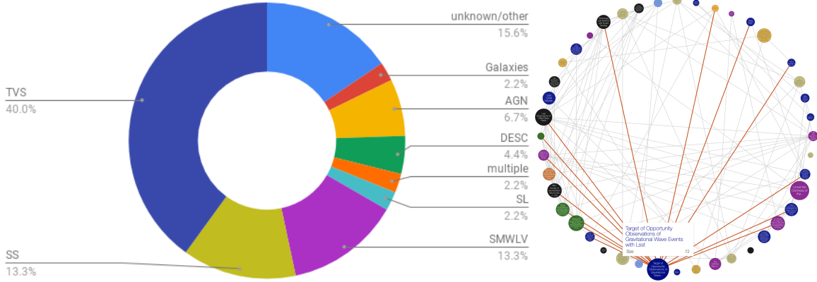
Figure 4. A synopsis of the 46 Cadence White Papers submitted in response to the call issued in 2018: on the left the papers are grouped by the Rubin LSST Science Collaboration (SC) of the lead author with fractions from each SC indicated in the figure. 15% of the papers were submitted by lead-authors unaffiliated with a SC. The right panel shows a screenshot of an interactive plot (available at http://fbb.space/LSSTWP/WPbyfirstAuthor.html ) describing the co-authors network through a chord diagram. Each circle represents a paper, the size of the circle reflecting the size of the authoring team (the largest is 72 co authors for Target of Opportunity Observations of Gravitational Wave Events with LSST), color-coded, as in the left panel, by the SC of the lead author. Papers are linked by their co-authors. This figure is discussed in Section 4 and Section 6.
