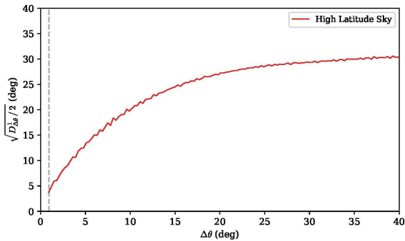
Figure 6. \sqrt{D}/2 vs separation \Delta\theta for the high-latitude C-BASS polarization angles, where D is the structure function, so \sqrt{D}/2 would equal the standard deviation, on scales large enough that pixel pairs are uncorrelated.
