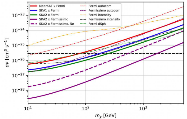
Figure 17. Limits on the cross-section as a function of the dark matter mass. Comparison with limits from: auto-correlation of gamma rays (dashed red for Fermi Ackermann et al. (2018) , light purple dashed for Fermissimo), intensity of the gamma-ray flux (yellow for Fermi Ackermann et al. (2015) , black for Fermissimo) and dwarf spheroidal galaxies ( Albert et al. 2017 ).
