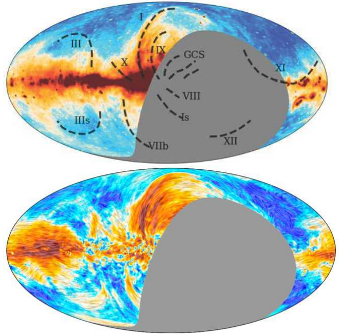
Figure 5. C-BASS North maps of total intensity ( top ) and polarised intensity ( bottom ) in Galactic coordinates using a mollweide projection. The total intensity map color scale has been saturated along the Galactic plane and includes the locations of well-known radio loops (Vidal et al. 2015). The polarised intensity map has the projected B-field direction overlaid using line-integral convolution.
