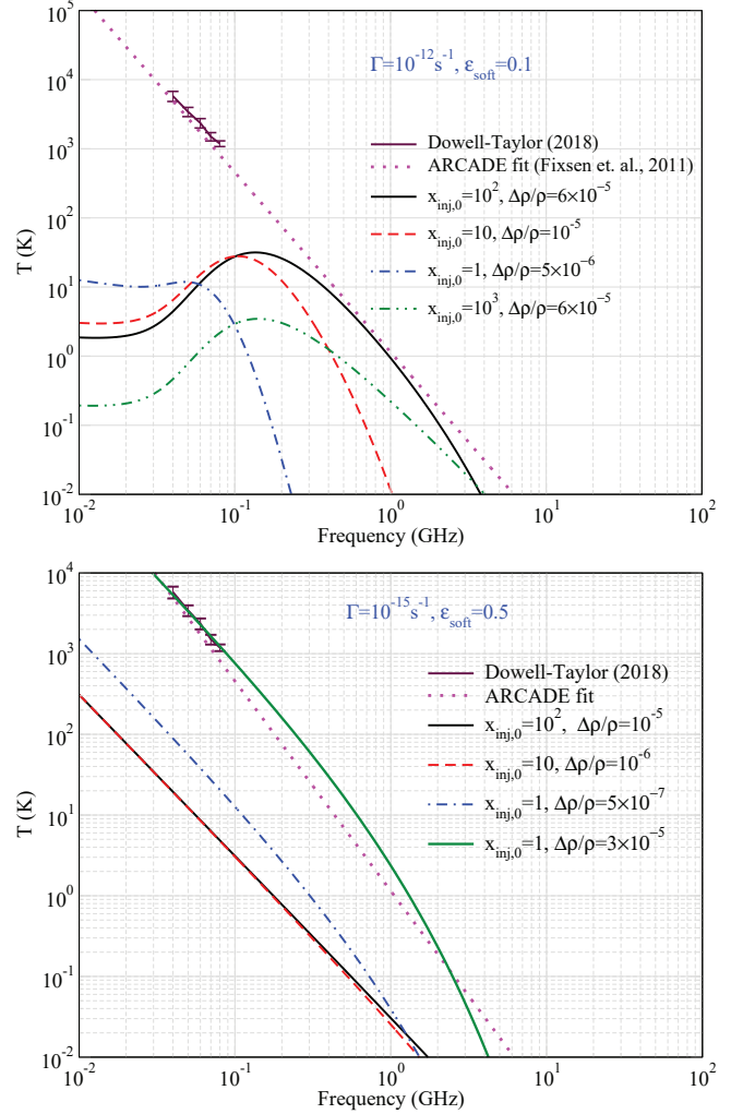
Figure 8. Spectral distortion signals created by free-free type soft photon injection from a decaying dark matter particle with lifetime t_X \simeq 10^{12} (top) and 10^{15} (bottom) second. In each case it is assumed that a fraction \epsilon_{\text{soft}} of the total energy (as labeled) is injected as soft photons. The injection frequency, x_{\text{inj},0} = h\nu_{\text{inj},0}/kT_0 is also varied with some of the shown cases coming intriguingly close to the ARCADE RSB level (figures provided by Sandeep Acharya).
