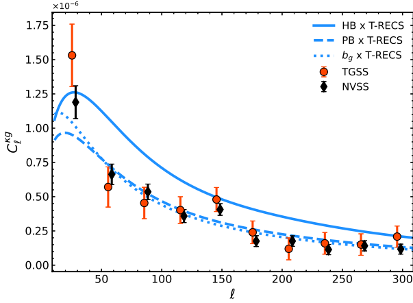
Figure 7. Measured cross-spectrum \kappa g of TGSS – CMB lensing (red dots) and NVSS – CMB lensing (black diamonds). Error bars represent the 1\sigma uncertainties obtained assuming Gaussian statistics. Blue curves represent model predictions obtained using different prescriptions for the bias, b(z) , while the T-RECS N(z) distribution of Bonaldi et al. (2018) is used (see Piccirilli et al. (2022) for a detailed description).
