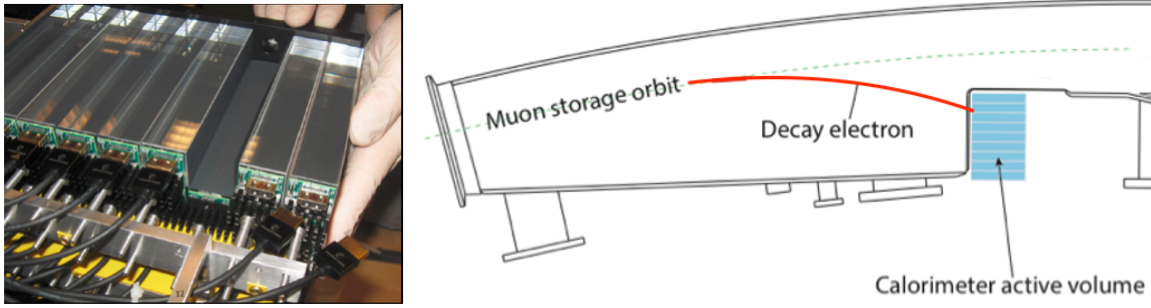
Figure 3: Left: Picture of \text{PbF}_2 crystals during calorimeter assembly, each coupled to a SiPM board (green). Right: Trajectory of emitted electron from muon decay, detected by the calorimeter.
