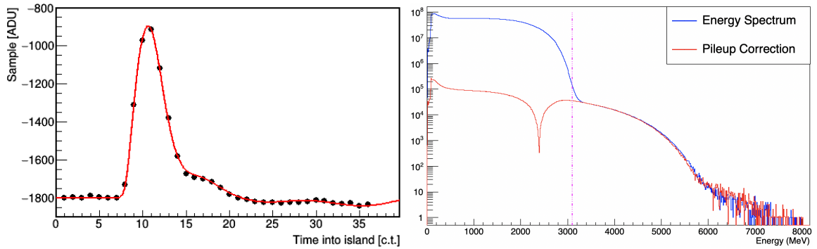
Figure 4: Left: Trace of a positron hitting a crystal, fitted with a predetermined template to obtain the time and deposited energy of the event. Right: Energy spectrum of clusters before pileup correction (blue) and absolute value of the correction (red), which would be positive until \sim 2.38 GeV and negative after that value.
