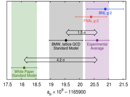
Figure 1: The Standard Model value recommended by the Muon g - 2 Theory Initiative (green band) [1] is compared to the experimental average [2] and to the evaluation by BMW collaboration using lattice QCD (grey band) [4].
