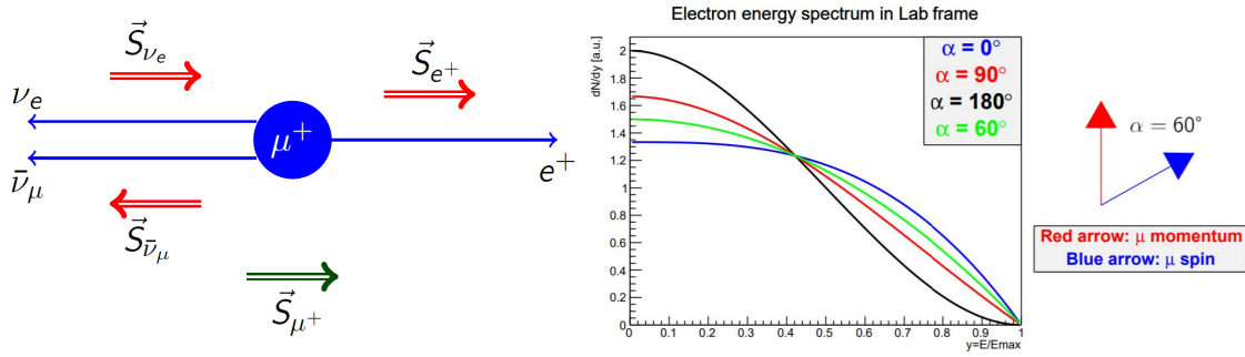
Figure 2: Left: Diagram of muon decay in the center-of-mass frame. Right: Energy spectrum of emitted positron in g - 2 laboratory frame, which changes as a function of the anomalous precession phase.
