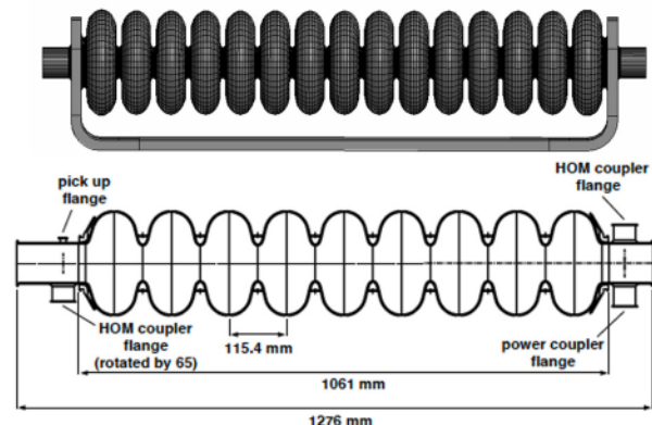
Figure 1: A one-meter-long TW structure with a 105^\circ phase advance per cell compared to the one-meter standing-wave TESLA structure [2]. Note that a TW structure for HELEN will be longer, perhaps 2-meter long.
