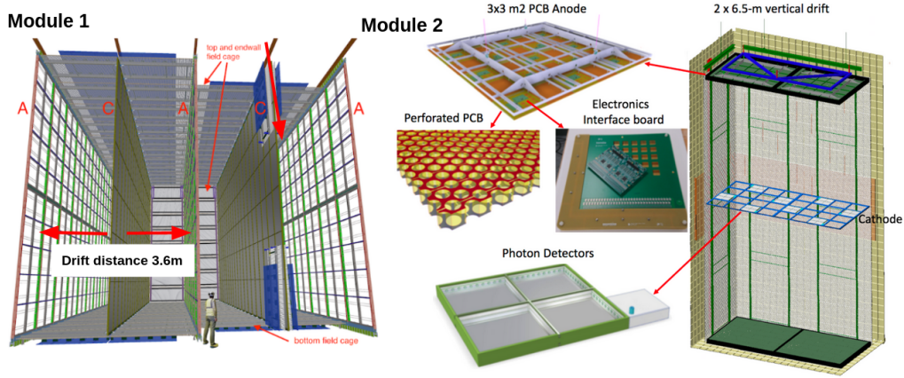
Figure 4: Sketch of the DUNE far detector module 1 (left) and module 2 (right).
