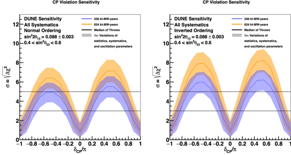
Figure 7: Sensitivity of the \delta_{CP} measurement for normal (left) and inverted (right) hierarchy. See text for detail. Figure is taken from [19].
