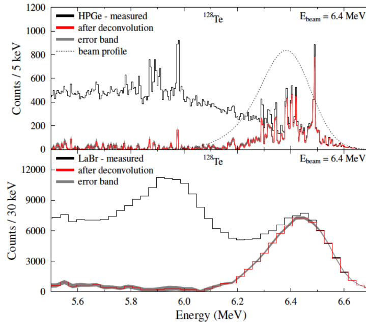
Figure 3.3: HPGe (top) and LaBr (bottom) spectra from singles \gamma -ray spectroscopy of ^{128}\text{Te} at a beam energy of 6.4 MeV. The black histograms show the actual spectra, and the red ones are the result of the deconvolution, which includes correcting for the detector response. The beam profile is indicated by a dashed curve in the upper panel. This figure is taken from [15].
