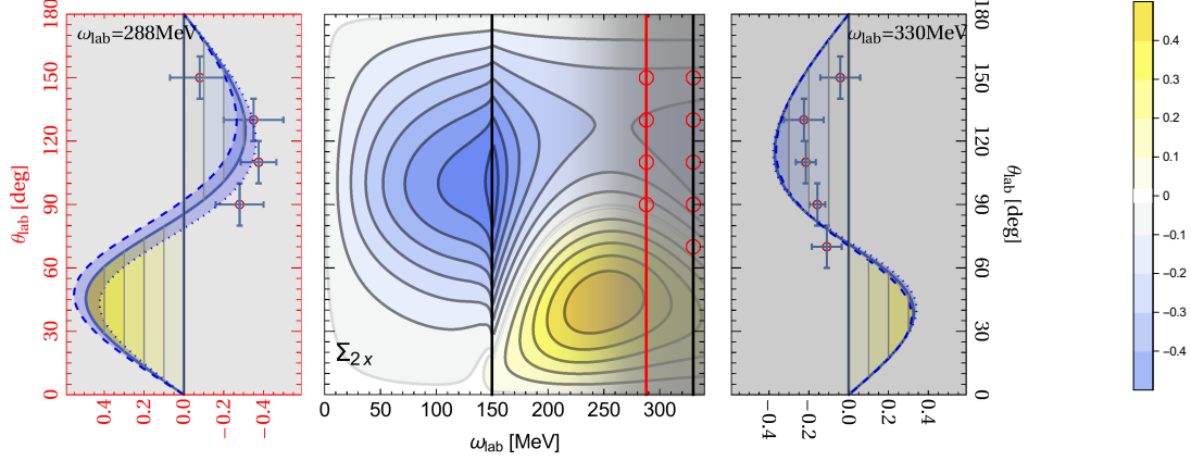
Figure 4.6: Prediction of the proton double-polarization observable \Sigma_{2x} with circularly polarized beam and transverse polarized target in EFT [30] compared to the data from MAMI [14, 15, 44, 45, 46].
