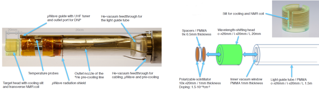
Figure 4.15: The Mainz Active Polarized Target [57].
