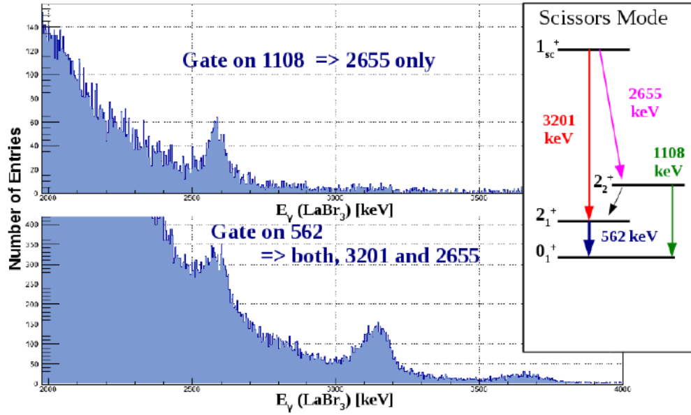
Figure 3.2: Example of \gamma - \gamma coincidence spectroscopy. The spectra show projections of \text{LaBr}_3 - \text{LaBr}_3 matrices after gating on transitions from the first and second 2^+ states in ^{76}\text{Ge} . The corresponding level scheme is given on the right-hand side. The scheme is an example for any dipole excited state with arbitrary intermediate levels between the J^\pi = 1^+ excited state and the ground state.
