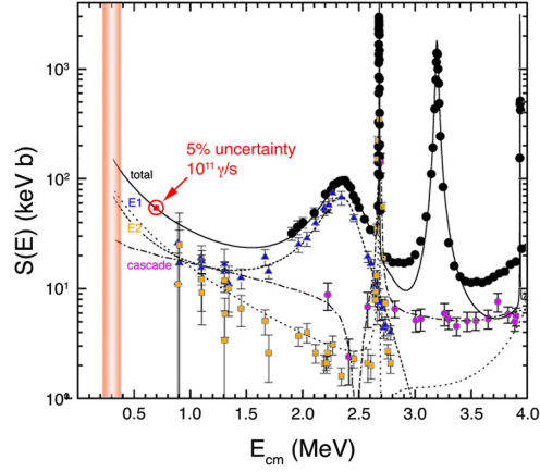
Figure 3.7: Plot of total S-factor data (filled-in circles) [76] for C(\alpha, \gamma)O compared with E1 (open triangles) and E2 (open squares) \gamma -ray measurements [77] and the E_{cm} = 6.05 MeV cascade data (open circles) [78]. The solid line represents the sum of the single amplitudes of an R-matrix fit [79], while the dotted and dashed lines are the E1 and E2 amplitudes, respectively. In addition, the R-matrix fit of [78] to their cascade data is shown as the dot-dashed line. The latter component is not included in the sum and might explain the high yield in the S-factor data between the resonances. This figure is adapted from Ref. [80].
