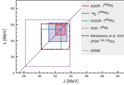
Figure 3.9: Constraints of the symmetry energy at saturation L and slope parameter J , obtained from a comparison of relativistic nuclear energy density functional results and data on anti-analog giant dipole resonance (AGDR) [91] and IVGQR [86] excitation energies in ^{208}\text{Pb} ; the dipole polarizability \alpha_D of ^{208}\text{Pb} [92]; and the PDR energy-weighted strength in ^{68}\text{Ni} [93] and ^{130,132}\text{Sn} [89]. This figure is taken from Ref. [94].
