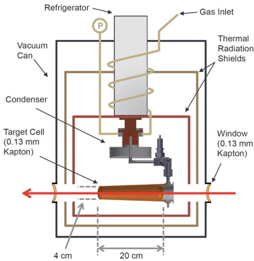
Figure 4.14: The cryotarget at HI S [53].
