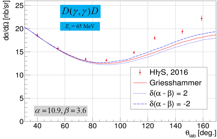
Figure 4.9: Differential cross section for elastic Compton scattering on deuterium at 65 MeV as a function of laboratory angle. The curves are EFT calculations that have been varied by \pm 2 in the polarizability difference [1, 32]. The agreement between data and theory is good at forward angles, but diverges at backward angles due to inelastic contributions.
