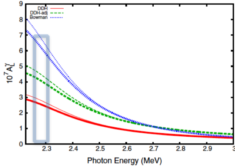
Figure 3.10: Plot of the calculated A_L^2 for parity violating photodisintegration of the deuteron as a function of photon energy. The lowest photon energy on the plot is the breakup threshold value corresponding to the deuteron binding energy. This figure is adapted from Ref. [128]. The curves represent next-to-leading-order EFT calculations using three different sets of hadronic weak coupling constants, which are labeled DDH, DDH-adj, and Bowman. DDH represents the DDH "best values" [129]. DDH-adj refers to a set in which two combinations of \bar{g}_1 and \bar{g}_2 couplings are fit to data on the longitudinal asymmetry, while the remaining couplings take the DDH "best values" [130]. The set labeled Bowman is obtained by fitting the parity violating couplings to a variety of available data [131]. The optimum energy window for the measurement is indicated by the rectangle.
