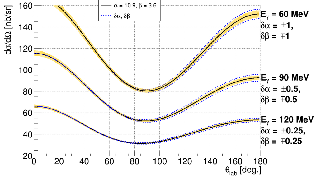
Figure 4.11: Predictions for the differential cross section for Compton scattering from He at photon laboratory energies of 60, 90, and 120 MeV in a phenomenological model [50]. The effect of varying the isoscalar \alpha and \beta while keeping their sum fixed is shown by the blue dotted lines. A combined statistical and point-to-point systematic uncertainty of 2.2% is indicated by the shaded bands.
