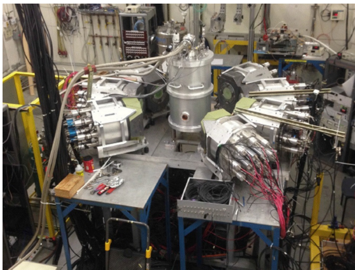
Figure 4.16: The High Intensity Gamma Source NaI Detector Array HINDA with eight NaI crystals at HI S is an example of present-day inorganic scintillators.
