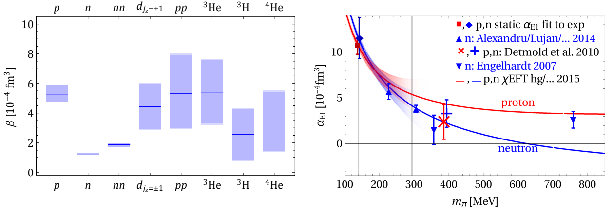
Figure 4.4: Left: Magnetic polarizabilities of nucleons and light nuclei extracted from lattice QCD computations performed at m_\pi = 800 MeV [22]. Right: Pion-mass dependence of the electric polarizabilities in \chi\text{EFT} , with experimental extractions at the physical point and available lattice results [26].
