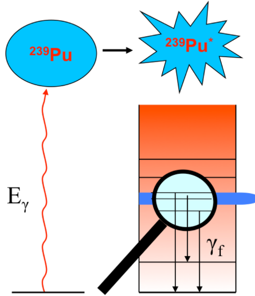
Figure 3.13: Schematic diagram of the NRF technique. First the incident photon is absorbed by a nucleus at certain resonance energies characterized by the parameters E_r , J , \Gamma . Then the excited state quickly re-emits \gamma -rays at the same or a different energy in a decay pattern that is unique for each type of nucleus. The MeV energy scale is high enough to penetrate heavily shielded containers, thus permitting non-destructive, unambiguous isotope identification and quantitative mass determination.
