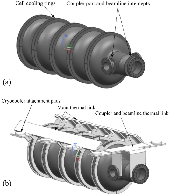
FIG. 20. (a) Rendering of the 5-cell cavity with e-beam welded cooling rings and (b) thermal links attached to the 5-cell cavity by bolting.
