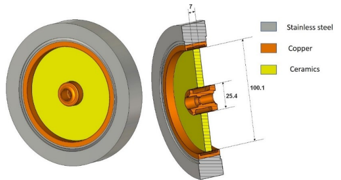
FIG. 15. Configuration and dimensions of the coupler ceramic window.
