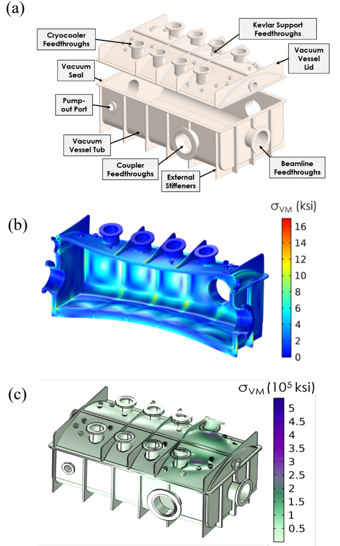
FIG. 24. (a) CAD view of the cryostat vacuum vessel made of a large tub and a lid that are sealed together (b) Distribution of von Mises stresses due to vacuum loading (displacements exaggerated 130-fold) (c) Von Mises stresses in the vacuum vessel when the first buckling failure mode occurs on one side of the lid. The loading required for this mode of failure is approximately 64 times larger than under normal loading.
