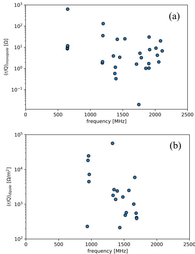
FIG. 13. Impedances of (a) monopole HOMs and (b) dipole HOMs as a function of mode frequency.
