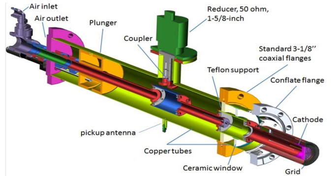
FIG. 2. RF gun design parameters (left) and components (right).
