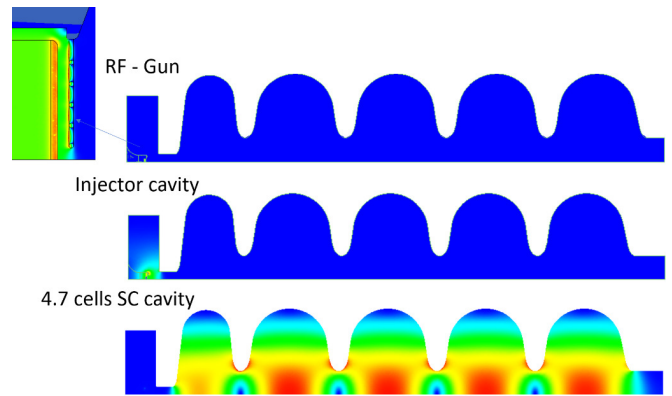
FIG. 10. The three sets of EM-fields used for MICHELLE simulation of beam transport through the accelerator.
