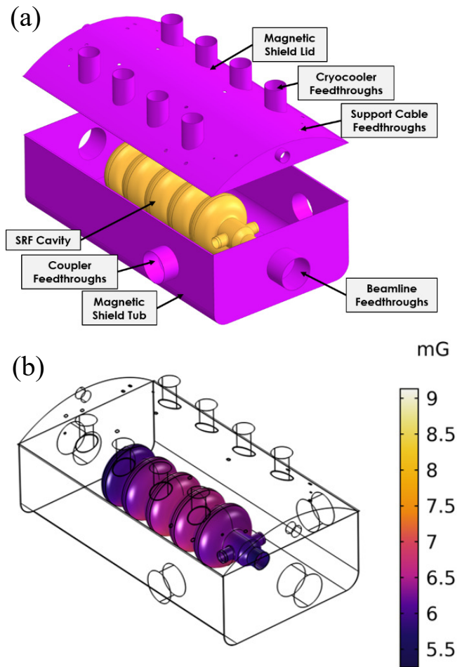
FIG. 23. (a) The exploded view of the magnetic shield shows that it is composed of two halves, a top lid and a bottom tub which are attached at a small interface flange during assembly. Chimneys are attached around each feedthrough to improve shielding (b) Magnetic flux density displayed along the surface of the SRF cavity, in the case where the beamline is oriented toward the North.
