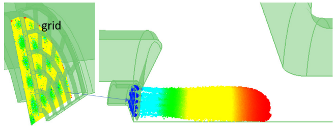
FIG. 4. Beam distribution at the time of emission from the cathode and \beta\gamma beam distribution in the middle of the injector gap.
