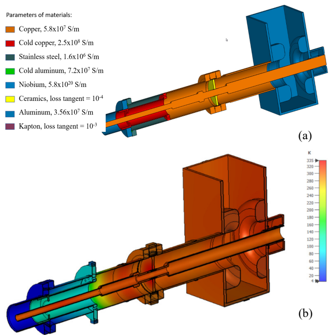
FIG. 17. Thermal analysis of the fundamental power coupler at 500 kW forward propagation (a) geometry and material properties (b) steady state temperature map.
