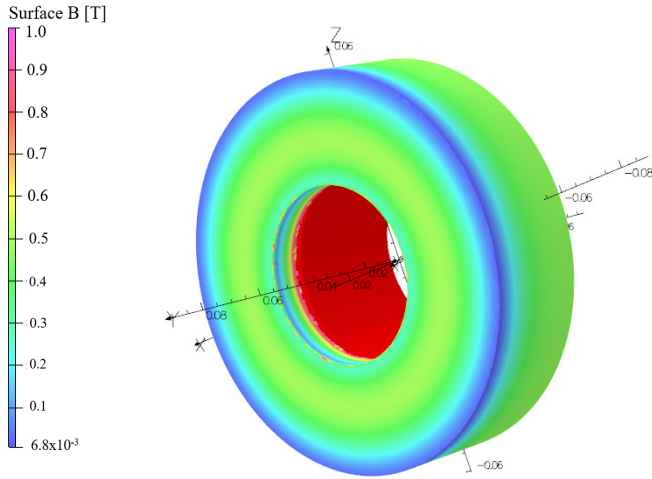
FIG. 6. Surface magnetic field produced by the solenoid (dimensions in m).
