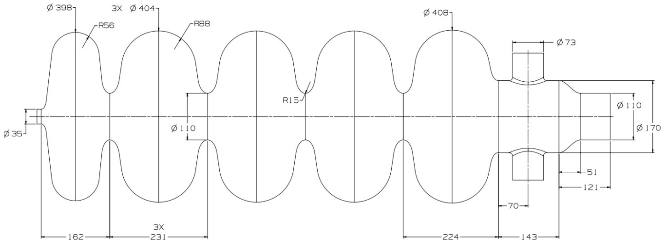
FIG. 7. Geometrical dimensions of the 5-cell cavity RF volume. All dimensions are in mm.
