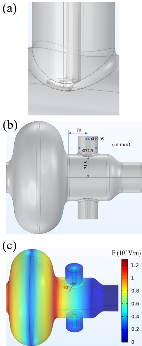
FIG. 9. 5-cell cavity coupler-side end-group (a) enlarged view of coupler antenna tip (b) dimensions of power coupler port and antenna position and (c) electric field distribution in the cavity end-group.
