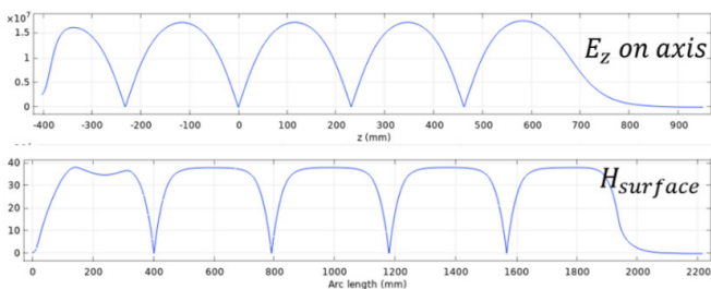
FIG. 8. Axial electric and surface magnetic field for the 5-cell cavity at 10 MV voltage gain.
