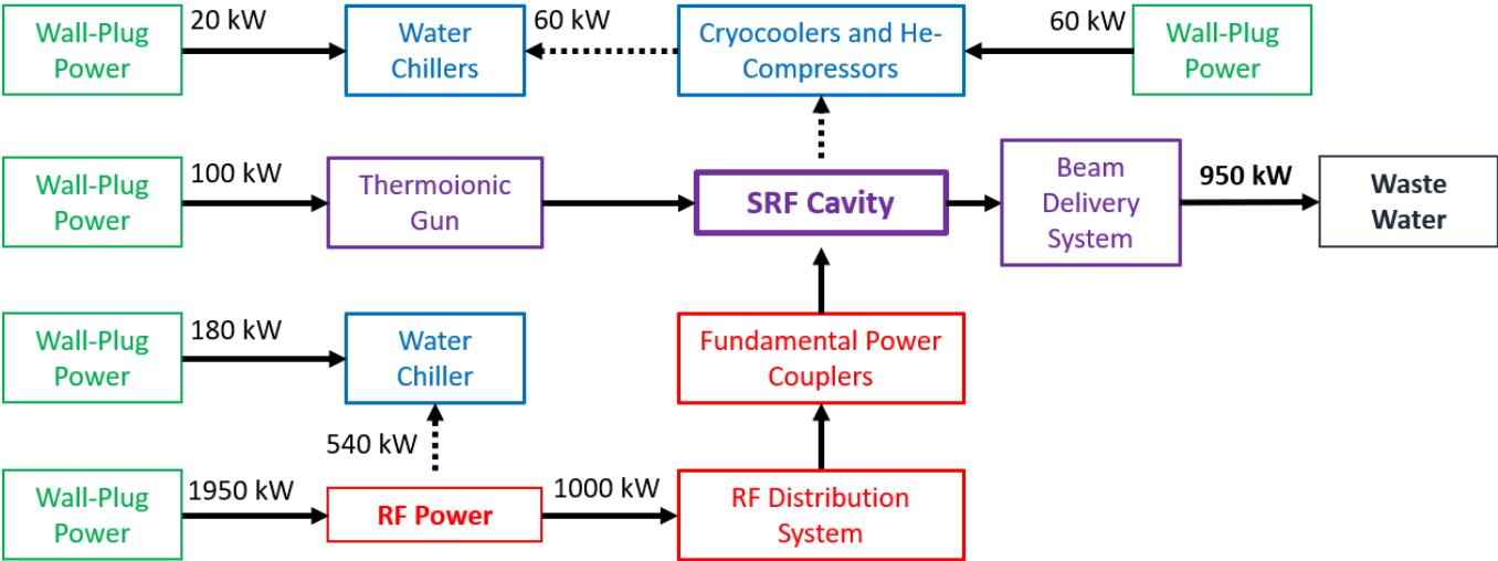
FIG. 27. Power flow diagram for the 10 MeV, 1 MW SRF accelerator.
