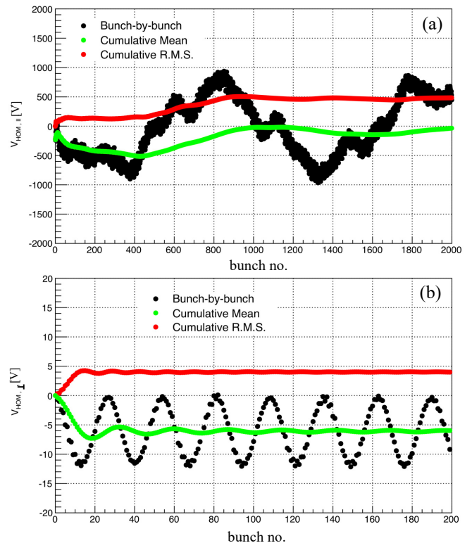
FIG. 14. (a) Monopole HOM voltage and (b) dipole HOM voltage for the 5-cell 650 MHz cavity.
