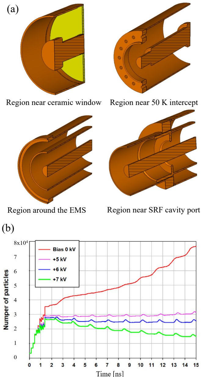
FIG. 18. (a) Vacuum side coupler sections analyzed for multipacting (b) representative observation of multipacting and mitigation by applying DC bias. A similar plot is obtained for each section but not shown here to avoid clutter.
