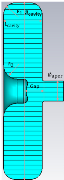
FIG. 3. Injector cavity design and operating parameters.
