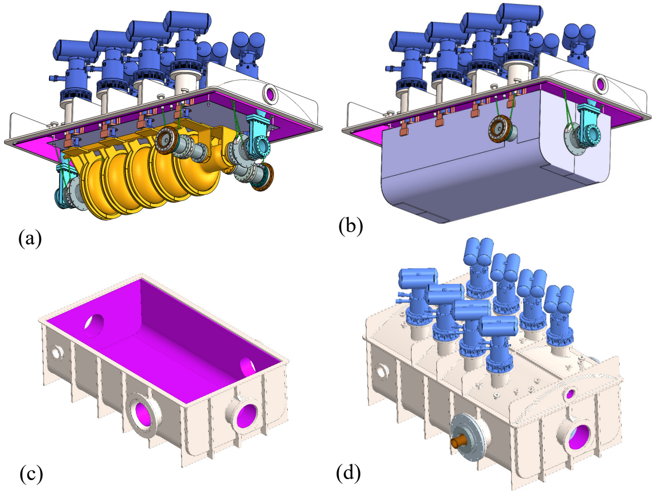
FIG. 26. Cryomodule assembly sequence (a) installation of the beamline assembly and cryocoolers on the vacuum vessel lid (b) installation of the the thermal shield (c) Installation of the bottom half of the magnetic shield inside the vacuum vessel tub and (d) fully assembled cryomodule.
