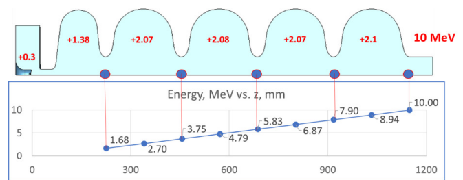
FIG. 11. Beam transport through the 5-cell SRF cavity: cell-by-cell bunch energy gain (left) and output beam parameters (right).
