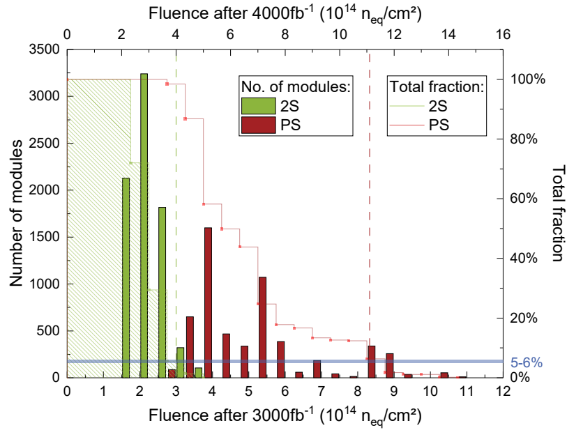
Figure 5. Distribution of the integrated fluence the modules will have received at the end of operation taking into account their locations in the CMS tracker. The lower x -axis indicates the fluence after 3000 \text{ fb}^{-1} and the upper after 4000 \text{ fb}^{-1} . Besides the histogram of the number of modules for each accumulated fluence bin, the plot includes the integrated total fraction of modules whose accumulated fluence will exceed the corresponding fluence. The green and red dashed lines indicate the maximum fluences for about 95% of modules in the 2S and PS regions, respectively. The data are based on FLUKA v3.7.20.1.
