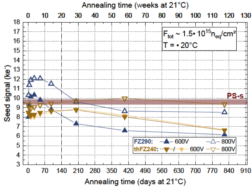
(b) Ultimate fluence for PS modules
