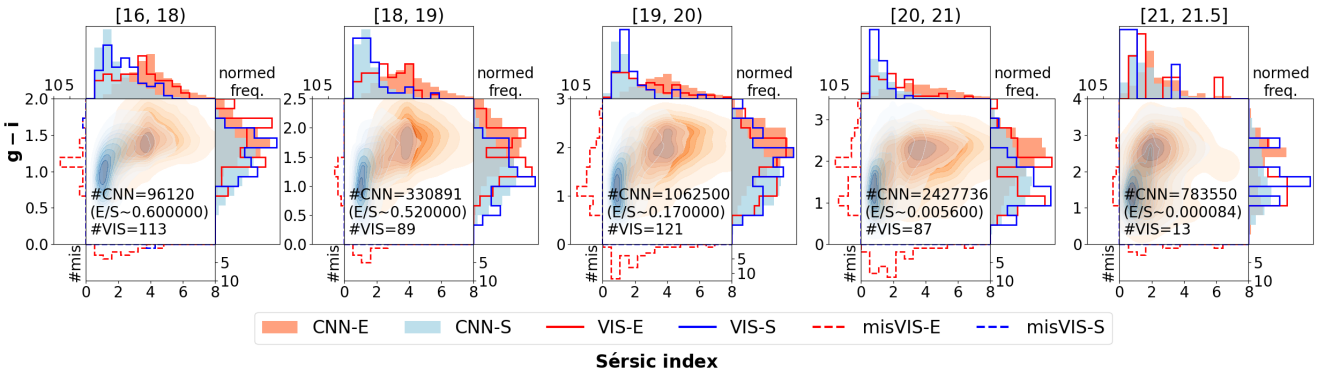
Figure 10. The diagram shows the colour and the Sérsic index distribution of our samples. The y -axis presents the colour g - i and the x -axis shows the Sérsic index. The central contour plot shows the two dimensional density distribution while the histograms at the top and the right show the normalised frequency distribution of each quantity, Sérsic index and g - i colour, respectively. The histograms at the bottom and the left show the samples with mismatched labels between the CNN and visual classifications for the Sérsic index and the colour, respectively. The red/orange colour represents the Ellipticals, while the bluish colour is for the spiral galaxies. The shadings represents the CNN predictions, and the solid lines show the distribution labelled by the visual classifications. Finally, the dashed lines show the misclassified samples with the labels from the visual classifications.
