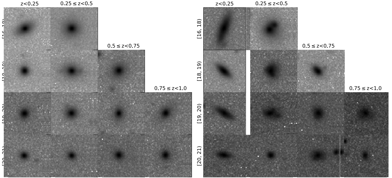
Figure 11. Examples within different magnitude and redshift bins. CNN-classified Ellipticals are shown at the left side while the right side showcases Spirals (disk galaxies). Each row and column represents a range of magnitude and redshift, respectively.
