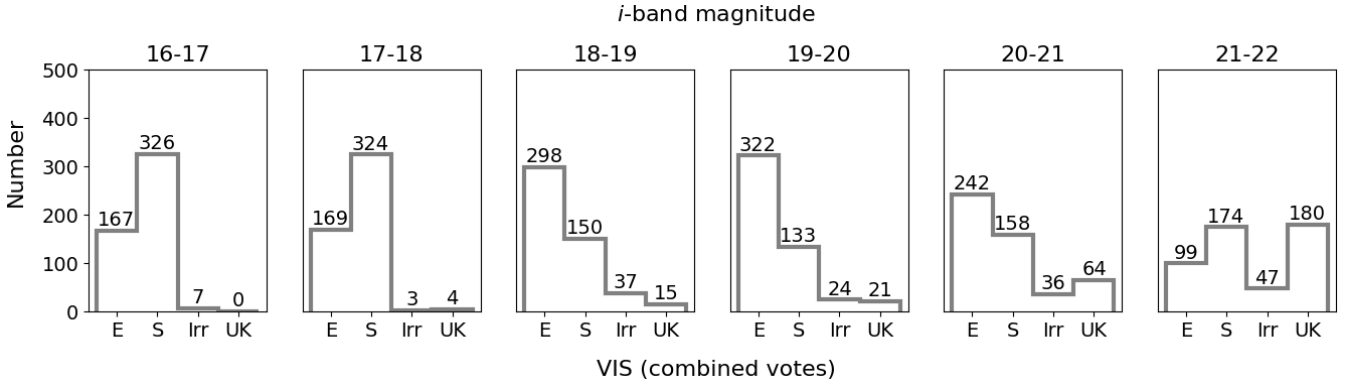
Figure 3. The frequency distribution of each visual classification in each magnitude bin. On the x-axis, ‘E’, ‘S’, ‘Irr’, and ‘UK’ is short for Ellipticals, Spirals, Irregulars, and Unknown, respectively. The number above each bar represents the number of galaxies visually classified in that category. The range of the magnitude in i -band is shown at the top of each panel.
