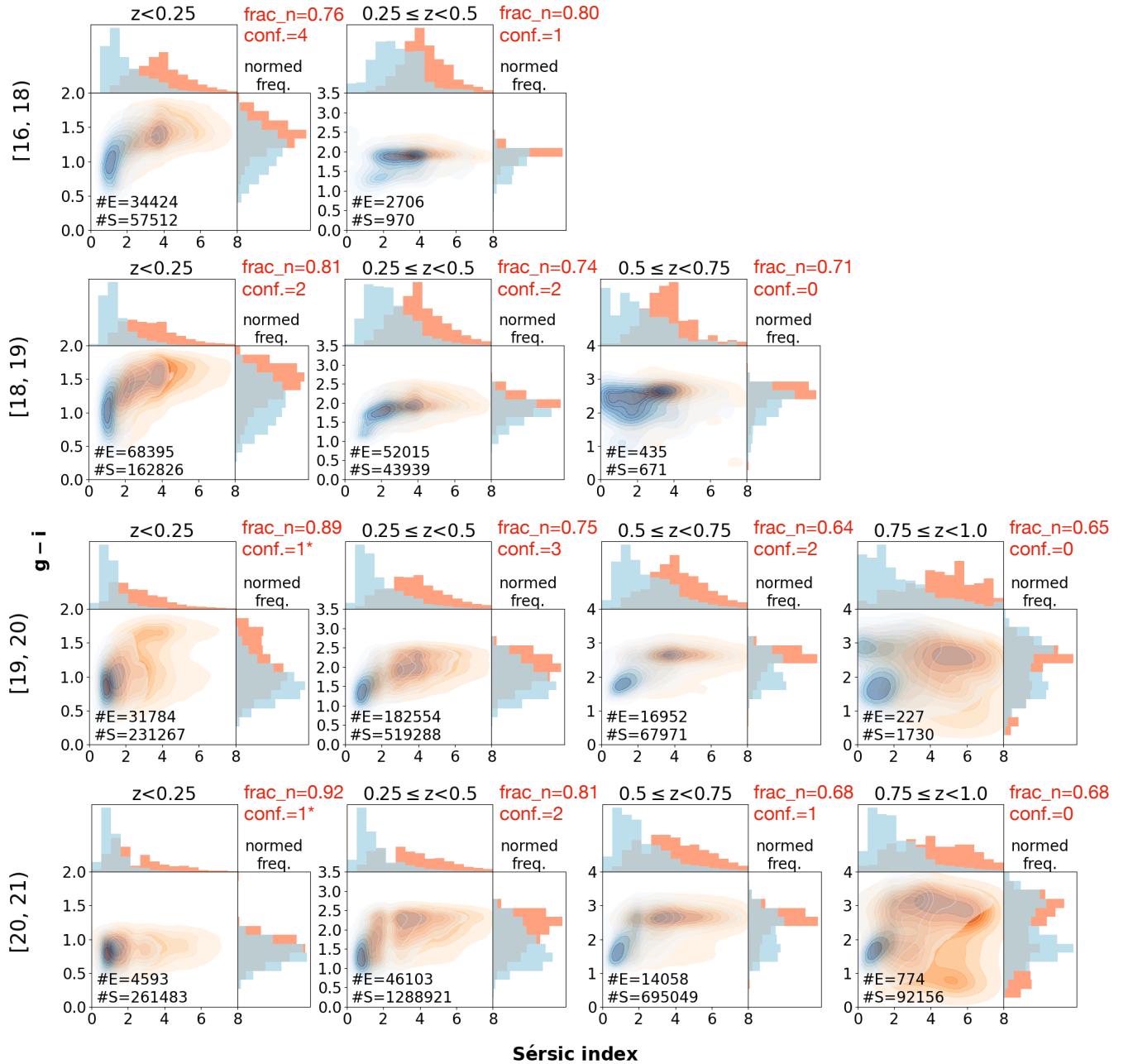
Figure 12. The colour-Sérsic diagrams of different redshift bins for each magnitude ranges. The histograms at the top and the right of each diagram show the normalised frequency distribution of Sérsic index and colour g-i , respectively. The red shading represents the Ellipticals classified by our CNN with a probability threshold of 0.5, while the blue shading shows the CNN-classified Spirals with a probability threshold of 0.5. The magnitude range is shown at the left of each row while the redshift range is presented above each graph. The textual information in the diagrams shows the number of Ellipticals (E) and Spirals (S) classified by our CNN and with the DES Y1 morphological measurements from Tarsitano et al. (2018). The red text at the top right corner of each plot indicates (1) the fraction of CNN classifications which satisfies Sérsic index criteria (frac_n; Equation 5) and (2) the confidence level (conf.) for each magnitude and redshift bin.
