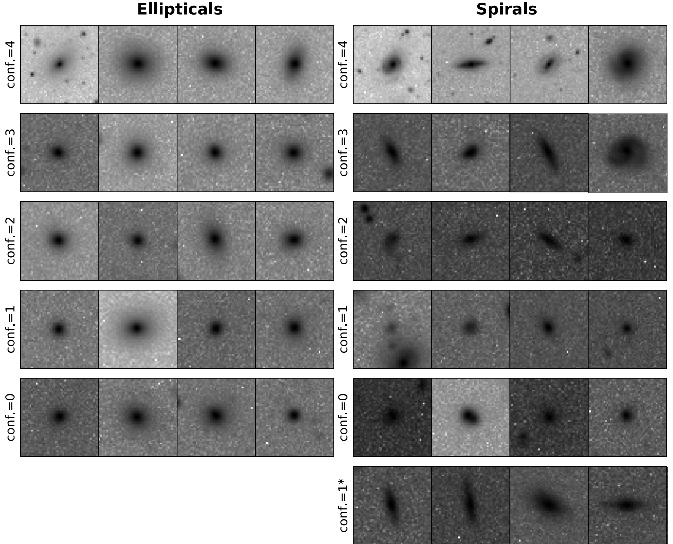
Figure 13. Examples of each confidence level (see Table 3) for the prediction of the two morphological types. The top row represents the most confident classification. CNN-classified Ellipticals are shown at the left side while the right panel presents CNN-classified Spirals. Confidence ‘1*’ is for Spirals only as explained in Table 3.
