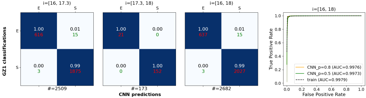
Figure 7. The combined graph of the confusion matrices and the ROC curve comparing our CNN predictions with the GZ1 labels defined by the debiased votes with a threshold of 0.8. The first three panels show the confusion matrices within certain magnitude ranges: 16 \leq i < 17.3 , 17.3 \leq i < 18 , and 16 \leq i < 18 , where the CNN predictions use a probability threshold of 0.8. The red or green colour in each quadrant represent the number of galaxies that agree with the classifications derived through CNN predictions and GZ1 classifications within each quadrant. The number above it indicates the fraction of these galaxies within each certain type decided by our CNN classifier. The number of galaxies within each magnitude range is shown below each graph.
