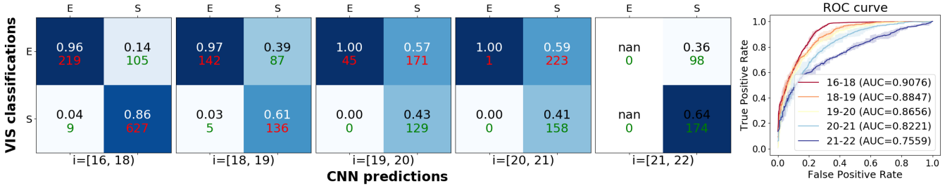
Figure 9. The confusion matrices and the ROC curve of different magnitude ranges. The x -axis of the confusion matrices is the CNN predictions with a probability threshold of 0.8 and the y -axis is our visual classifications. On the ROC curve, the x -axis is the false positive rate while the y -axis represents the true positive rate. Different colours indicate different magnitude ranges.
