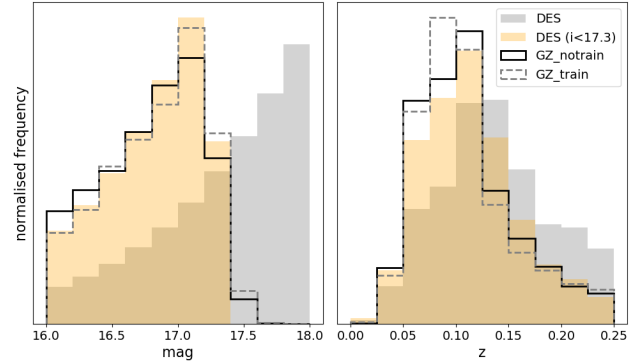
Figure 5. The magnitude and redshift distribution of the DES Y3 data with the same coverage as the training set (Section 2.2). The gray and yellow shading represents the DES Y3 data without and with a cut at i = 17.3 , respectively. The solid lines show the overlap region with the GZ1 catalogue, excluding the training set, while the dashed lines show only the training set.
