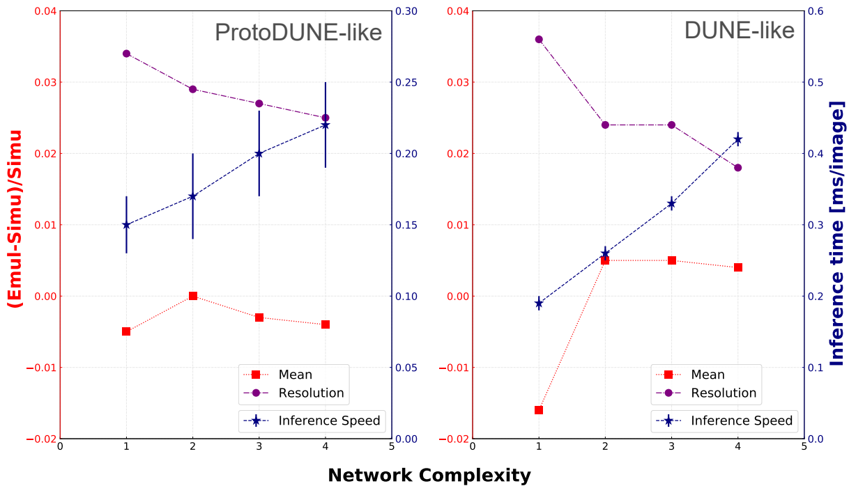
FIG. 6. Precision ( y axis on the left), inference time ( y axis on the right), and neural network complexity.
