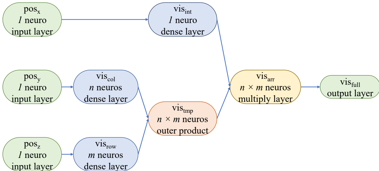
FIG. 1. General GENN architecture. pos_y -layer and pos_z -layer are used to predict the photon distribution on the photon detection system, while pos_x -layer is a normalization factor for the number of total detected photons. OuterProduct layer expands the dimension of the inputs.
