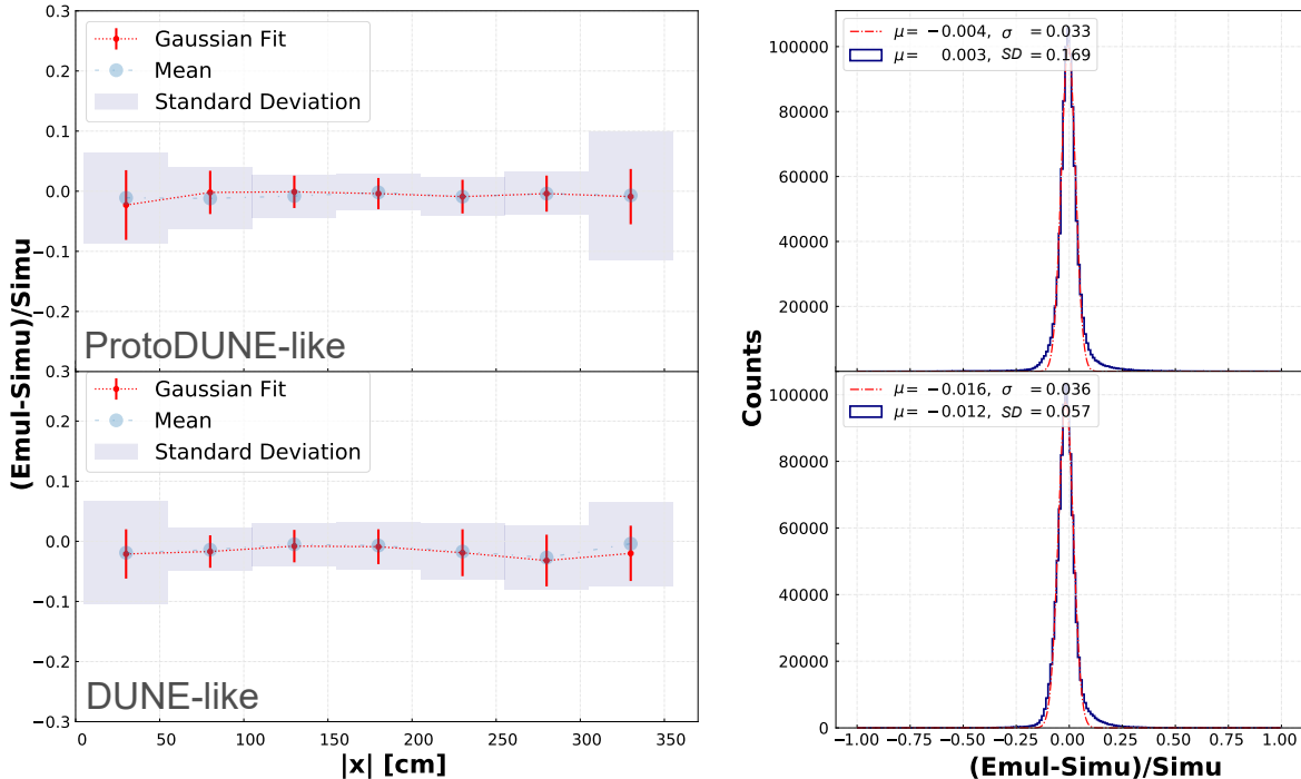
FIG. 4. Discrepancy of total detected photons per scintillation vertex. Left: discrepancies variation along the x -direction, which is the distance to the photon detector array. Right: overall discrepancies, where the red dashed line is a Gaussian fit. Comparison for ProtoDUNE-like geometry is on the top and DUNE-like geometry on the bottom. Note, due to the large sample sizes, the uncertainties on the mean values and resolutions are negligible.
