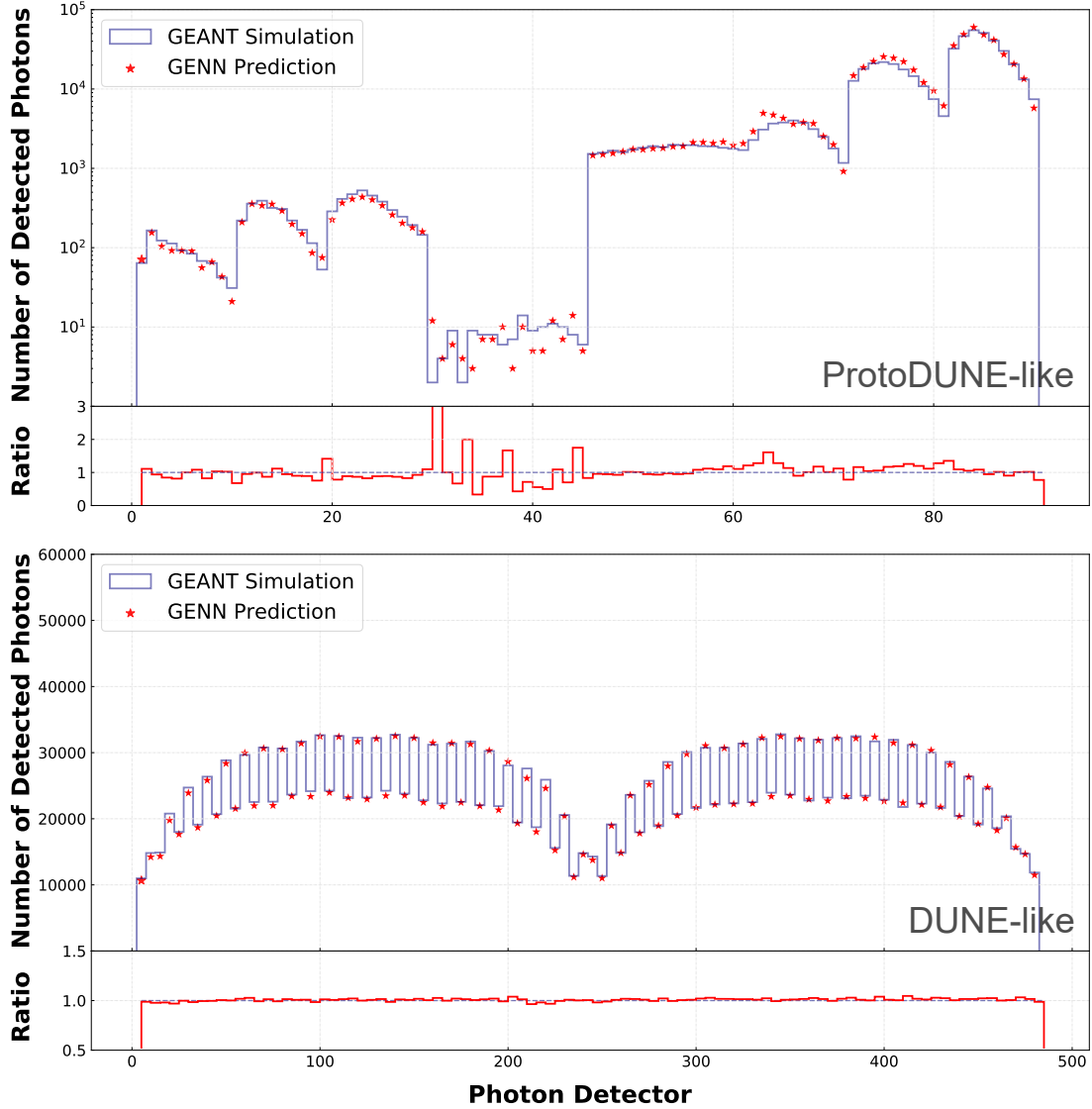
FIG. 5. Distribution of the detected photons on photon detection system. Top: the sum of detected photons on photon detectors from 200 MeV monoenergetic muon events starting from one specific position in the ProtoDUNE-like geometry. The response is much lower and scattered around photon detector #40 is caused by the fact that those photon detectors are the segmented ones which are much smaller than the bar-like light collectors. Bottom: the sum of detected photons on photon detectors from supernova neutrinos uniformly distributed in the DUNE-like geometry.
