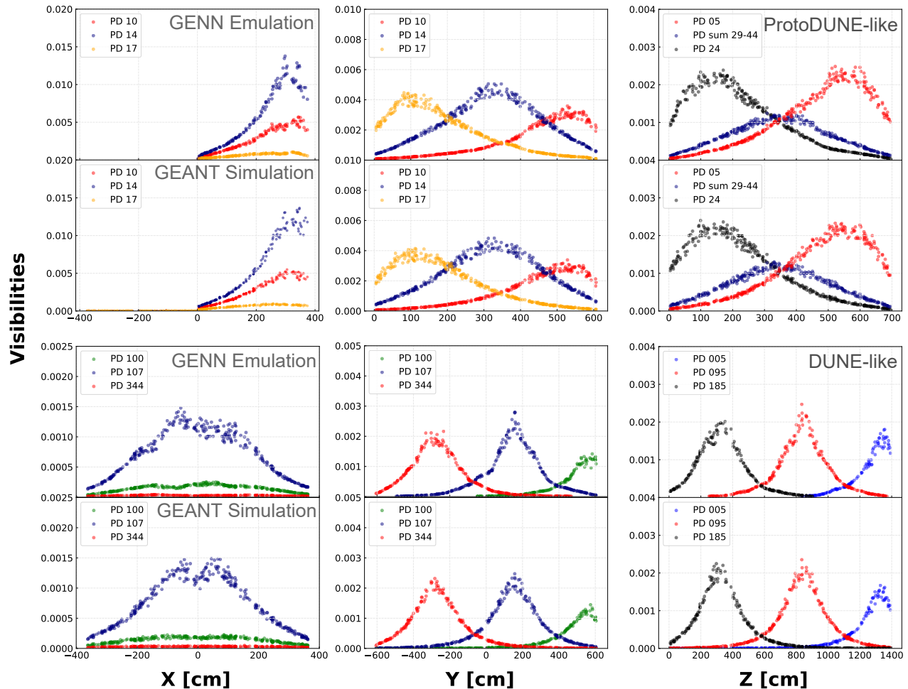
FIG. 3. Feature-learning capability. In each figure, the horizontal axis is the position of the light sources along specific directions: x , y , and z direction, while the vertical axis shows the photon detection probabilities (visibilities), on particular photon detectors (PDs). The top two rows show the visibilities in ProtoDUNE-like geometry while the bottom two are for the DUNE-like geometry. The visibilities from GENN prediction are plotted on the first and third rows and those from GEANT4 simulation are on the second and fourth rows. Note: positions of particular PDs and light sources are shown in TABLE. I.
