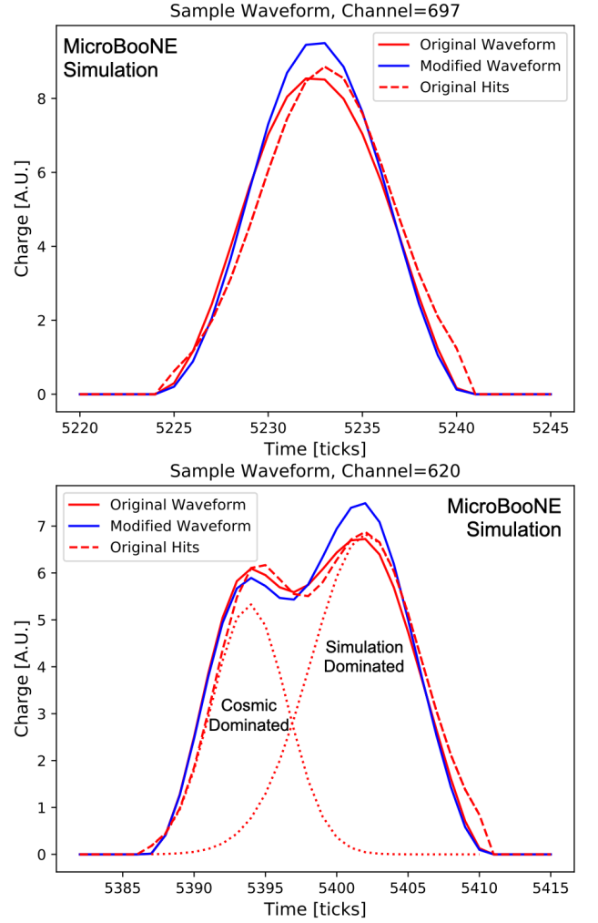
FIG. 10. Examples of modified waveforms. The top graph shows a simple example where the wire signal region is well-described by a single Gaussian function. The bottom graph shows a case where one portion of the waveform is associated to simulated charge while the other is associated with cosmic data charge. Here, the simulation-dominated portion of the waveform is modified but the cosmic-dominated portion is not.
