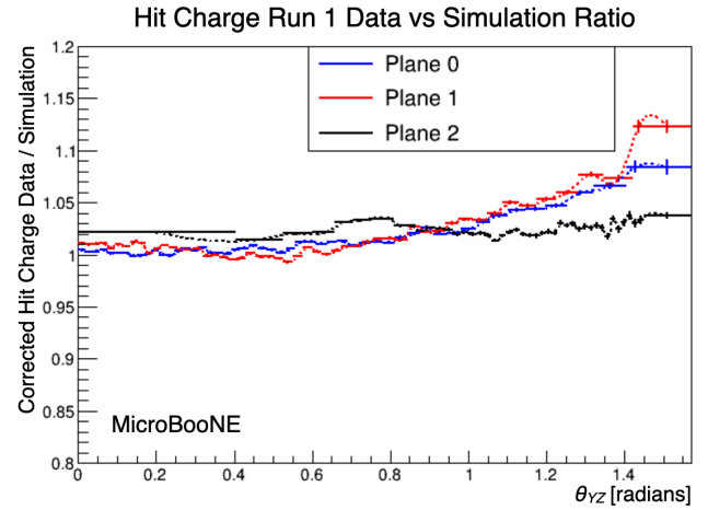
FIG. 9. Ratio functions (data/simulation) for hit charge vs. \theta_{YZ} . The solid lines are the values of the ratio in each bin, and the dashed lines are the spline fits. The bin at 1.4 < \theta_{YZ} < \pi/2 rad is extrapolated as described in the text.
