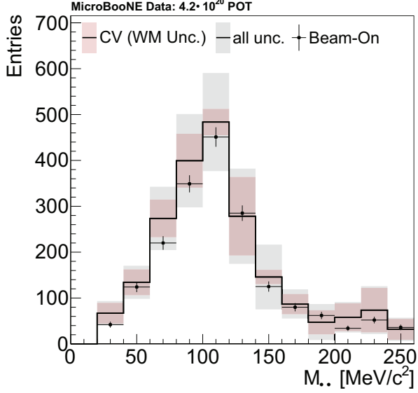
FIG. 12. Measured diphoton invariant mass distribution using BNB beam data (points) and central value (CV) simulation (black line), prior to additional shower energy corrections. The red band indicates the uncertainty from the wire modification alone. The gray band indicates the full uncertainty, including other detector uncertainties, as well as uncertainties on the neutrino flux and the interaction model. The bands represent the uncertainty calculated using Equation 8 where p is the number of events in the bin, and are symmetric. The error bars on the data are statistical only.
