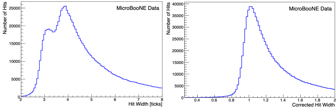
FIG. 6. Distribution of hit widths on the collection plane for -10 < y < 0 cm in the cosmic data. On the left, this distribution before any correction for the hit width dependence on x . The “double-peak” structure is evident, where the low-width peak comes from ACPT trajectory points near the anode and the high-width peak comes from points near the cathode (see Figure 4). On the right, the x -correction has been applied and the double-peak structure is removed. A time tick translates to 0.5 \mu\text{s} [1].
