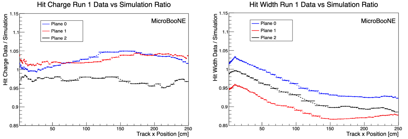
FIG. 5. Ratios (data/simulation) and fitted simulation modification functions for mean hit charge and mean hit width vs. x on each of the three wire planes. The solid lines are the bin values, with error bars showing the statistical uncertainties, and the dashed lines are spline fits. The width of each bin is indicated by the solid horizontal bars. The binning is chosen to ensure high statistics in each bin.
