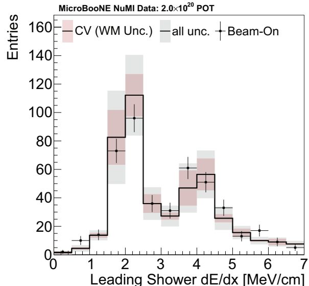
FIG. 11. Distribution of the shower dE/dx using NuMI beam data (points) and central value (CV) simulation (black line). The red band indicates the uncertainty from the wire modification alone. The gray band indicates the full uncertainty, including other detector uncertainties as well as uncertainties on the neutrino flux and the interaction model. The bands represent the uncertainty on the number of events in that bin, calculated using Equation 8, and are symmetric. The error bars on the data are statistical only.
