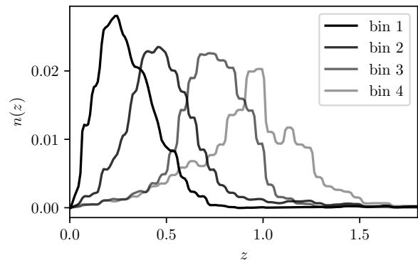
Figure 1. Redshift distributions as estimated in data for the four DES Y3 tomographic bins [75].
