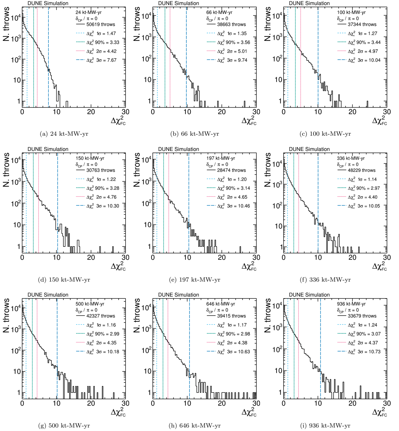
FIG. 19. Distribution of \Delta\chi^2 values, calculated using Equation 5, for a large number of throws with true \delta_{CP} = 0 , for a variety of exposures. The \Delta\chi_c^2 values (vertical lines) obtained using the Feldman-Cousins method show the \Delta\chi_{FC}^2 value below which 68.27% (1 \sigma ), 90%, 95.45% (2 \sigma ) and 99.73% (3 \sigma ) of throws reside, with the calculated values given in the legend. The number of throws used is also given.
