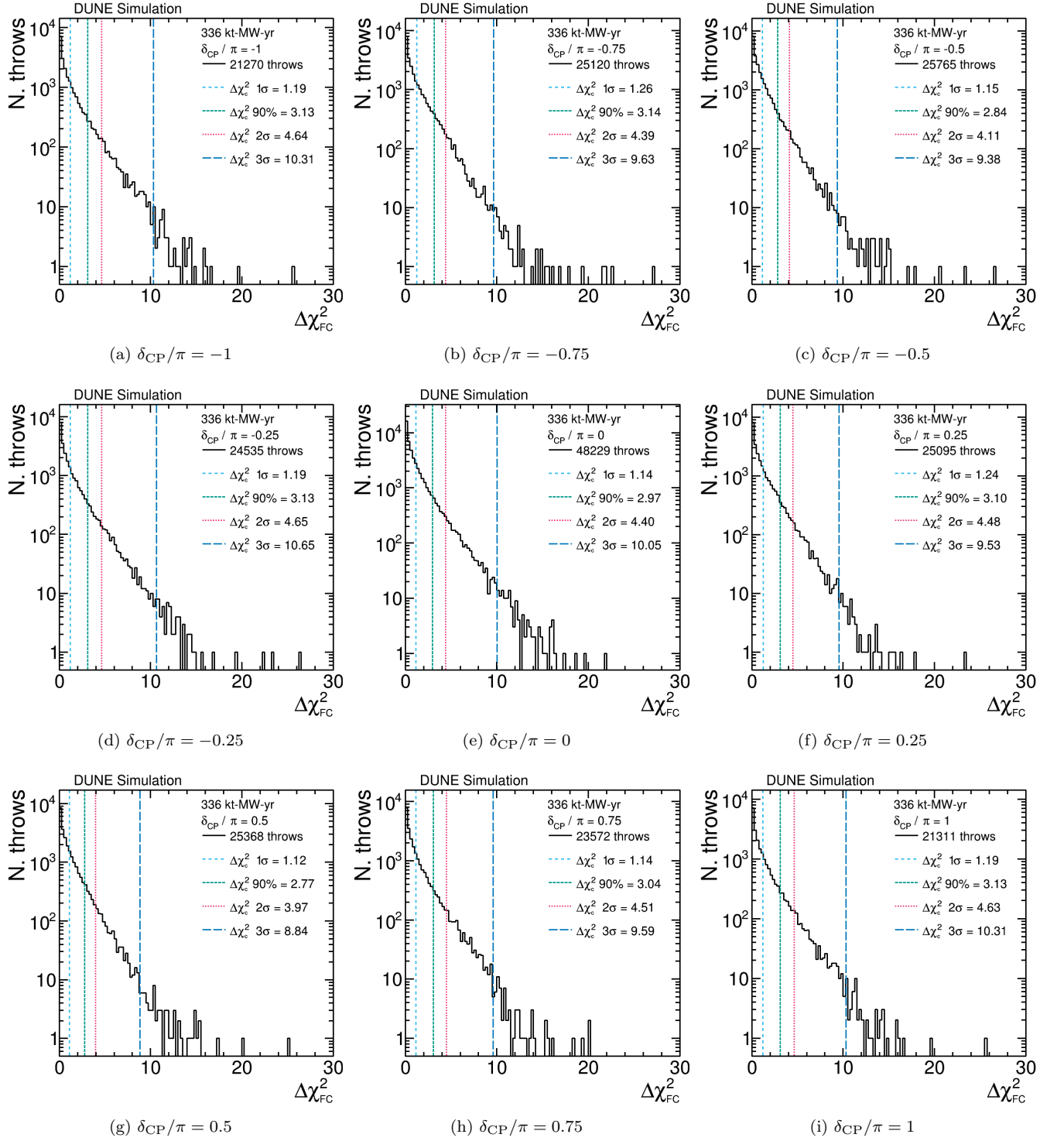
FIG. 21. Distribution of \Delta\chi^2 values, calculated using Equation 5, for a large number of throws for 9 different values of true \delta_{CP} , for a 336 kt-MW-yr exposure. The \Delta\chi^2_{FC} values (vertical lines) obtained using the Feldman-Cousins method show the \Delta\chi^2_{FC} value below which 68.27% ( 1\sigma ), 90%, 95.45% ( 2\sigma ) and 99.73% ( 3\sigma ) of throws reside, with the calculated values given in the legend. The number of throws used is also given.
