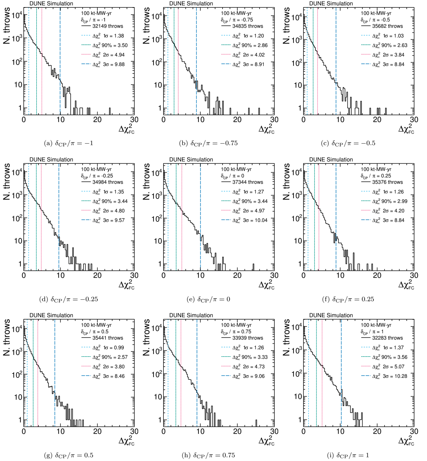
FIG. 20. Distribution of \Delta\chi^2 values, calculated using Equation 5, for a large number of throws for 9 different values of true \delta_{CP} , for a 100 kt-MW-yr exposure. The \Delta\chi_c^2 values (vertical lines) obtained using the Feldman-Cousins method show the \Delta\chi_{FC}^2 value below which 68.27% ( 1\sigma ), 90%, 95.45% ( 2\sigma ) and 99.73% ( 3\sigma ) of throws reside, with the calculated values given in the legend. The number of throws used is also given.
