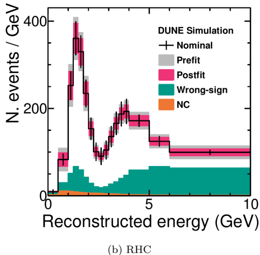
FIG. 3. Reconstructed energy distribution of selected CC \langle \bar{\nu}_\mu \rangle -like events in the FD, for 50 kt-MW-yr exposure in both FHC and RHC beam modes, for a total 100 kt-MW-yr exposure. The plots are shown for NO, all other oscillation parameters are set to their NuFIT 4.0 best-fit values (see Table I). The size of the systematic uncertainty bands from all of the flux, cross-section and ND detector systematics used in the analysis are shown, as well as the postfit uncertainty bands with parameters constrained by ND data. NC backgrounds and wrong-sign contributions to the event rate are also shown.
