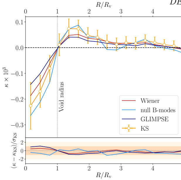
Figure 13. Top panel: Void imprints on the DES mass maps. Bottom panel: Differences of signals measured from different mass maps, relative to the KS results and errors (shaded ranges are 1\sigma and 2\sigma about the KS signal).
