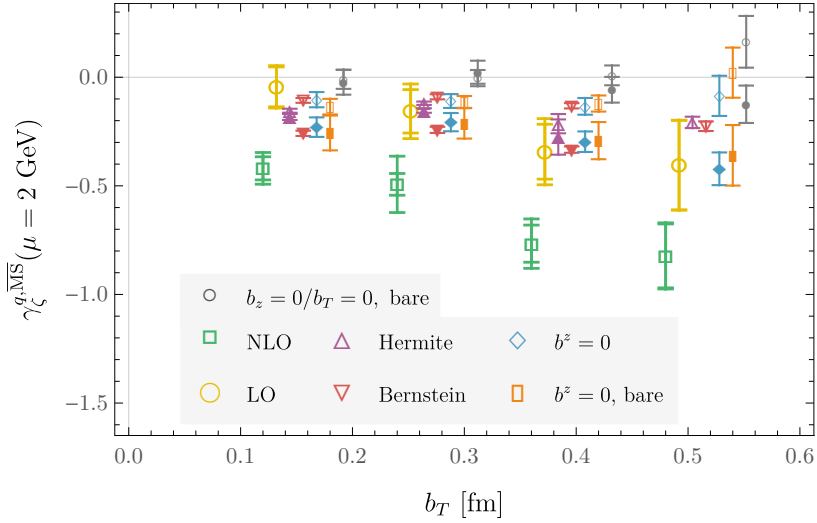
FIG. 14. b_T -dependence of the Collins-Soper kernel computed from the same quasi beam functions via the different approaches defined in Sec. III D. All points other than the primary results of this work (“NLO”) are offset on the horizontal axis for clarity. For the “NLO” and “LO” approaches, results computed based on quasi beam functions with Dirac structures \gamma^4 and \gamma^3 are combined as described in the text; the outer error bars include half the difference between the results with \gamma^4 and \gamma^3 combined in quadrature with the average uncertainty, shown by the inner error bars. For the other approaches the empty (filled) points show results obtained with Dirac structure \gamma^4 ( \gamma^3 ). “Hermite/Bernstein” points with Dirac structure \gamma_3 are not shown at b_T/a = 4 because the corresponding fits of the P^z b^z -dependence of the relevant quasi beam functions were of poor quality, as described in the text.
