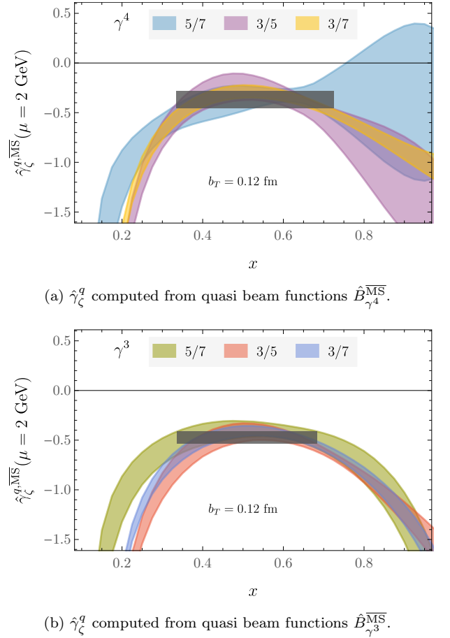
FIG. 12. \hat{\gamma}_{\zeta}^q , computed as defined in Eq. (28) for all momentum pairs \{P_1^z, P_2^z\} , denoted by P_1^z/P_2^z in the legend. The horizontal shaded band shows the fit window in x , as well as the total uncertainty of the best result, determined as described in the text.
