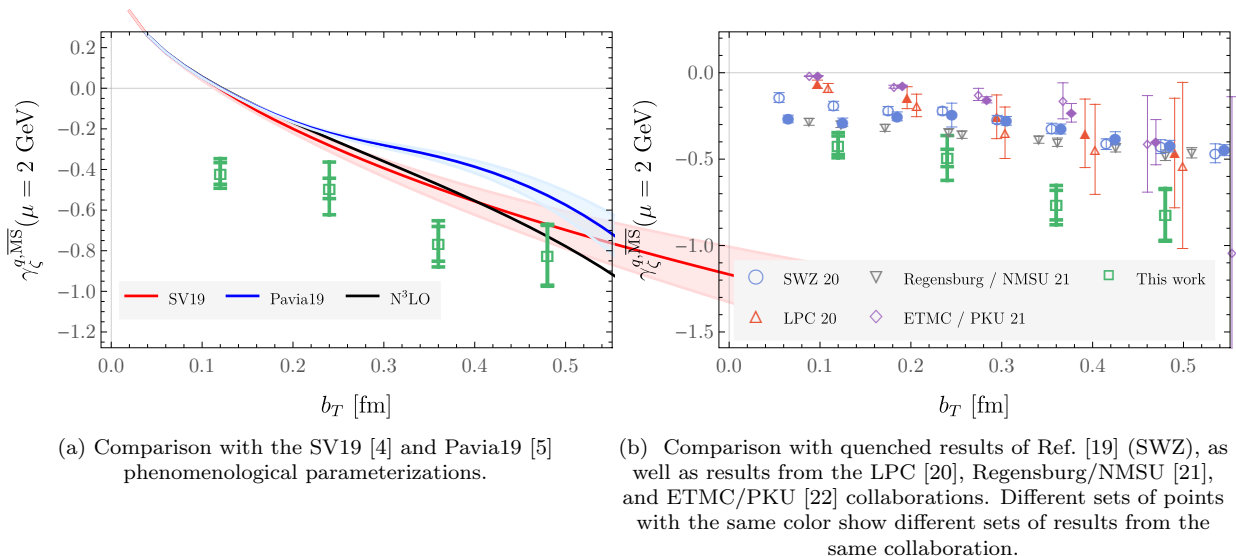
FIG. 15. b_T -dependence of the Collins-Soper kernel as determined in this work (green squares in both panels) compared with (a) phenomenological results, and (b) the results of other lattice QCD calculations of this quantity.
