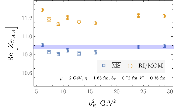
FIG. 5. Example of numerical results for Z_{O_{\gamma^4 \gamma^4}}^{RI'/MOM} (orange circles) and Z_{O_{\gamma^4 \gamma^4}}^{\overline{MS}} (blue squares), computed using the different values of p_R given in Table II, for operator geometry \eta/a = 14 , b^z/a = 3 , b_T/a = 3 , at renormalization scale \mu = 2 GeV. The blue shaded band shows the value used in further analysis, obtained as described in the text.
