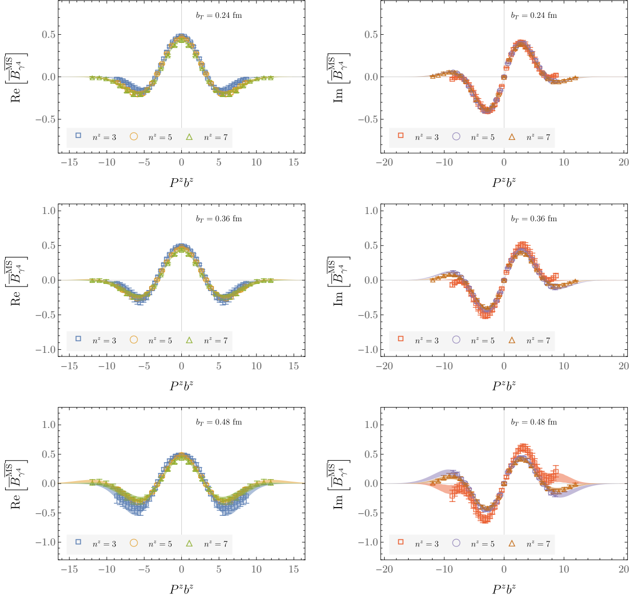
FIG. 23. Examples of the averaged asymmetry-corrected modified \overline{\text{MS}} -renormalized quasi beam functions \overline{B}_{\gamma^4}^{\text{MS}} , including fits by Eqs. (26) and (27) to the real and imaginary parts, shown as shaded bands. Fig. 11 of the main text shows the example for b_T = 0.12 fm.
