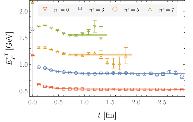
FIG. 2. Effective energy function defined in Eq. (14) for pion states boosted in the \hat{z} -direction with P^z = n^z 2\pi/L . Shaded bands display the result of single-exponential fits to the two-point correlation functions with the largest two momenta, and two-exponential fits to those with the smallest two momenta, obtained as described in the text.
