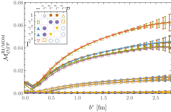
FIG. 4. Submatrix of the RI'/MOM mixing matrix \mathcal{M}_{O, \Gamma p}^{RI'/MOM} , defined in Eq. (24), computed for quark bilinear operators with straight Wilson lines ( b_T = 0 ) with various extents b^z , for momentum n^\nu = (12, 12, 12, 12) in lattice units. Points representing Dirac structures in the upper triangle of the mixing matrix are slightly offset on the horizontal axis for clarity.
