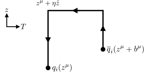
FIG. 1. Diagrammatic representation of the Wilson line included in the operators \mathcal{O}_i^i(b^\mu, z^\mu, \eta) , see Eq. (4).
