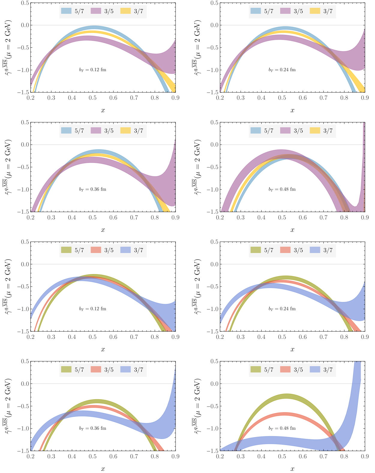
FIG. 26. \hat{\gamma}_{\zeta}^q computed as defined in Eq. (28) with a DFT of \overline{B}_{\Gamma}^{\overline{\text{MS}}} replacing the Fourier transform of analytic fits \hat{B}_{\Gamma}^{\overline{\text{MS}}} to the P^z b^z -dependence of the quasi beam functions, for momentum pairs \{P_1^z, P_2^z\} denoted by P_1^z/P_2^z in the legend.
