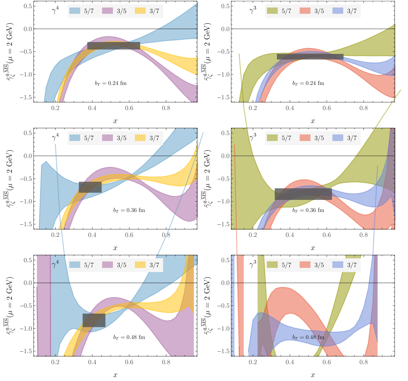
FIG. 25. \hat{\gamma}_{\zeta}^q computed as defined in Eq. (28) for momentum pairs \{P_1^z, P_2^z\} , denoted by P_1^z/P_2^z in the legend. The horizontal shaded band shows the total uncertainty of the best result, and the corresponding x -window, determined as described in the text. Fig. 12 of the main text shows the analogous results for b_T = 0.12 \text{ fm} .
