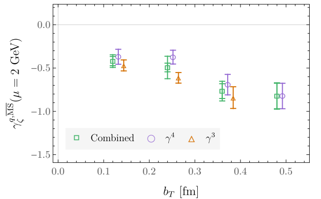
FIG. 13. Collins-Soper kernel as a function of b_T , determined from \hat{B}_{\gamma^4}^{\overline{\text{MS}}} (purple circles) \hat{B}_{\gamma^3}^{\overline{\text{MS}}} (red triangles), and the final combined results of this work (green squares), computed as described in the text. For the latter points, the inner (outer) error bars show the first (quadrature-combined) uncertainties given in Table. III.
