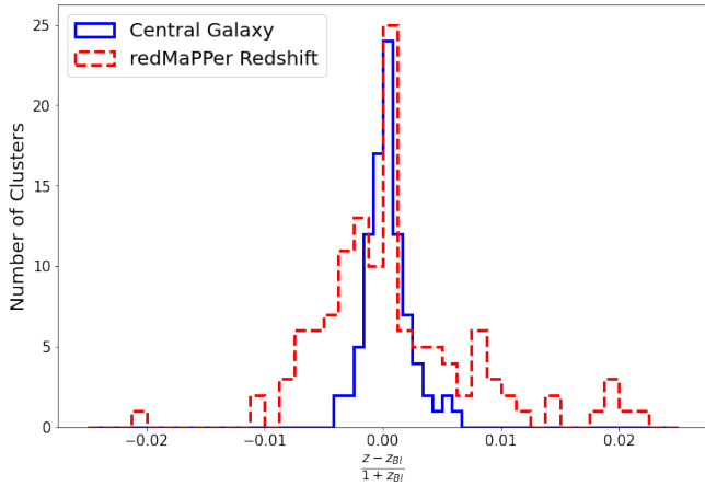
Figure 5. Difference in redshift between the biweight location estimate of the central cluster redshift and the redMaPPer estimated cluster redshift in z = 0.00083 wide bins (dashed red). Difference in redshift between the biweight location estimate and the redMaPPer central galaxy spectroscopic redshift where available in z = 0.0013 wide bins (solid blue).
