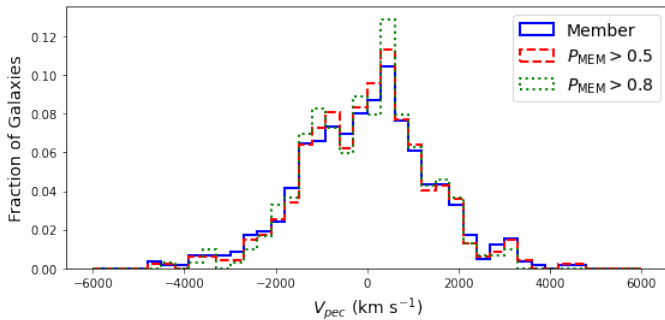
Figure A4. Histogram of the fractions of galaxies from outlier clusters stacked together in peculiar velocity bins for all member galaxies (solid blue), galaxies with P_{\text{MEM}} > 0.5 (dashed red), and galaxies with P_{\text{MEM}} > 0.8 (dotted green). These distributions are extremely similar, and limiting our sample based on P_{\text{MEM}} does not reduce or eliminate the outlier population.
