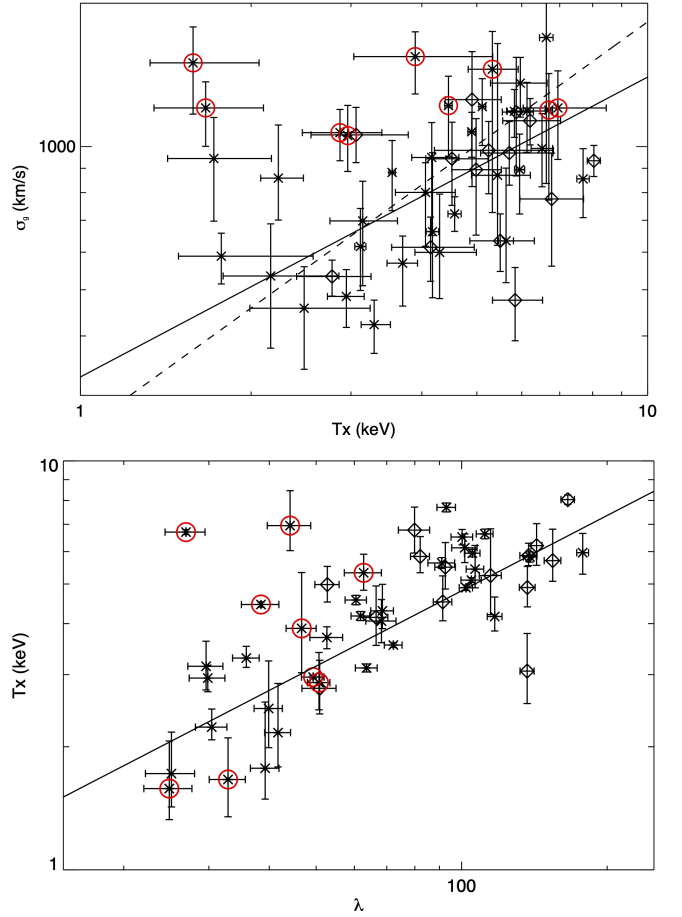
Figure 11. Top: Velocity dispersion-temperature relation compared to the relations from Farahi et al. (2018) (solid line) and Wilson et al. (2016) (dashed line) for X-ray selected samples observed with XMM. Bottom: Temperature-richness relation compared to the relation from Farahi et al. (2019) for DES Y1 redMaPPer clusters (solid line). In both plots, XMM temperature measurements are plotted with asterisks and Chandra measurements with diamonds. Chandra temperatures have been adjusted to the XMM scale using the relation from Rykoff et al. (2016). The T_X - \lambda relation from Farahi et al. (2019) has likewise been adjusted to the XMM temperature scale. Velocity dispersion outlier clusters are circled in red.
