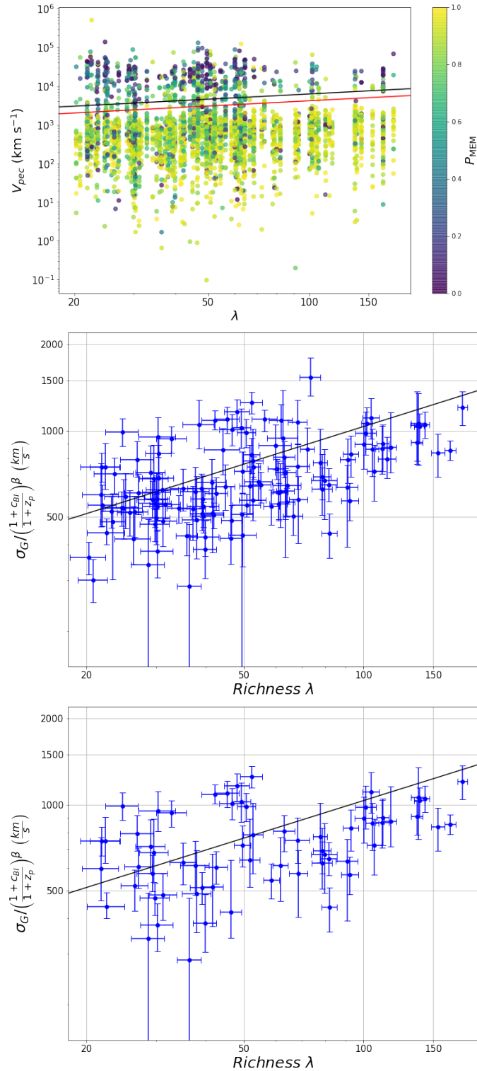
Figure A7. Top: Equivalent to Figure 1 but showing a modified velocity offset limit in red. This modified limit changes the 3000 \text{ km s}^{-1} in Equation 2 to 2000 \text{ km s}^{-1} . Middle: Equivalent of Figure 3 for members selected using the modified velocity offset limit. Bottom: Equivalent of Figure 4 for members selected using the modified velocity offset limit.
