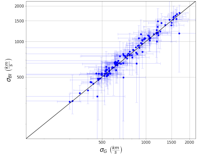
Figure 2. Comparison of the velocity dispersion estimators \sigma_G and \sigma_{BI} . The black line shows a one to one relation between. It is apparent that these estimators agree well for the majority of the clusters in our sample.
