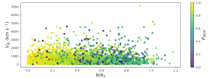
Figure A6. Member galaxy peculiar velocity shown against R/R_\lambda with P_{\text{MEM}} on the color axis. The dependence of P_{\text{MEM}} on R/R_\lambda is apparent with high P_{\text{MEM}} galaxies on average having low R/R_\lambda .
