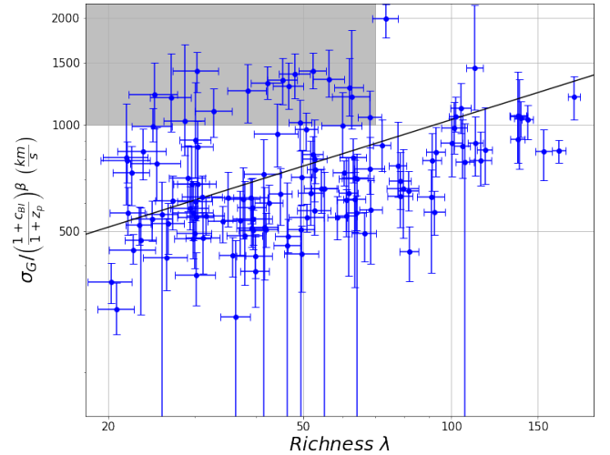
Figure 3. Velocity dispersion-richness relation for velocity dispersion estimated with the gapper method. The black line shows the \lambda adjusted \sigma_{v-\lambda} trend line found by Rozo et al. (2015) , with the richness adjusted for the difference between SDSS and DES Y3 using equation 12. The redshift dependence is accounted for by adjusting the cluster velocity dispersion based on the cluster redshift ( z_p = 0.171 , \beta = 0.54 ) following the redshift dependence found in Rozo et al. (2015) . The \sigma_G-\lambda relation shows a bi-modal distribution with a small, but significant fraction of clusters having apparent velocity dispersions that are high for their richnesses; several factors can act to inflate the observed velocity dispersion including projection effects of structure along the line of sight and mergers, while effects like miscentering can act to reduce the observed richness. The grey shaded region outlines the defined region for outlier clusters with \lambda < 70 and \sigma_G > 1000 \text{ km s}^{-1} .
