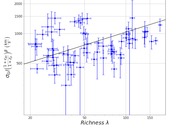
Figure 4. Gapper method velocity dispersions versus cluster richness limited to clusters in the volume-limited redMaPPer catalog with 0.20 < z < 0.65 . The black line is the \lambda adjusted \sigma_G - \lambda trend line found by Rozo et al. (2015) . The redshift dependence is accounted for by adjusting the cluster velocity dispersion based on the cluster redshift ( z_p = 0.171 , \beta = 0.54 ) following the redshift dependence found in Rozo et al. (2015) . The outlier population of low richness, high velocity dispersion clusters persists after volume limiting and redshift limiting the clusters studied.
