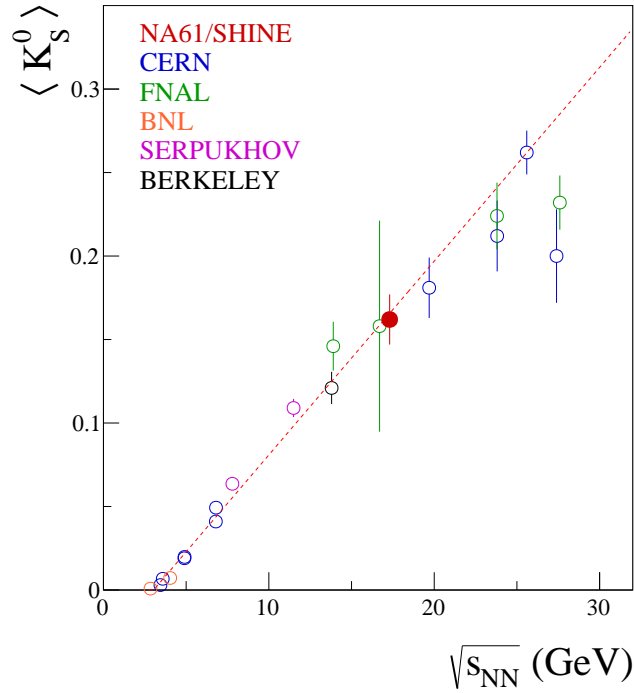
Figure 13: (Color online) Collision energy dependence of mean multiplicity of K_S^0 mesons produced in p+p interactions. The full coloured red circle shows the measurement by NA61/SHINE presented with its systematic uncertainty. The results published by other experiments are presented with open circles coloured in blue (CERN), green (FNAL), orange (BNL), magenta (SERPUKHOV) and black (BERKELEY). The references for the plotted data points are given in the text.
