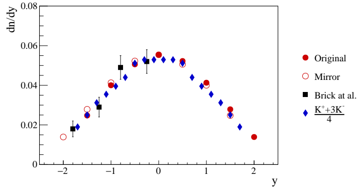
Figure 11: (Color online) Rapidity distribution dn/dy of K_S^0 mesons in inelastic p+p interactions at 158 GeV/c. Full red-coloured circles correspond to the NA61/SHINE results, open circles are mirrored values, black squares represent results from Brick et al. at FNAL [19] and blue full diamonds show results obtained from the formula \frac{1}{4}(N_{K^+} + 3 \cdot N_{K^-}) using charged kaon yields recently measured by NA61/SHINE at the same beam momentum [20].
