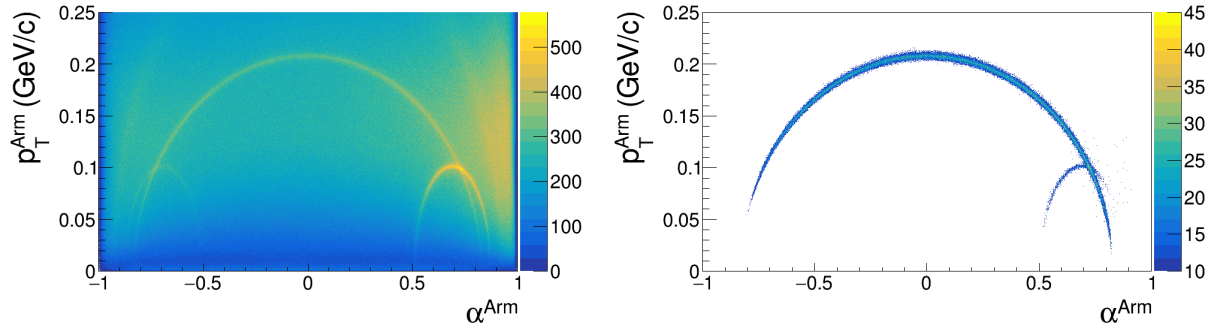
Figure 4: Armenteros-Podolanski plots for V^0 candidates without ( left ) and with all track and topology selection criteria ( right ).
