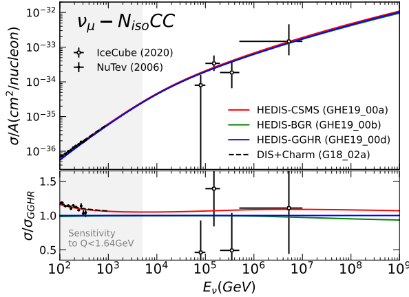
Fig. 10. Predictions of total cross section per nucleon for \nu_\mu CC scattering assuming isoscalar target for three different models implemented in HEDIS: BGR18 [85], CMS11 [93] and GGHR20 [82]. Predictions from G18_02a (assuming DIS and charm production) and NuTeV [95] and IceCube [96] measurements are shown up to E_\nu = 1 TeV for comparison. Grey area shows the region where low-momentum contributions ( Q < 1.64 GeV) are relevant.
