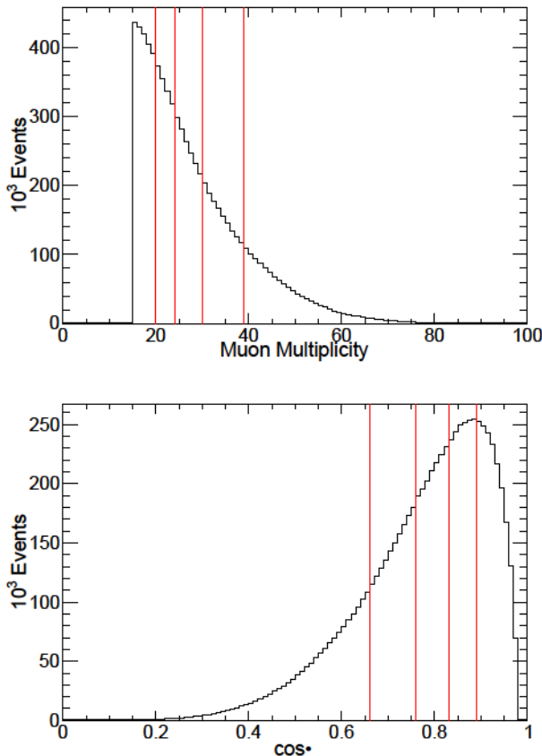
FIG. 2. Reconstructed quantities for all showers used in the analysis. Top: The muon multiplicity of air showers recorded in the NOvA detector. Only multiplicities of 15 or more are considered. Bottom: The cosine of the zenith angles of air showers. Showers with vertical zenith angle or horizontal showers from the east/west are removed from the analysis due to reconstruction challenges which suppresses the showers at high \cos\theta . In both panels, the vertical lines denote the bin boundaries used in section V.
