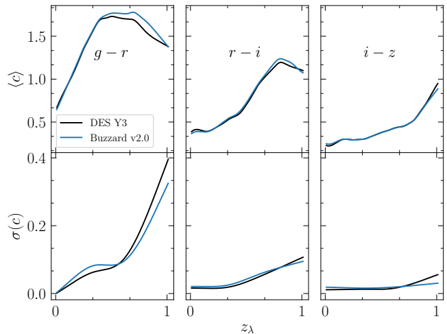
FIG. 2. Comparison of red-sequence colors between Buzzard and DES Y3 as measured by redMaPPer . (Top) Mean red-sequence color as a function of redshift for the DES Y3 data (black) compared to the Buzzard simulations (blue). The largest differences occur at high redshift in g-r , where the mean color is poorly constrained in the data. (Bottom) Scatter in red-sequence colors as a function of redshift for the DES Y3 data and Buzzard .
