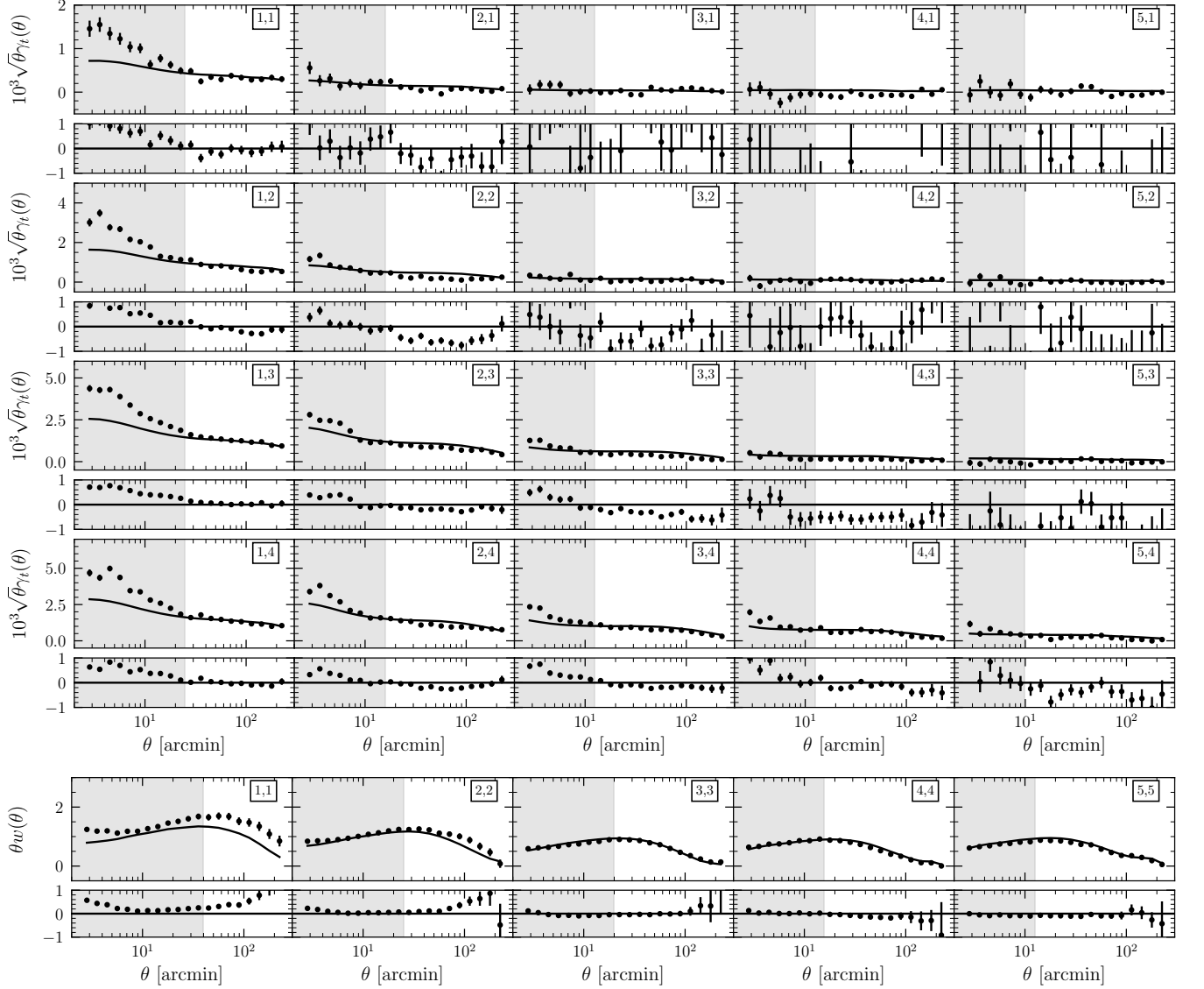
FIG. 4. Comparison of \gamma_t(\theta) and w(\theta) between Buzzard (lines) and the measurements from the Y3 data using the redMaGiC lens sample (points), with error bars given by the fiducial Y3 covariance matrix. Shaded regions indicate the angular scale cuts applied in the fiducial 3 \times 2 -point analysis. Rows alternate between showing the measured signals and the fractional difference between data and simulations. Numbers in each panel label the bin combinations shown, with the numbers in the \gamma_t(\theta) panels representing the lens-source bin pair, and numbers in w(\theta) panels denoting the lens bins alone. The intent of this comparison is to gauge how well the galaxy clustering and lensing properties in Buzzard match those observed in the data, with the caveat that disagreement may arise due to differences in cosmology, and source and lens galaxy redshift distributions. Agreement in w(\theta) is generally better than for \gamma_t(\theta) especially for the 2nd–5th lens bins, which may be a result of slightly different source redshift distributions between the simulations and data, especially where there is significant overlap between source and lens redshift distributions. We also observe a marked deficit of power on small scales in \gamma_t(\theta) for the first lens bin at smaller scales than those used in the analysis, part of which is likely due to resolution effects in Buzzard . The excellent match between \gamma_t(\theta) on larger scales in the first lens bin is interesting in light of the large discrepancy in the amplitude of w(\theta) between the DES Y3 data and Buzzard for this lens bin. DES Collaboration [21] demonstrates that under the assumption of \Lambda CDM the redMaGiC w(\theta) and \gamma_t(\theta) imply bias values that differ by 12%, so this may play some role in the discrepancies seen between the Buzzard and DES Y3 w(\theta) measurements in the first lens bin.
