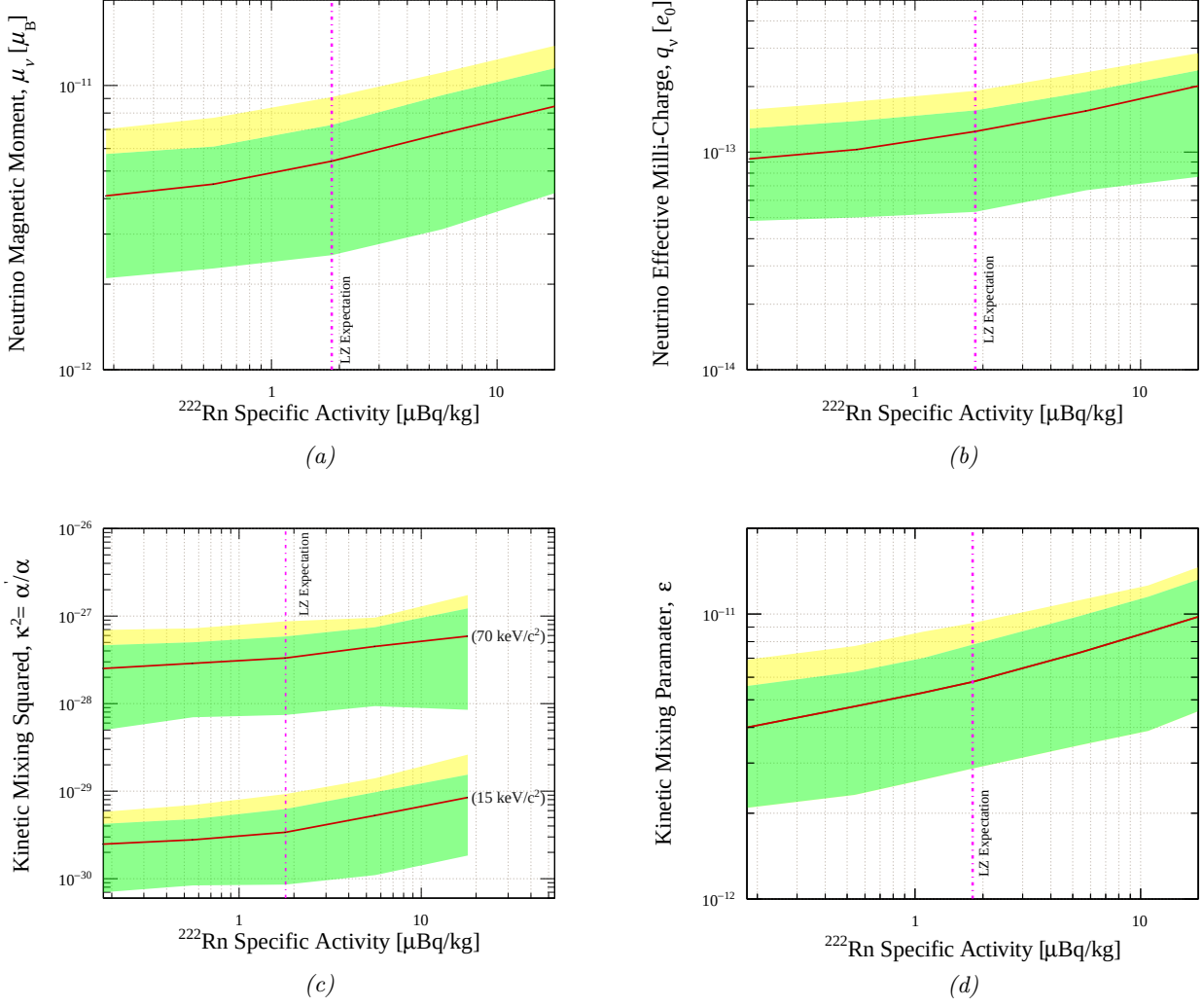
FIG. 5: Variation of 90% C.L. exclusion sensitivity to (a) solar neutrino magnetic moment, (b) solar neutrino effective millicharge, (c) kinetic mixing squared, \kappa^2 for 15 and 70 keV/c 2 hidden photons and (d) mirror dark matter kinetic mixing for local mirror electron temperature 0.3 keV. \pm 1\sigma (green) and +2\sigma (yellow) bands are also shown.
