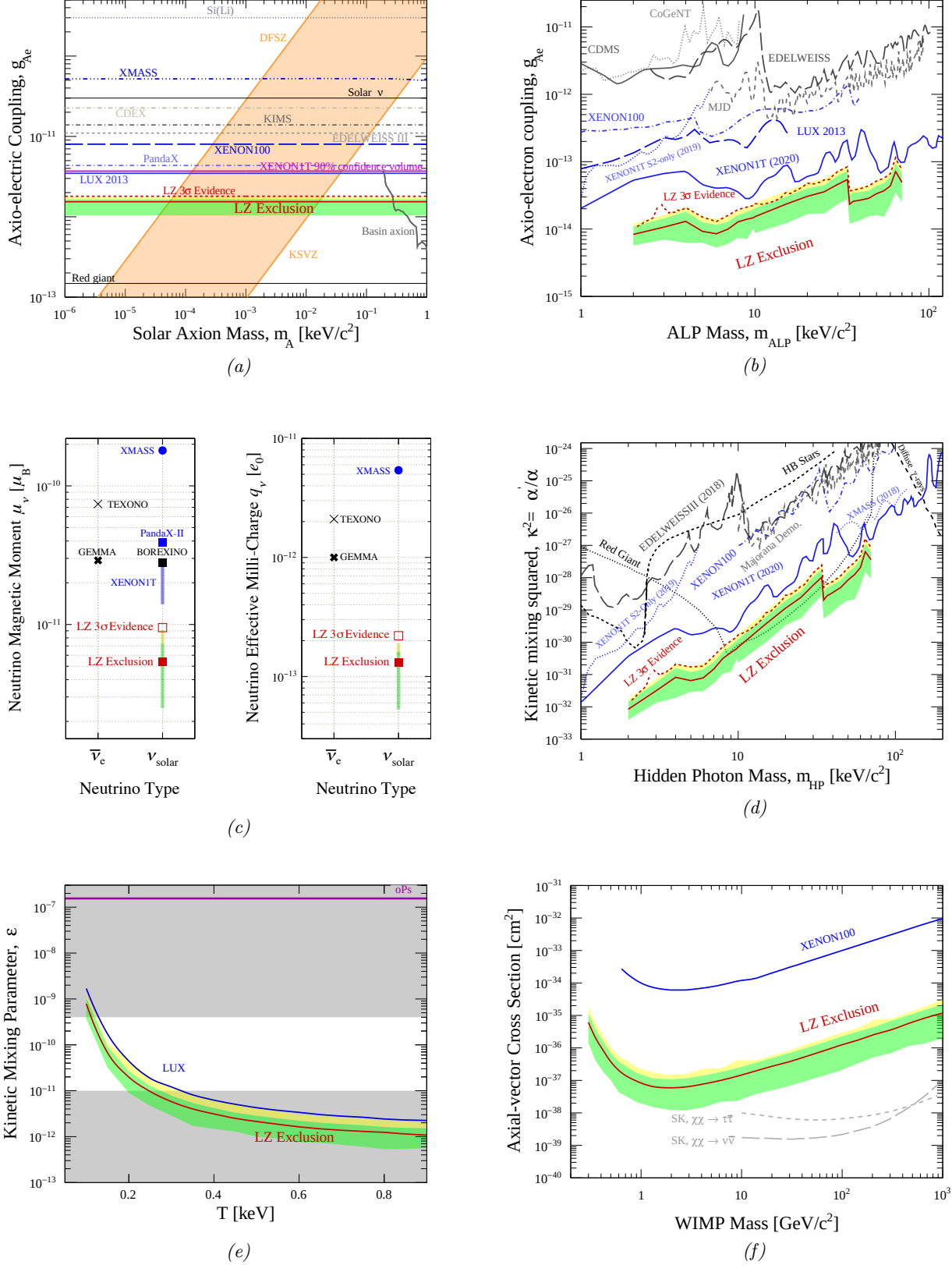
FIG. 4: 90% C.L. exclusion sensitivity to (a) axio-electric coupling for solar axions, (b) axio-electric coupling for galactic ALPs, (c) electromagnetic neutrino couplings \mu_\nu and q_\nu , (d) kinetic mixing squared, \kappa^2 for hidden photons, (e) mirror dark matter kinetic mixing, and (f) axial-vector cross-section for leptophilic dark matter. \pm 1\sigma (green) and +2\sigma (yellow) bands are also shown. For selected models, sensitivity to 3\sigma evidence is also shown. Results from other experiments and astrophysical constraints are referenced in the text.
