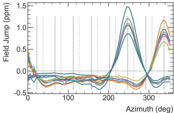
FIG. 27: The field step size as a function of azimuth for all field jumps during the Run-1a dataset. The vertical gray lines indicate the positions of the radial stops (solid: top, dashed: bottom).
