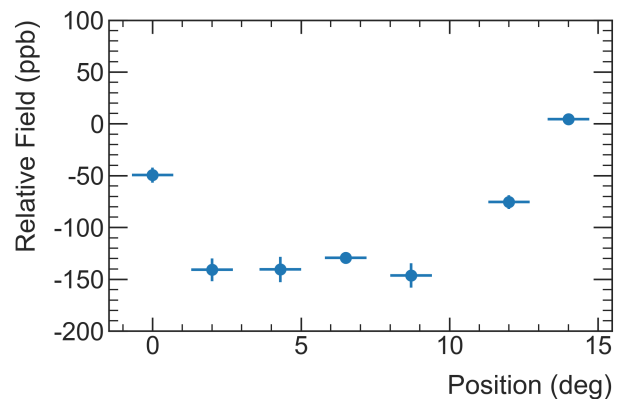
FIG. 24: The relative field shift caused by the transient as a function of the azimuthal position with respect to the center ( \phi = 0 deg) of a long ESQ. The transient is strongest in the center of the ESQ section, falling off toward the edges.
