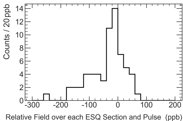
FIG. 25: The distribution of the observed ESQ transient effect over all stations and sections. The full width of the distribution is used as the uncertainty ( \pm 178 ppb) in the ESQ region and scaled down by the geometrical coverage factor of the ESQ in the storage ring (0.433).
