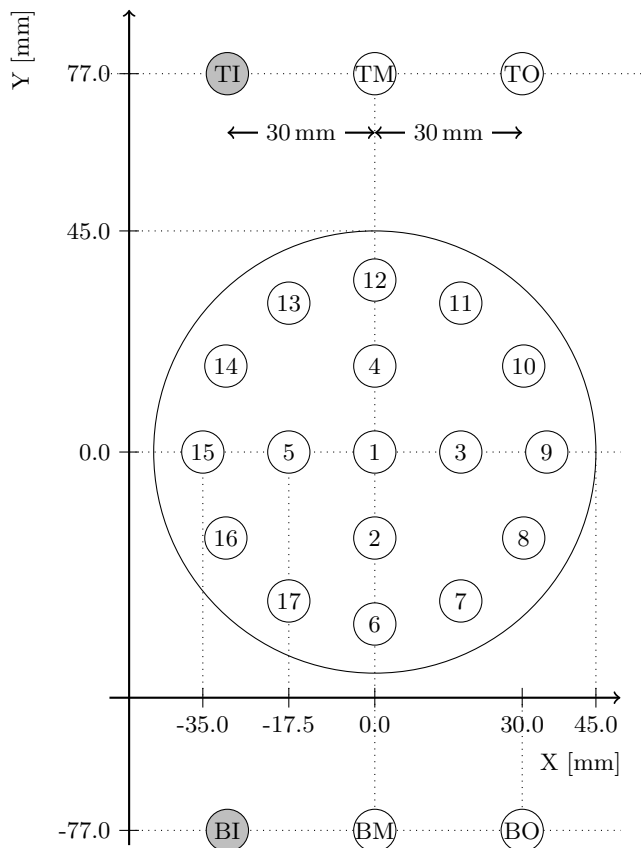
FIG. 6: The layout of the 17 probes in the trolley. Positive x is towards higher radius. The fixed probe locations on the top (T) and bottom (B) of the storage ring are shown as well. For the fixed probes, the six-probe stations have probes in the inner (I), middle (M), and outer (O) positions. In the four-probe stations, only the middle and outer probes are present.
