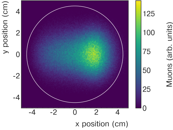
FIG. 19: A typical example of the muon distribution measured by the trackers after integrating for several hours. This distribution is used to weight the field map.
