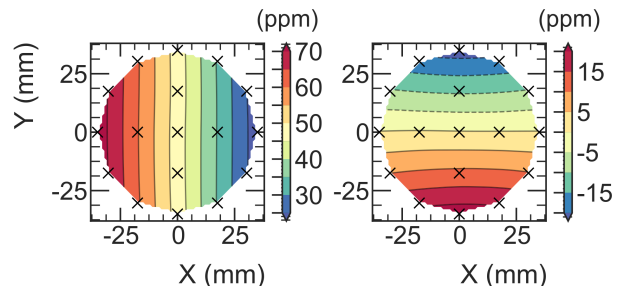
FIG. 11: \Delta\omega_{j,x}^{\text{tr}} (left) and \Delta\omega_{j,y}^{\text{tr}} (right) measured by the trolley. The graphs were fitted to a two-dimensional polynomial to extract the large imposed field gradient. These gradients are used to uniquely identify a probe’s location in the xy plane.
