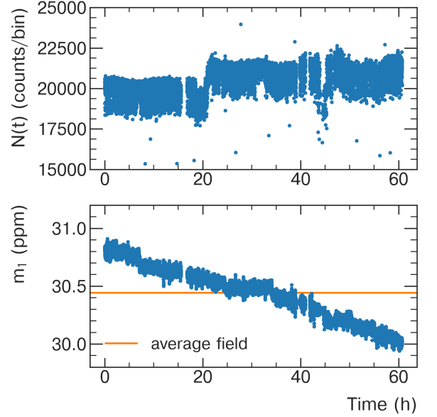
FIG. 20: The number of muons integrated per bin over a typical trolley run pair and the azimuthally averaged dipole field over the same time. The number of integrated muons, represented by the number of observed decay positrons, is used to weight the field when evaluating the integral over time in Eq. (26).
