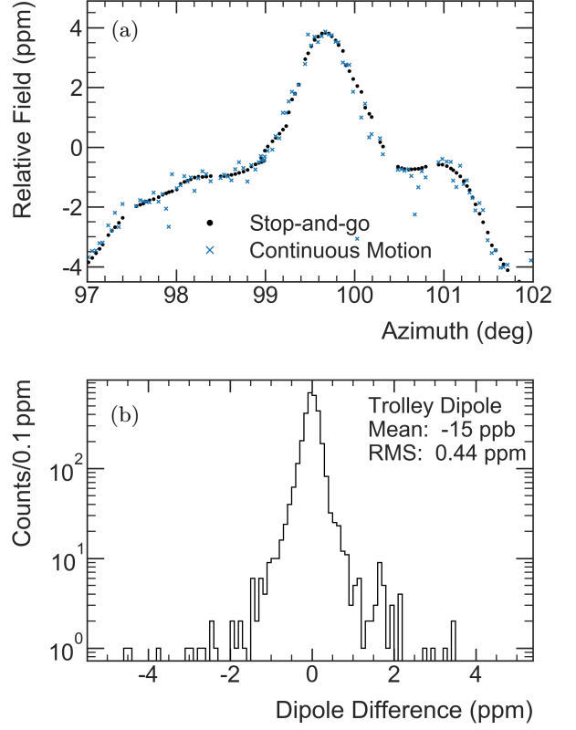
FIG. 14: The difference between moving and static trolley measurements. (a) Comparison of the frequencies measured in a selected azimuthal region for the normal trolley motion and the stop-and-go operation. (b) The distribution of the dipole differences between motion and static measurements over the full ring.
