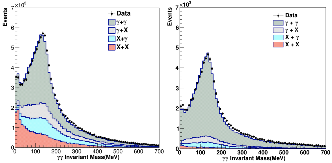
(a) Baseline reconstruction of the neutral pion (b) Neutral pion reconstruction with ML prediction
