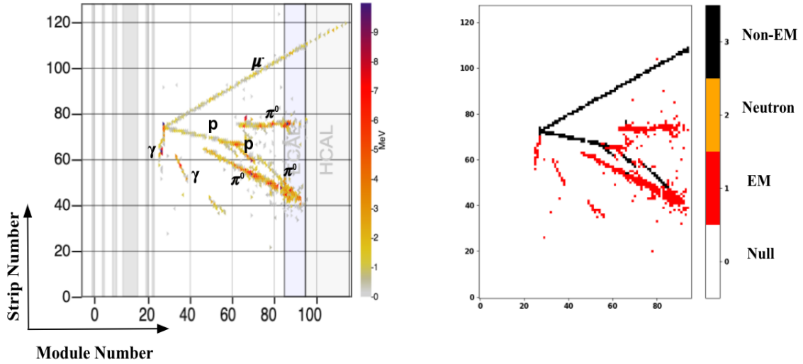
Figure 5: Left: A visualization of a simulated DIS neutral pion production event using the web-based tool Arachne[31] tool. Right: a semantically-segmented image of the same event. For the medium energy dataset, many events have \gamma s with trajectories very close to each other, thereby increasing the difficulty of distinguishing \gamma pairs. The higher the \pi^0 energy is, the smaller the opening angle is, raising the complexity of distinguishing the \gamma s' pair. A common approach when faced with this type of issue is by rejecting these mis-reconstructed events, which reduces the efficiency of \pi^0 reconstruction.
