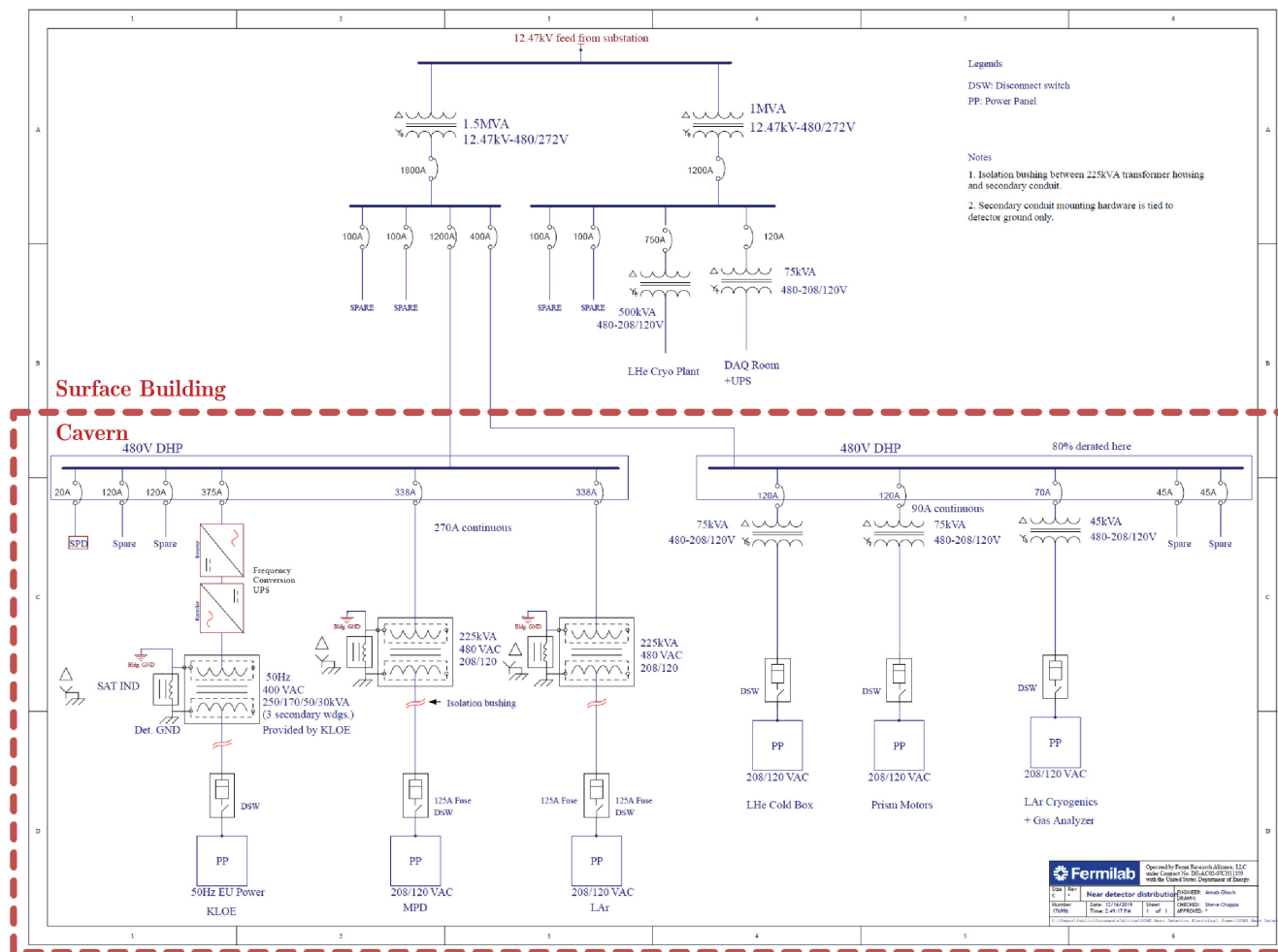
Figure 8.19: DUNE ND detector power distribution diagram.
