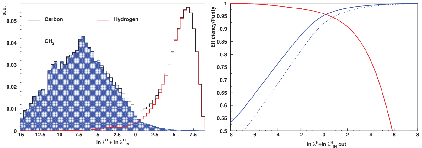
Figure 5.26: Left plot: Example of kinematic identification of \nu(\bar{\nu})H interactions for the \nu_{\mu}p \rightarrow \mu^- p \pi^+ CC topologies reconstructed in the STT. The distributions of the logarithm of the likelihood ratio H/C for the H signal, the C background, and the CH 2 plastic (sum) are shown. Right plot: Efficiency (red color) and purity (blue color) as a function of the kinematic cut for the exclusive processes \nu_{\mu}p \rightarrow \mu^- p \pi^+ (solid lines) and \bar{\nu}_{\mu}p \rightarrow \mu^+ p \pi^- (dashed-dotted lines) on H [51].
