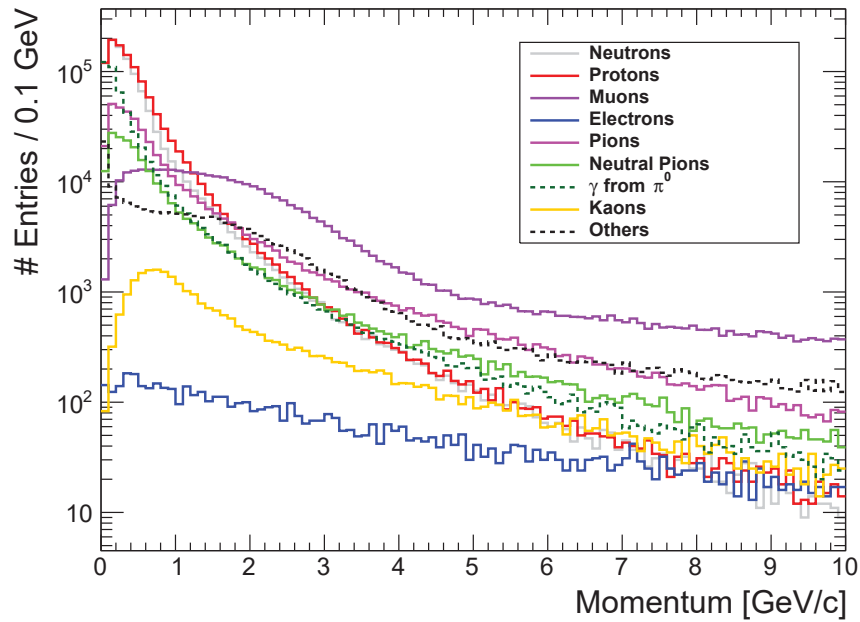
Figure 3.34: GENIE prediction of momentum spectra for particles resulting from neutrino interactions in ND-GAR, shown in log scale on the vertical axis.
