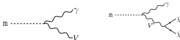
Figure 7.1: Production of fermionic DM via two-body neutral pseudoscalar meson decay \mathbf{m} \rightarrow \gamma V , when M_V < m_{\mathbf{m}} (left) or via three-body decay with off-shell V \mathbf{m} \rightarrow \gamma \chi \bar{\chi} (right).
