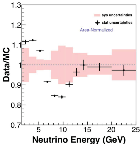
Figure 1.2: Ratio of the observation to simulation for the reconstructed MINERvA medium-energy NuMI neutrino event spectrum for low energy-transfer events. (This is the updated version of what is shown in [18].)
