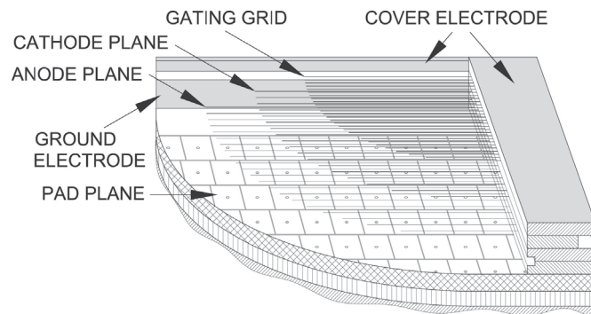
Figure 3.3: Schematic diagram of the ALICE MWPC-based ROC with pad plane readout, from Ref. [97].
