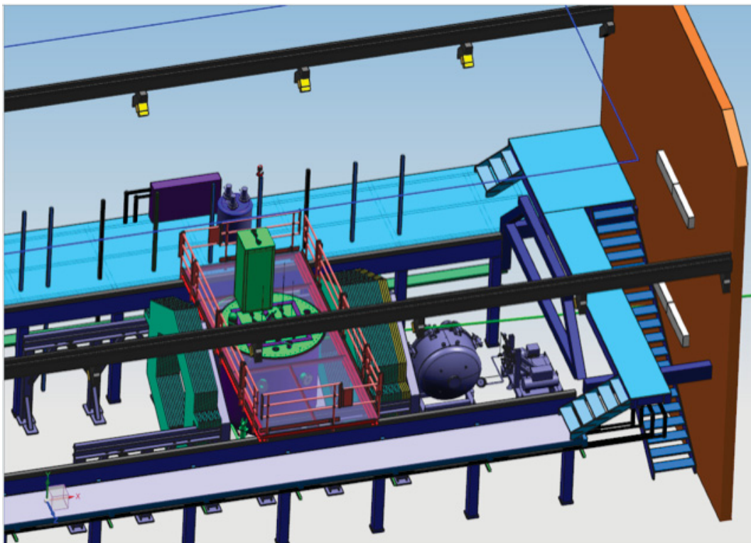
Figure 2.14: A drawing of the ArgonCube demonstrator deployed in the MINOS ND hall at Fermilab, forming ProtoDUNE-ND. One module is shown in the extracted position. The neutrino beam is incident from the left. Sections of MINERvA are shown upstream and downstream of the demonstrator. A prototype of the gas TPC of ND-GAr is also shown at the downstream end.
