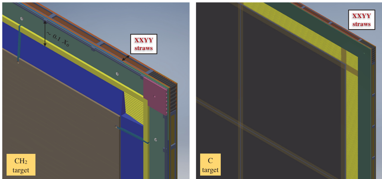
Figure 5.14: Left picture: Detailed 3D engineering CAD model of one STT module equipped with \text{CH}_2 target slab (in brown color) and radiator (in blue color). The average density of the detector can be fine tuned between 0.005 \text{ g/cm}^3 (without target slab and radiator) and 0.18 \text{ g/cm}^3 (configuration in the drawing). Both the target slab and the radiator can be unmounted during data taking by removing four corner screws. Right picture: Engineering CAD model of of one STT module equipped with graphite target (in black color). The tracking part is composed of four straw layers XXYY and is the same as in the \text{CH}_2 module on the left.
