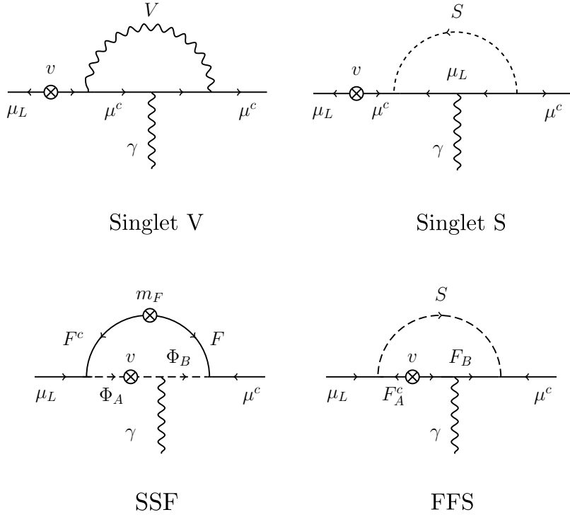
Figure 3: Representative 1-loop contributions to (g - 2)_\mu in the simplified models we consider. Top row: Singlet Scenarios with a SM neutral vector V or scalar S that couple to the muon. Note that the Higgs VEV on the muon line gives both the chirality flip and the EW breaking insertions in these models. Bottom left: EW Scenario of SSF type, with one BSM fermion and two BSM scalars that mix via a Higgs insertion. Bottom right: EW Scenario of FFS type, with one BSM scalar and two BSM fermions that mix via a Higgs insertion.
