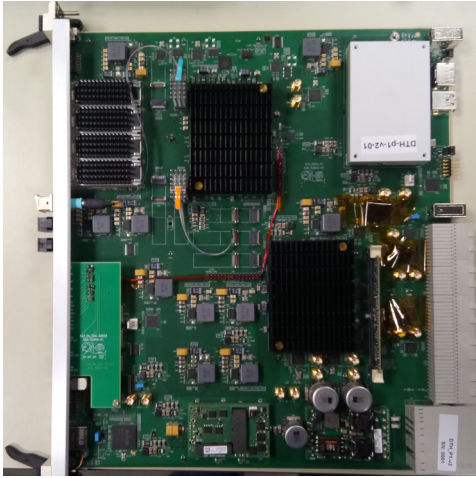
Figure 3. Left: block diagram of the DTH board. Right: DTH P1-v2 board prototype. This prototype uses two KU15P FPGA. The prototype 2 of the board, currently being designed, will use a VU35P FPGA with on-chip HBM.
