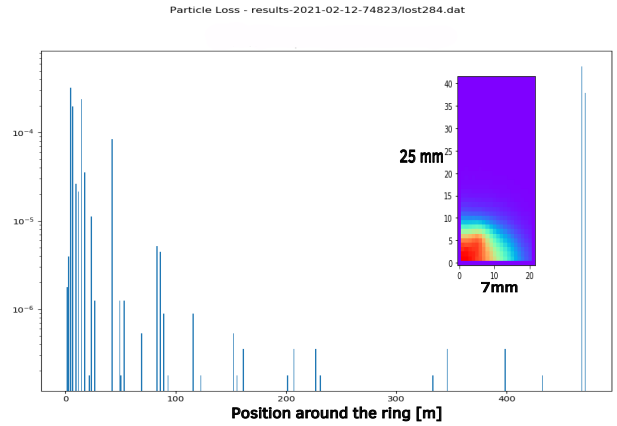
Figure 5: Large angle loss pattern. Losses around 470 m (upstream of the injection point) are likely due to a reduction in available vertical aperture at that location.
