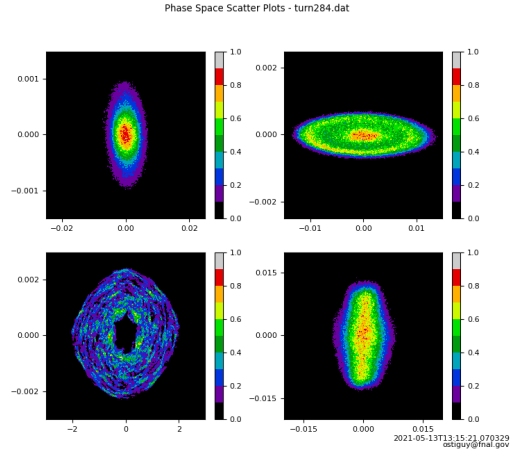
Figure 4: Beam distribution at the end of the injection. Top: left x-x' , right: y-y' , Bottom: left dp/p-\phi right: x-y . Both transverse phase ellipses are now filled. The center region of the longitudinal ellipse remains hollow.
