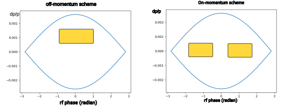
Figure 2: Left: off-momentum scheme. Right: on-momentum scheme. Linac bunches are accepted only when they fall within the shaded areas.
