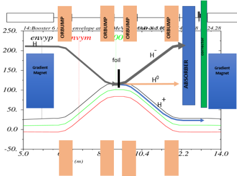
Figure 1: Schematic of the PIP-II Booster injection region. The H^- ions are injected vertically. The vertical orbit is deflected using four orbumps magnets and the beam hits the foil at a fixed location near the inner lower corner of the foil.
