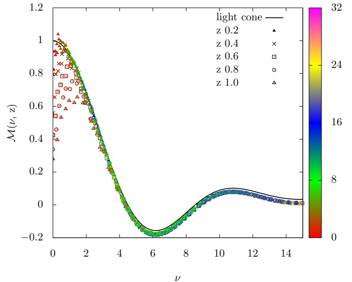
FIG. 26 The proton unpolarized u quark pseudo distribution normalized to one is shown for different values of quark field separation z in \text{GeV}^{-1} . P_3 is tagged from 0 to 32 \text{GeV}^{-1} according to color. We see that at small Ioffe time \nu , for lower values of P_3 , the pseudo pdf deviates substantially from the expected Ioffe time behavior of the light cone parton distribution. The momentum space GPD used to evaluate the curves in this figure was obtained using the reggeized diquark model from Ref. (Gonzalez-Hernandez et al. , 2013).
