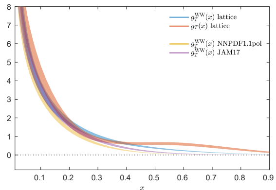
FIG. 9 Comparison of g_T(x) from lattice (red band) with its WW approximations: lattice-extracted g_T^{\text{WW}} (blue band) and calculated from global fits (NNPDF1.1pol (Nocera et al. , 2014) orange band, JAM17 (Ethier et al. , 2017) purple band). The proton momentum is P_3 = 1.67 GeV.
