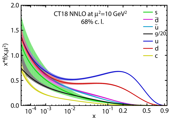
FIG. 2 The CT18 PDFs at \mu^2 = 10 \text{ GeV}^2 for the xu , x\bar{u} , x\bar{d} , xs = x\bar{s} , and xg PDFs. Error bands correspond to the 68% confidence level. Figure from (Kovařík et al. , 2019).
