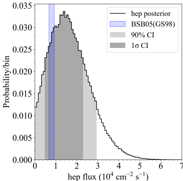
FIG. 4. The posterior distribution for the hep flux, marginalized over all other fit parameters, with the 90% and 1\sigma credible intervals. The BSB05(GS98) standard solar model prediction [7, 8] is also shown for comparison.
