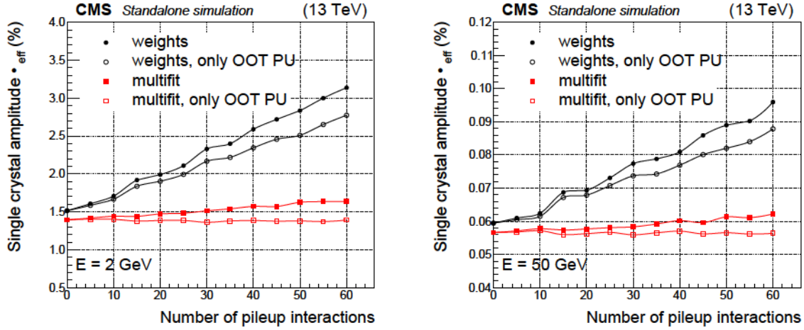
Figure 9: Measured amplitude resolution for two generated energy deposits ( E = 2 \text{ GeV} or E = 50 \text{ GeV} ) in a single ECAL barrel crystal, at \eta = 0 , reconstructed with either the multifit or the weights algorithm. Filled points show the effective resolution expressed as the difference between the reconstructed energy and the true energy, divided by the true energy. Open points show the percent resolution estimated when the true energy is replaced with the sum of the true energy and the in-time pileup energy.
