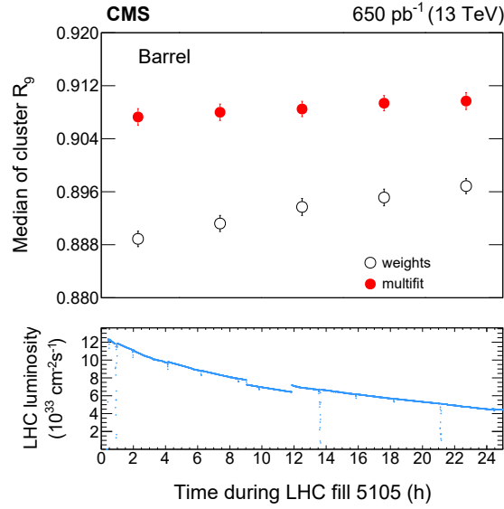
Figure 15: History of the median of the R_9 cluster shape for electrons from Z \rightarrow e e decays during one typical LHC fill in 2016. Hits are reconstructed with either the multifit (filled circles) or the weights algorithm (open circles). Each point represents the median of the distribution for a 5 hour period during the considered LHC fill. Error bars represent the statistical uncertainty on the median. The bottom panel shows the instantaneous luminosity delivered by the LHC as a function of time. The steps in the luminosity occurring about every two hours correspond to changes in the LHC beam crossing angle, which changes the overlap area of the bunches. Larger brief drops could indicate emittance scans during the fill.
