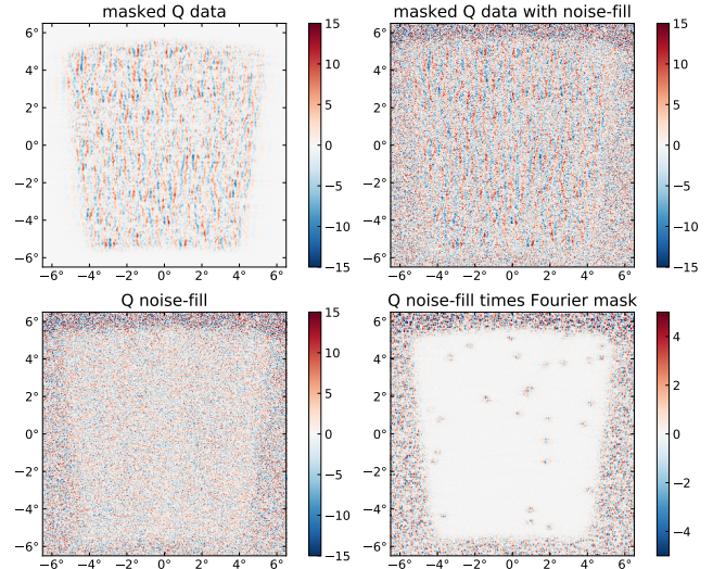
Figure 4. A demonstration of the “noise-fill” procedure described in Section 3.8, which makes it much easier to exactly Wiener filter the data even in the presence of pixel and Fourier space masking and a noise covariance model which is not diagonal in either space. The top-left panel shows 100D-DEEP data with the mask applied, including Fourier and pixel masks. The top-right panel additionally has the noise-fill, \bar{n} , added in; this panel is exactly the data, d , which is used in the posterior in Eq. (8). The bottom-left panel shows just \bar{n} , and the bottom-right panel is \bar{n} multiplied by the Fourier mask. In this last panel, one can see that in the region interior to the mask and in the range of Fourier modes which are not masked by the Fourier mask, no extra noise is added (hence this procedure does not degrade constraints). Here we have plotted just the Q -polarization component; U -polarization behaves qualitatively the same.
