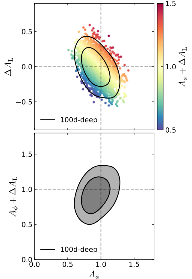
Figure 11. (Top panel) Joint constraints from the 100D-DEEP dataset on the amplitude of the lensing potential, A_\phi^{100 \rightarrow 2000} , and the residual lensing-like power, \Delta A_L . The correlation coefficient between the two is \rho = -0.40(5) , demonstrating only about 9(3)% of the A_\phi^{100 \rightarrow 2000} constraint originates from the power spectrum of the data. (Bottom panel) The same posterior as in the top panel but in terms of the A_L = A_\phi^{100 \rightarrow 2000} + \Delta A_L parameter, which controls the total lensing-like power in the data model. These results demonstrate the unique ability of the Bayesian lensing procedure to infer parameters from an optimal lensing reconstruction and from delensed bandpowers while easily and exactly accounting for correlations between the two.
