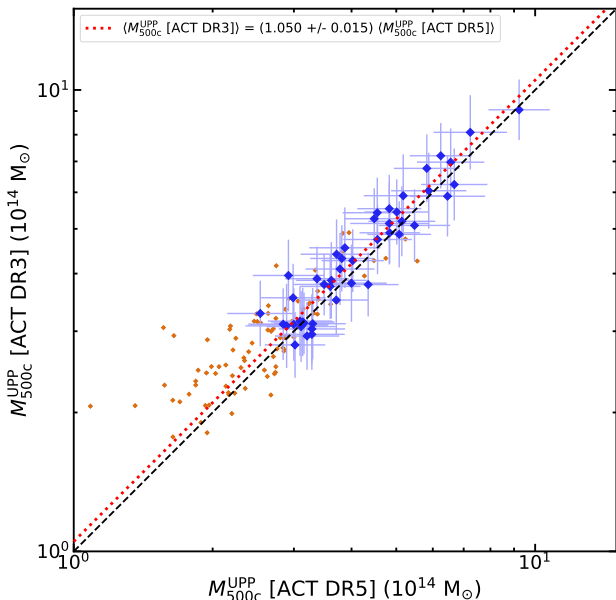
Figure 19. Comparison between ACT DR5 mass estimates (this work, plotted along the horizontal axis) and previous ACT cluster mass estimates as reported in Hilton et al. (2018) (labeled ACT DR3). Both analyses assume the same scaling relation between SZ signal and mass. The large blue points are objects with \text{SNR}_{2.4} > 6 in both samples (for which the unweighted mean ratio is calculated, shown by the dotted red line), while the small orange points (without error bars) show objects below this threshold. The dashed black line shows the 1:1 correlation.
