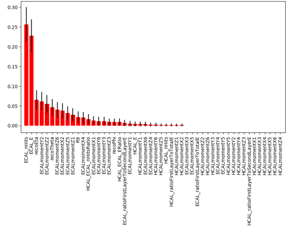
Fig. 24. Feature importances for inputs used in BDT training. Values shown are gini importances [33].
