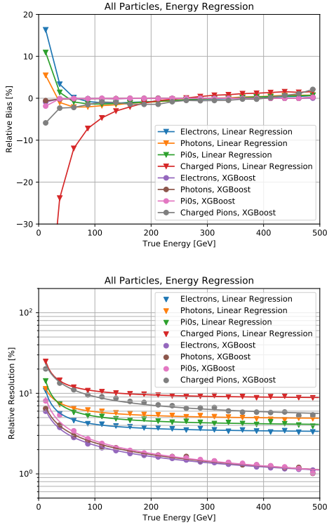
Fig. 27. Bias (top) and resolution (bottom) as a function of true energy for linear regression and XGBoost predictions of particle energy for the different particle types.
