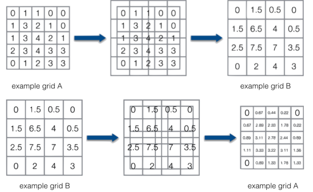
Fig. 16. Example of the resampling procedure used to emulate CLIC data on a different detector geometry (the example shown here is simply a larger grid). First, we extrapolate hit information from one geometry to another (top). Next, we extrapolate back to the original geometry (bottom). This allows us to emulate the rougher granularity of the second geometry, while keeping data array sizes constant and enabling us to use the models we have already developed for the CLIC dataset. Note that some information is lost at the edges.
