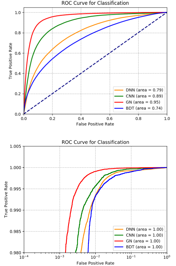
Fig. 13. ROC curve comparisons for \gamma vs. \pi^0 (top) and e vs. \pi^\pm (bottom) classification using different neural network architectures. Samples include particle energies from 10 to 510 GeV, and an inclusive \eta range.
