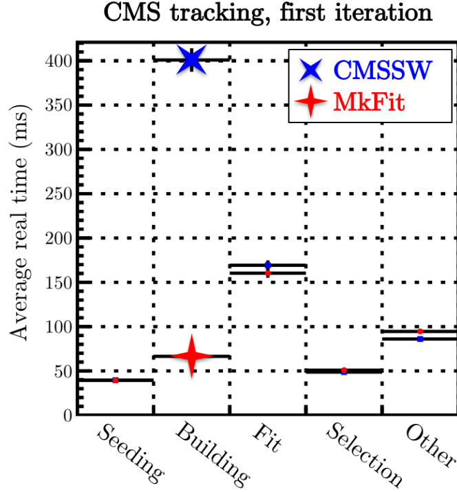
Figure 10. Comparison of the single-thread time to run MkFit as an external within the CMSSW framework (red) to the time to run the standard first iteration of offline tracking in CMSSW (blue). Note that MkFit is used as a replacement for the building step only. MkFit achieves a speedup >6\times over CMSSW in the track building stage. Time measured on SKL-SP using t\bar{t} events with \langle\text{PU}\rangle=50 and CMSSW version 10_4_0_patch1.
