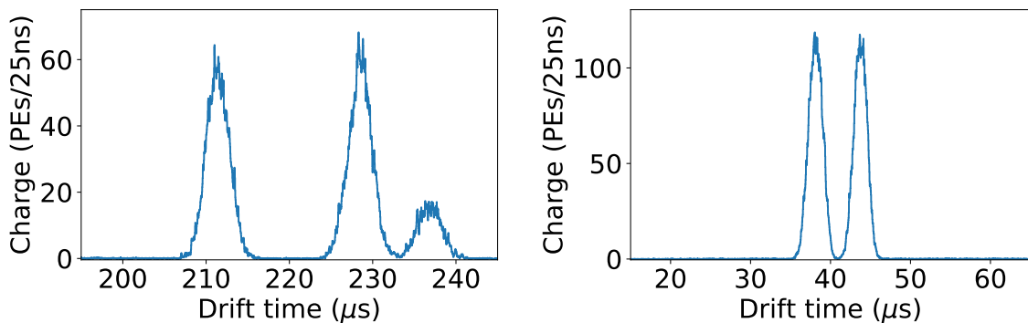
Figure 12. Examples of PMT waveforms of simulated 2\nu ECEC signal events that are incorrectly identified by NEXT standard reconstruction algorithms. Left panel: event with three separate energy deposits, reconstructed as having two S_2 signals at times 211 and 228 \mu\text{s} , respectively. Right panel: event with two separate energy deposits, reconstructed as having one S_2 signal at time 38 \mu\text{s} .
