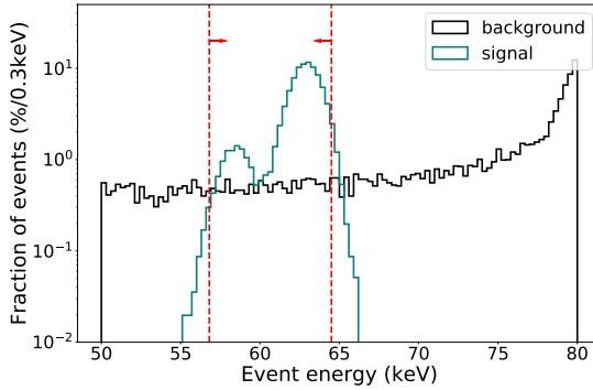
Figure 8. Event energy E_{\text{evt}} signal and background distribution after fiducial selection, with optimal E_{\text{evt}} cut positions (red lines).
