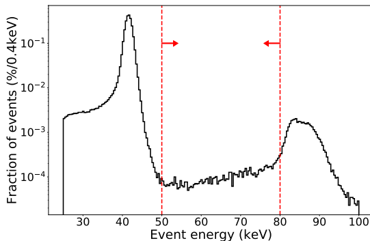
Figure 5. Event energy spectrum of fully reconstructed low-energy triggers from a 26.6 h low-background run of NEXT-White. Red lines indicate the broad energy window for the ^{83\text{m}}\text{Kr} veto.
