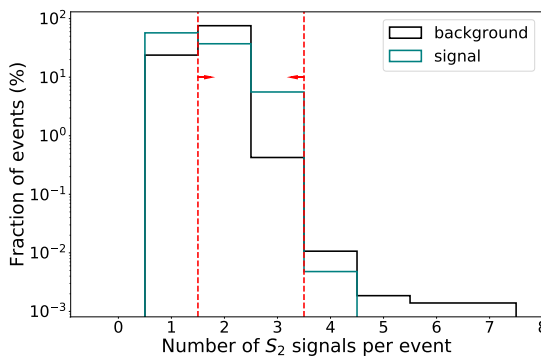
Figure 6. S_2 multiplicity per event for signal and background events after the ^{83\text{m}}\text{Kr} veto. Red lines indicate the limits of the range of accepted values.
