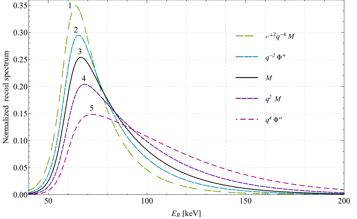
FIG. 1. Expected recoil-energy spectra of argon nuclei in DarkSide-50 from the interaction of 100 MeV/c 2 WIMPs with the SHM velocity distribution for five different EFT operators. Spectra include the acceptance of the detector and are arbitrary normalized. Curve labeled (3) shows the standard spectrum corresponding to the SI operator, i.e., the form factor M in the adopted notation. The other four curves correspond to (1) the nuclear response function M times the factor v^{\perp 2} q^{-4} , (2) \Phi'' times q^{-2} , (4) M times the factor q^2 , and (5) \Phi'' times q^4 .
