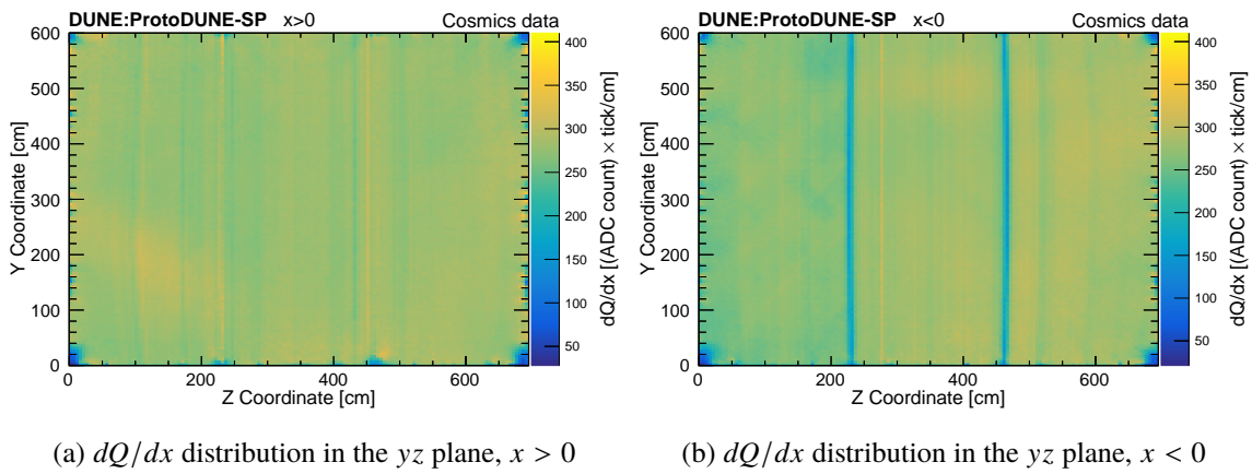
Figure 55: dQ/dx distributions for ProtoDUNE-SP Run 5770 in the yz plane, for x > 0 (a), x < 0 (b), using cosmic-ray cathode-crossing muons. A sample of 99689 throughgoing cosmic ray muon tracks was used in making the plots, which constitutes 23.2% of the total number of cathode-crossing tracks in Run 5770.
