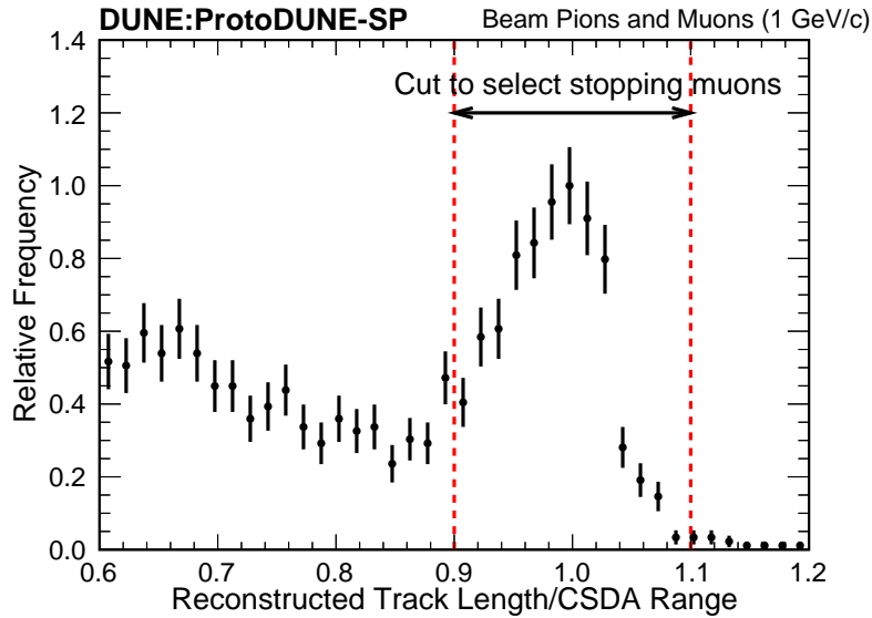
Figure 60: The ratio of track length (SCE corrected) and continuous-slown-down-approximation (CSDA) length for data candidates under the assumption the particle is a muon. The cut to select the stopping muons is indicated. The histogram is normalized such that the maximum frequency is one.
