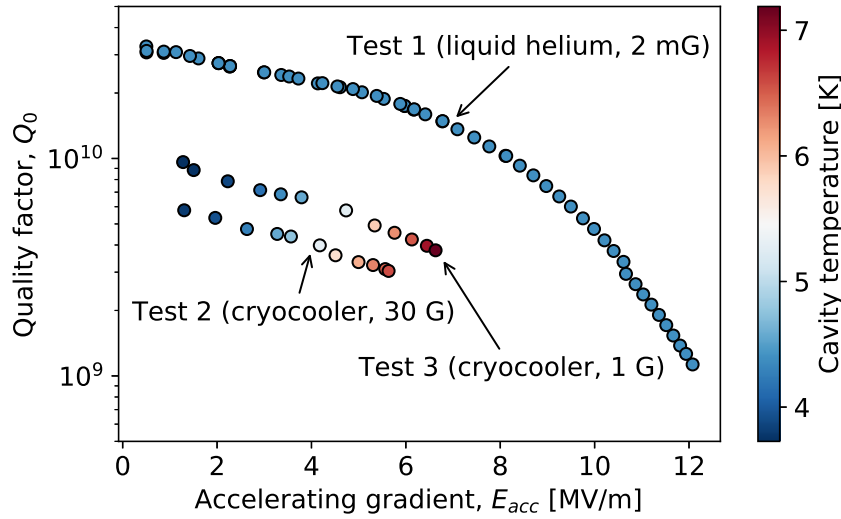
Figure 2. Cavity quality factor, Q_0 vs. accelerating gradient, E_{acc} measured on a single cell, Nb 3 Sn coated, 650 MHz niobium SRF cavity. The data uncertainty is <10%. Test 1 used a helium bath cooled cavity at 4.4 K, in Fermilab Vertical Test Stand with background magnetic field of 2 mG. In Tests 2 and 3, the cavity was conduction-cooled with a 2 W @ 4.2 K pulse tube cryocooler. The improvement in Test 3 resulted from the reduction of magnetic field around the cavity when magnetic disc springs (residual ~30 G) were replaced with cleaner disc springs (residual <1 G).
