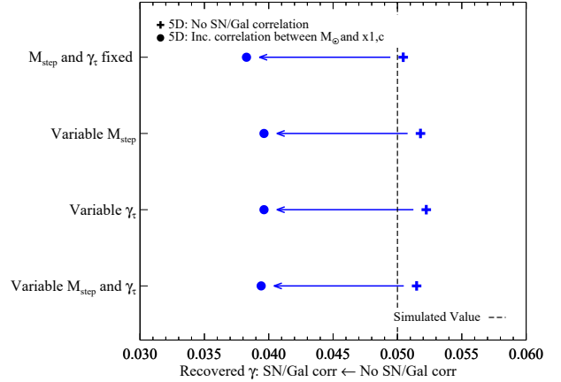
Figure 13. Simulation Output: The best-fit value of \gamma_{\text{fit}} for our simulated DES-SN samples considering different systematic uncertainties when assuming a 5D \mu_{\text{bias}} correction. For each entry, the right-hand value (plotted as a plus symbol) indicates the value when our simulated sample does not contain a correlation between M_{\text{stellar}} and (x_1, c) , while the left-hand entry (plotted as a filled circle) is the result when a correlation is enforced using the prescription described in §5.2.2. The simulated value of \gamma_{\text{sim}} = 0.05 is shown as dashed vertical line. Entries are for our fiducial HOSTLIB, derived from DES-SV data, matched to the mass distribution. Four results with differing assumptions about the mass step parameterisation are shown. In all cases, \gamma_{\text{fit}} is reduced by \sim 0.10 mag when correlations between M_{\text{stellar}} and x_1, c are included. As shown in Table 7 and Table 8, using alternative galaxy catalogues and weighting schemes results in consistent results.
