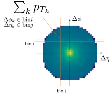
Figure 3. Illustration of a jet image used as the input data format.
