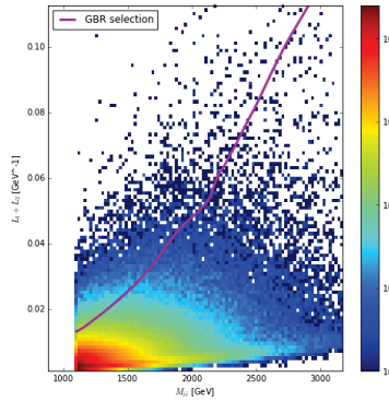
Figure 8. Quantile regression for loss threshold identification.
