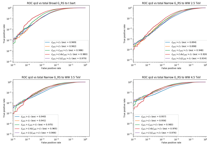
Figure 5. ROC curves for G_{RS} \rightarrow t\bar{t} (top left), G_{RS} \rightarrow WW 2.5 TeV (top right), G_{RS} \rightarrow WW 3.5 TeV (bottom left) and G_{RS} \rightarrow WW 4.5 TeV (bottom right) with different loss combination strategies (distinct lines in each plot)
