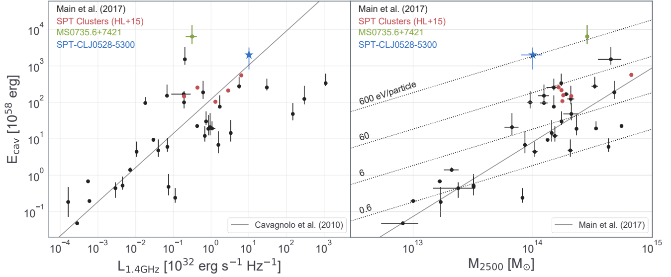
Figure 4. The scaling relations between cavity/outburst energy ( E_{cav} = 4pV_{tot} ) vs total radio luminosity ( L_{1.4\text{GHz}} ) and cluster mass ( M_{2500} ), from Hlavacek-Larrondo et al. (2015, median z \sim 0.6 ) and Main et al. (2017, median z \sim 0.06 ). SPT0528 and MS0735 are plotted here for reference. While we measure an extreme cavity energy for SPT0528, we see that it is entirely consistent with that predicted by its radio luminosity. Solid black lines in both panels represent the best-fit scaling relations among respective quantities from Cavagnolo et al. (2010) and Main et al. (2017).
