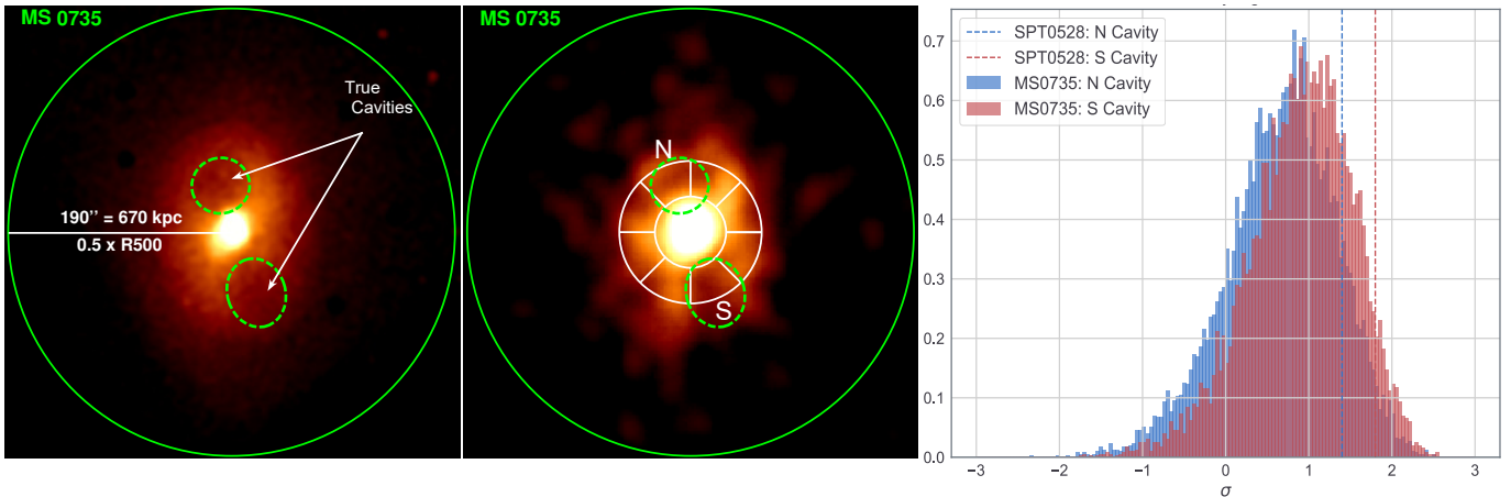
Figure 3. Left: Chandra image of MS0735, the most powerful AGN outburst known (e.g. Rafferty et al. 2006; McNamara et al. 2009). Center: MS0735 downsampled to the same depth ( \sim 1400 counts), energy range (0.5–4 keV), redshift ( z=0.768 ) and self-similar scale ( r_{\text{pixel}}/R_{500} = \text{constant} ) as SPT0528. We calculate the significance of the downsampled cavities by measuring the flux in each of the eight annular wedges illustrated here, subtracting from the average flux across all eight sectors, then dividing by the scatter. Right: The significance distribution of the downsampled cavities in MS0735, calculated over 10,000 realizations. Dashed vertical lines indicate the significance of the cavities in SPT0528 calculated in the same way, demonstrating that the cavities in SPT0528 look similar to what a comparably powerful outburst as in MS0735 would look like at the same depth and redshift.
