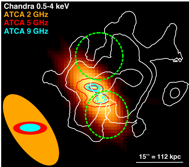
Figure 2. ATCA 2 GHz radio image of SPT0528 with X-ray contours overlaid in white. The 5 GHz ATCA data are represented by red contours at 0.4, 1.7, and 3.1 mJy beam -1 , while the 9 GHz data are represented by cyan contours at 0.5, 0.7, 1.0, and 1.3 mJy beam -1 . The dashed green ellipsoidal regions outline the X-ray cavities as before. The radio source is coincident with the ICM centroid, and is elongated in the direction of the X-ray cavities. The ATCA beam sizes are shown in the bottom-left corner.
