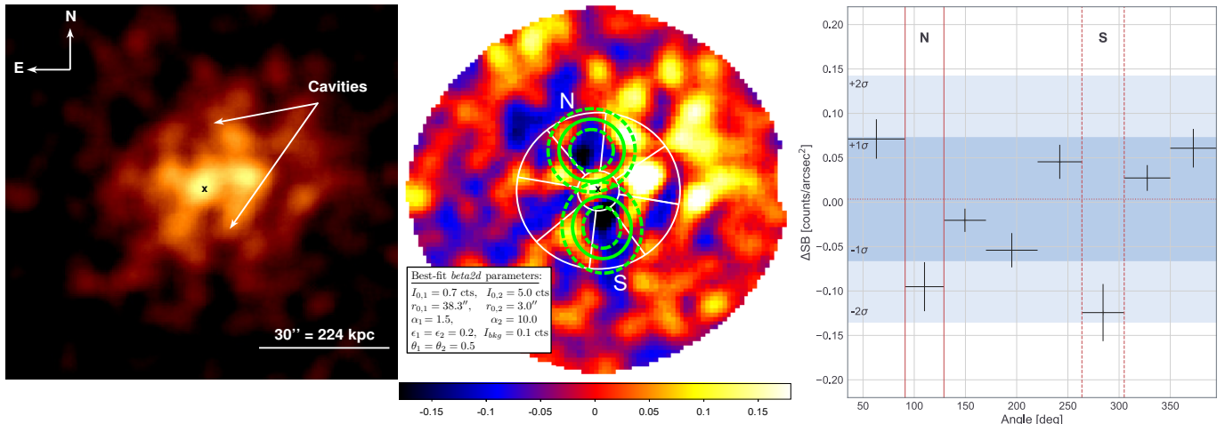
Figure 1. Left: stacked, cleaned 0.5–4 keV Chandra counts image of SPT0528, and center: double-beta model-subtracted residual image with best-fit parameters, both on the same spatial scale. The ‘x’ marks the location of the large-scale ICM centroid. The counts image has been smoothed with a 10-pixel radius Gaussian kernel, while the residual image was first binned by 2 \times 2 -pixels then smoothed with a 5-pixel Gaussian kernel. Solid and dashed ellipsoidal regions outline the detected cavities and their estimated size uncertainty. White annular wedges illustrate where we measured surface brightness in the unsmoothed residual map as a function of azimuthal angle to determine the significance of the cavities, shown in the right panel. The two cavities are detected at 1.4\sigma and 1.8\sigma below the median.
