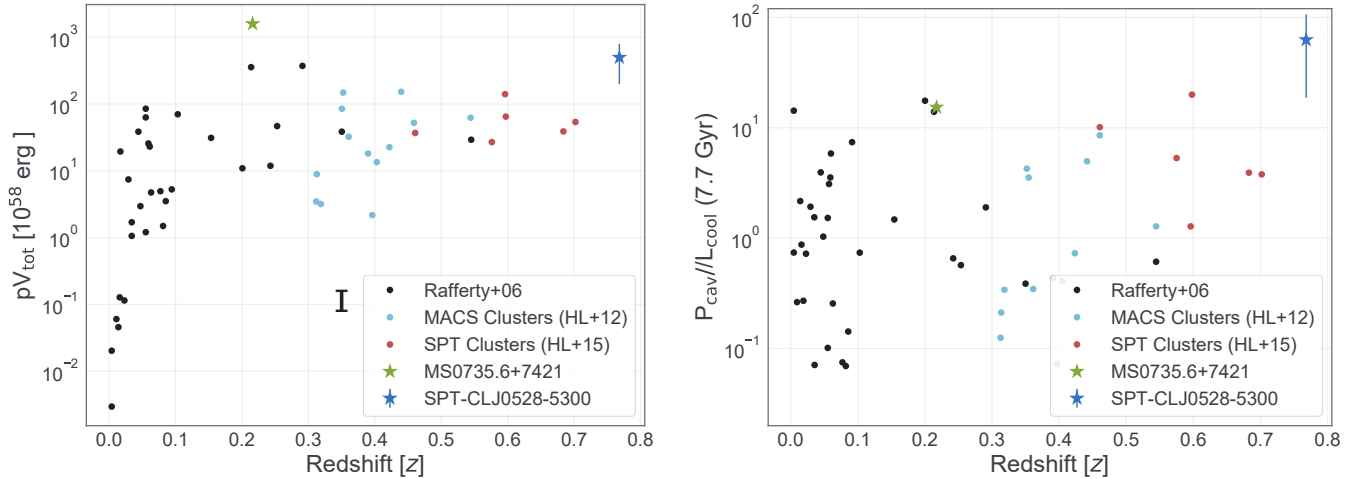
Figure 5. Left: Cavity/outburst energy, and right: ratio of cavity power ( P_{cav} ) to cooling luminosity ( L_{cool} ), as functions of redshift, adapted from Hlavacek-Larrondo et al. (2015). This demonstrates that SPT0528 is amongst the most powerful outbursts yet discovered. The discovery of similar systems at equally high redshifts could significantly influence the inferred evolution of AGN feedback.
