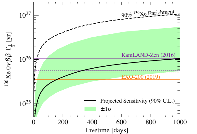
FIG. 4. LZ projected sensitivity to ^{136}\text{Xe } 0\nu\beta\beta decay as a function of detector live time. The light green shaded band represents a \pm 1\sigma statistical uncertainty on the sensitivity. The dashed black line shows the projected sensitivity to ^{136}\text{Xe } 0\nu\beta\beta decay for a dedicated run with 90% ^{136}\text{Xe} enrichment. For comparison, the limits set by EXO-200 [55] (orange full) and KamLAND-Zen [5] (purple full) are also shown, along with the respective projected sensitivities (dashed).
