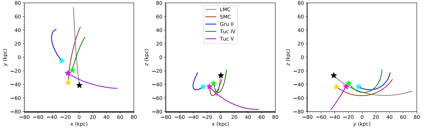
Figure 8. (left) Projections of the orbits on the X-Y plane for Gru II (blue), Tuc IV (green), and Tuc V (purple), as well as the LMC (gray) and SMC (brown). The orbits are integrated backward for 400 Myr, and the star at the end of each trajectory indicates the present position of the object. (middle) Projections of the orbits on the X-Z plane for the same dwarfs. (right) Projections of the orbits on the Y-Z plane. The very different paths by which the three ultra-faint satellites have reached the current apparent grouping are clear. The LMC and Tuc IV orbits intersect \sim 150 Myr ago in all three planes.
