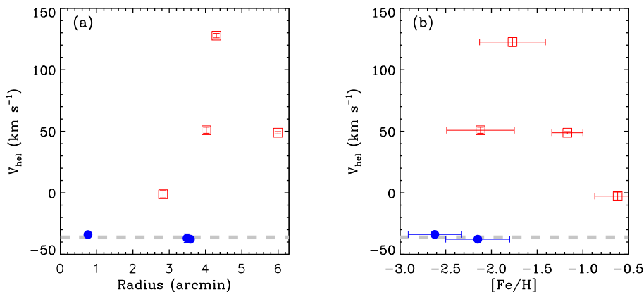
Figure 5. (left) Velocity as a function of distance away from the center of Tuc V for stars in the RGB selection region shown in Fig. 3a. The identified Tuc V members are plotted as filled blue circles, while the spectroscopic non-members are shown as open red squares. The systemic velocity of Tuc V is displayed as a dashed gray line. (right) Velocity as a function of metallicity for stars in the RGB selection region (between the two isochrones and brighter than g \approx 21.1 ) shown in Fig. 3a. Symbols are as in the left panel. The spectrum of the faintest Tuc V member does not have a high enough S/N ratio for an accurate measurement of the CaT equivalent width, so only the two brighter members are plotted in this panel. Note that because CaT metallicities depend on the assumed distance, the metallicities for the non-Tuc V stars are likely underestimated (presuming that these stars are in the foreground). The Tuc V members share a common velocity and are closer to the center and more metal-poor than the non-members.
