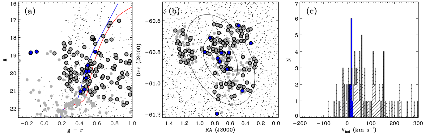
Figure 2. (a) DES color-magnitude diagram of Tucana IV. Stars within 17' of the center of Tuc IV are plotted as small black dots, and stars selected for spectroscopy (as described in §2.2) are plotted as filled gray circles. Points surrounded by black outlines represent the stars for which we obtained successful velocity measurements, and those we identify as Tuc IV members are filled in with blue. The M92 sequence and PARSEC isochrone used to define the RGB are displayed as blue and red curves, respectively. (b) Spatial distribution of the observed stars. Symbols are as in panel (a). The black ellipses represent one and two times the half-light radius of Tuc IV. (c) Radial velocity distribution of observed stars. Tuc IV members are highlighted in blue, and the hatched histogram indicates stars that are not members of Tuc IV.
