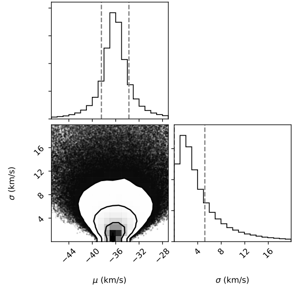
Figure 7. Corner plot for the velocity and velocity dispersion of Tuc V.
