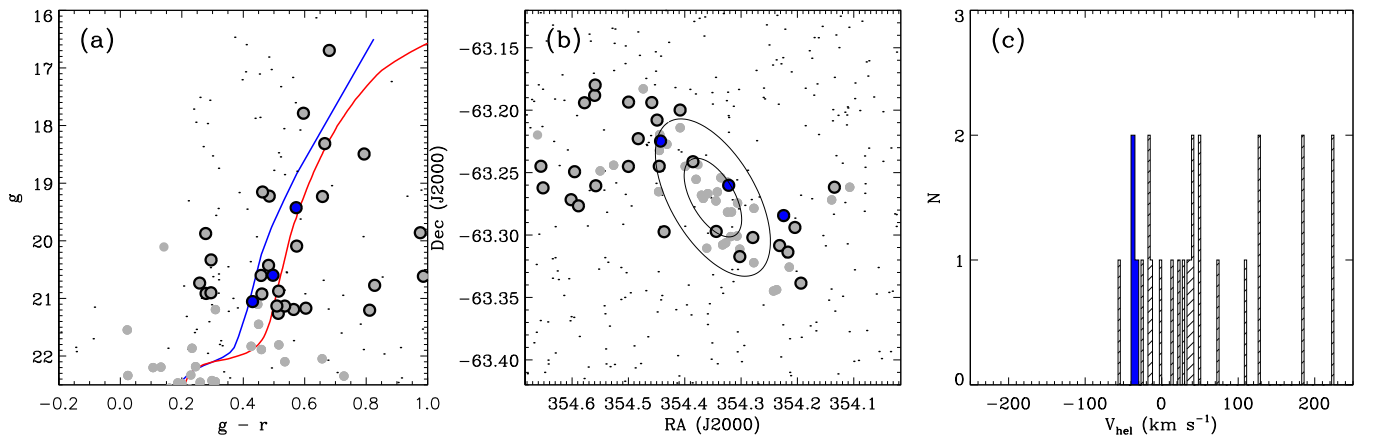
Figure 3. (a) DES color-magnitude diagram of Tucana V. Stars within 7' of the center of Tuc V are plotted as small black dots, and stars selected for spectroscopy (as described in §2.2) are plotted as filled gray circles. Points surrounded by black outlines represent the stars for which we obtained successful velocity measurements, and those we identify as Tuc V members are filled in with blue. The M92 sequence and PARSEC isochrone used to define the RGB are displayed as blue and red curves, respectively. (b) Spatial distribution of the observed stars. Symbols are as in panel (a). The black ellipses represent one and two times the half-light radius of Tuc V. (c) Radial velocity distribution of observed stars. Tuc V members are highlighted in blue, and the hatched histogram indicates stars that are not members of Tuc V.
