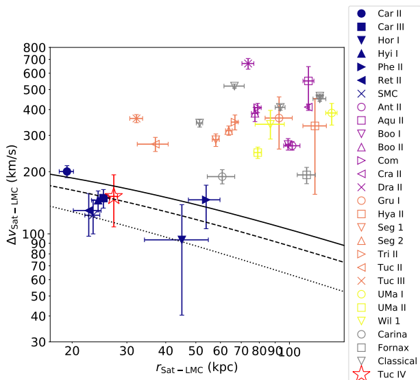
Figure 9. Distance and speed of satellites with respect to the LMC. This figure is almost identical to the one in Erkal & Belokurov (2019) except we have also included the relative distance and velocity of Tuc IV. The dotted, dashed, and solid lines show the escape velocity for an LMC with masses of 5, 10, 15 \times 10^{10} M_{\odot} and scale radii of 6.2, 12.4, 17.1 kpc, respectively. The solid blue markers show the satellites that Erkal & Belokurov (2019) identified as Magellanic satellites. Interestingly, Tuc IV sits at a similar position in phase-space.
