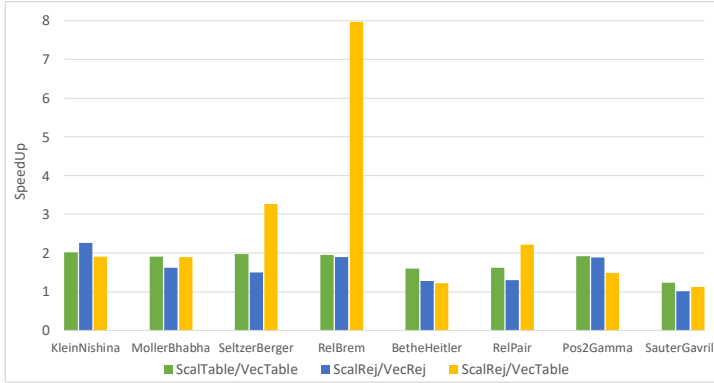
Figure 1: Speedup of the final state generation of different electromagnetic physics models obtained with SIMD vectorization in case of different sampling algorithms. The results were obtained by using Google Benchmarks [17] on an Intel® Haswell Core™ i7-6700HQ, 2.6 GHz, with Vc backend and AVX2 instruction set processing 256 tracks.
