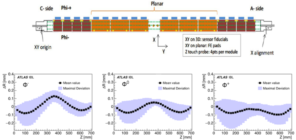
Figure 24: Summary of the planarity, R , for the 33 production bare staves in three azimuthal positions as defined in the text: (a) \Phi^- ; (b) \Phi^0 ; and (c) \Phi^+ .
