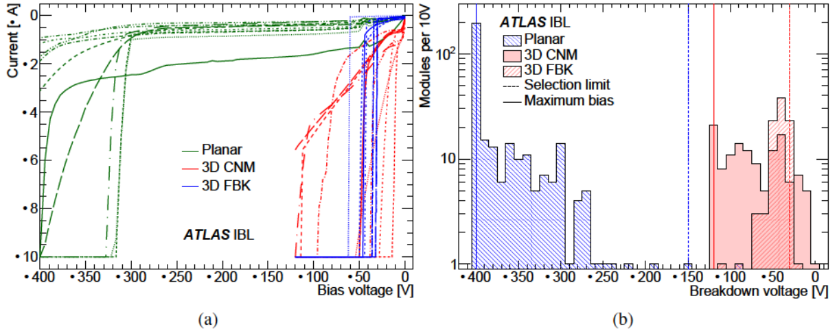
Figure 14: (a) The I-V characteristics of ten randomly chosen modules of each sensor type. The I-V curves were measured at approximately 20 °C and a current limit of -10 \mu\text{A} was used to protect the modules. The FE-I4B chips were not powered. (b) The breakdown voltage ( V_{\text{bd}} ) distributions of the tested IBL modules (313 planar, 128 3D CNM and 93 3D FBK modules). The solid vertical lines indicate the maximum measurement point of -400 \text{ V} for the planar modules and -120 \text{ V} for the 3D CNM and FBK modules. The V_{\text{bd}} acceptance criteria of below -150 \text{ V} (blue) for the planar modules and below -30 \text{ V} (red) for 3D modules are also indicated as dashed lines.
