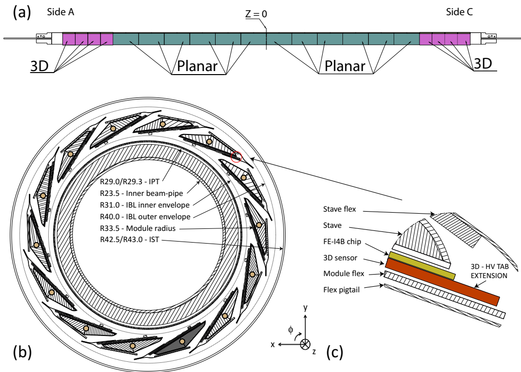
Figure 3: IBL detector layout: (a) Longitudinal layout of planar and 3D modules on a stave. (b) An r section showing the beam pipe, the inner positioning tube (IPT), the staves of the IBL detector and the inner support tube (IST), as viewed from the C-side. (c) An expanded r view of the corner of a 3D module fixed to the stave.
