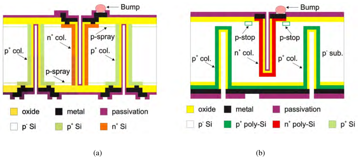
Figure 9: Design of the columns of (a) FBK and (b) CNM 3D sensors. This sketch is for illustration only and is not to scale.
