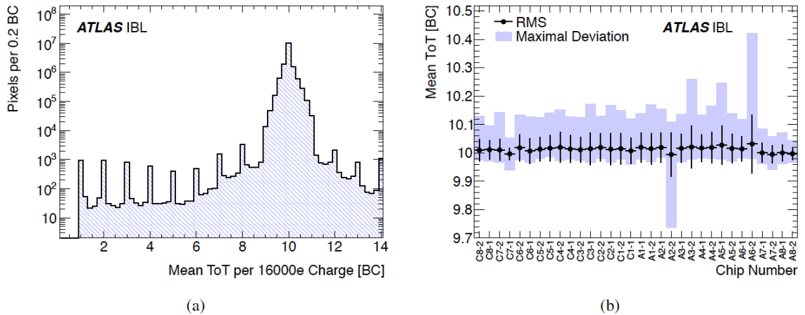
Figure 37: (a) One-dimensional Time-over-Threshold (ToT) distribution for all pixels when tuned to 10 ToT, using an injected charge of 16\,000\text{ e}^- . The spikes result from injection failures where the selected ToT value is not 10. Non-integer mean ToT values result when successive injections to evaluate the mean select differing ToT values. (b) The average ToT distribution as a function of the chip number (position) on the stave. The data are from all 18 qualified staves using a mean module threshold of 1500\text{ e}^- at -12\text{ C} .
