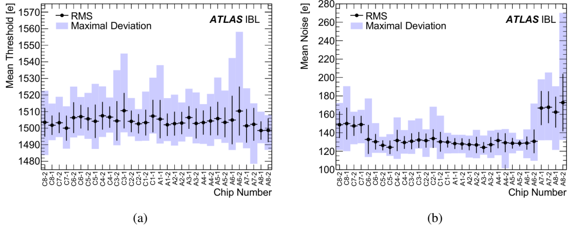
Figure 40: (a) Mean threshold and (b) mean noise (ENC) distributions for all 18 qualified staves as a function of the chip number (position) on the stove, for a 1500 e - threshold tuning at -12 C. The error bars represent the RMS value accounting for the differences between staves whereas the solid colour describes the full range covered by data.
