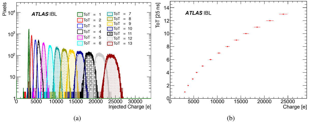
Figure 17: Calibration function of the Time-over-Threshold (ToT) to charge: (a) for a given ToT value, the mean injected charge of each pixel, and (b) the charge-to-ToT calibration function. Measurements of the charge distributions for ToT = 14 were biased by the maximum injected charge and were excluded from the calibration.
