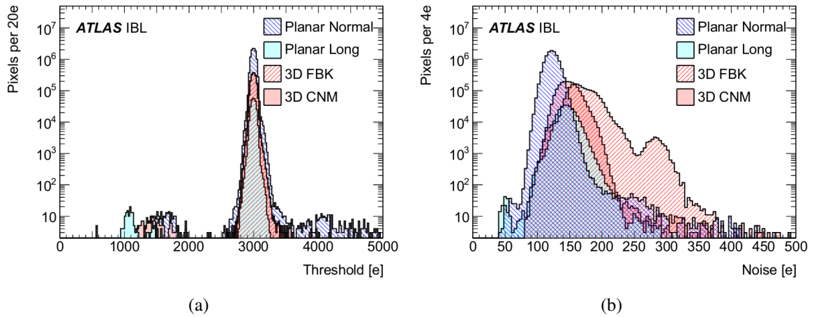
Figure 38: (a) Threshold and (b) noise (ENC) distributions of individual pixels for a 3000 e^- threshold tuning at 22 C. The threshold width is primarily determined by the injection circuit, and only a few individual pixels were badly tuned.
