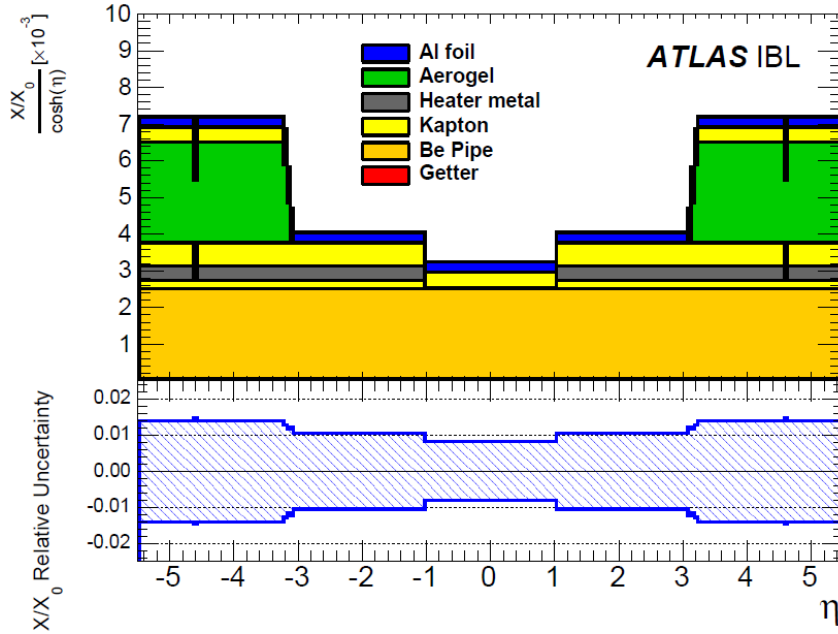
Figure 53: The calculated radiation length X/X_0 of the new beam pipe normalised by \cosh^{-1} as a function of \eta . The lower plot shows its relative uncertainty. The Getter (NEG) contribution is small and is not visible.
